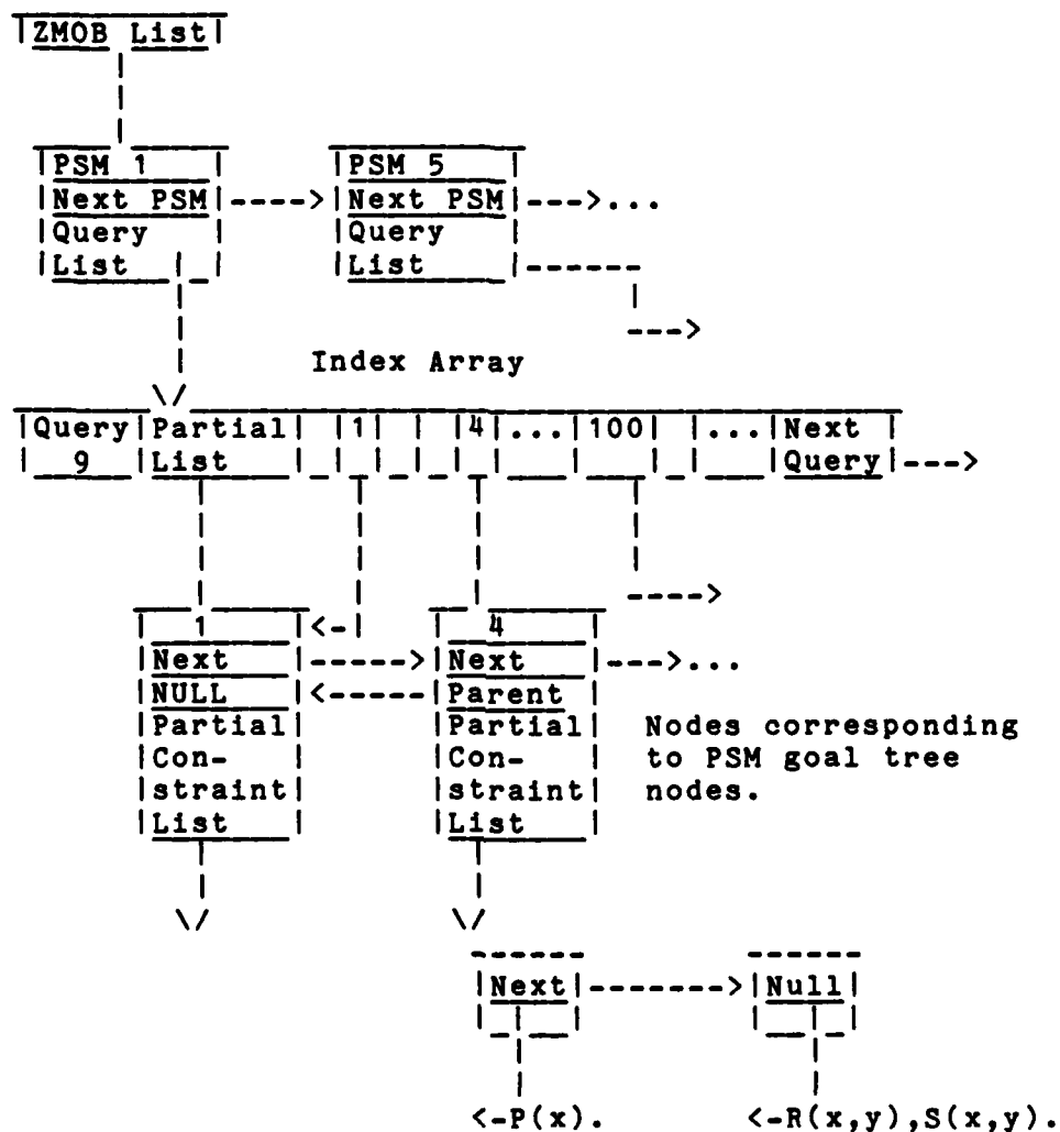
Fig. 2. Structure of the partial constraint tree.
