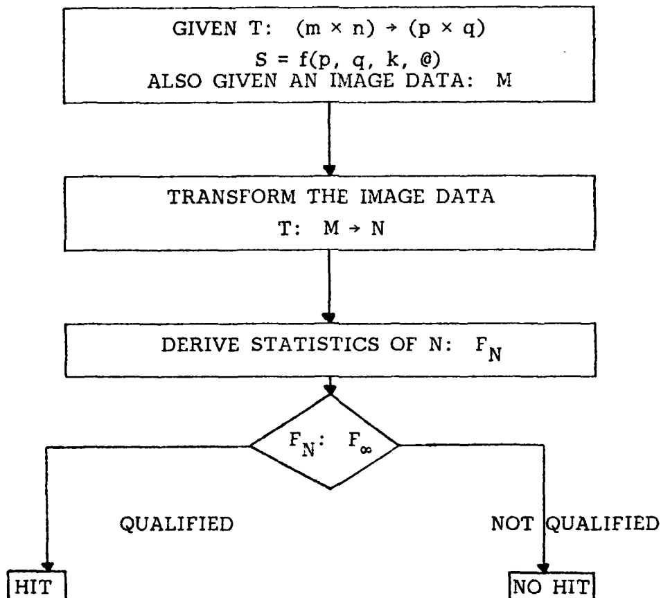
Fig. 5. Object detection scheme.
