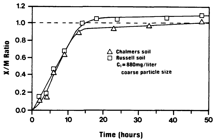
Figure 12. Adsorption Equilibration for Coarse Particle Soil with TCE Concentration of 880 mg/l.
