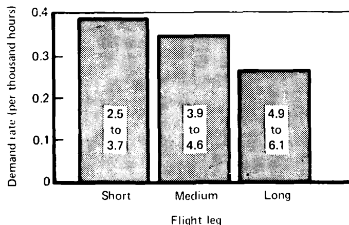
Fig. 5 - Commercial engine removal experience
