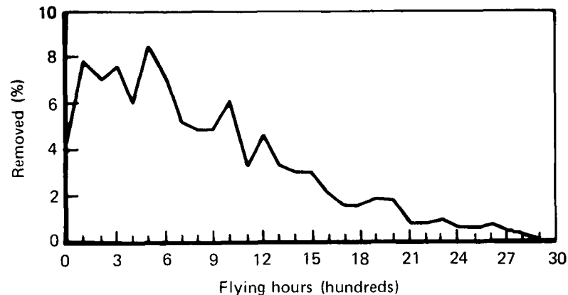
Fig. 13 — Percentage of engines removed by age interval
