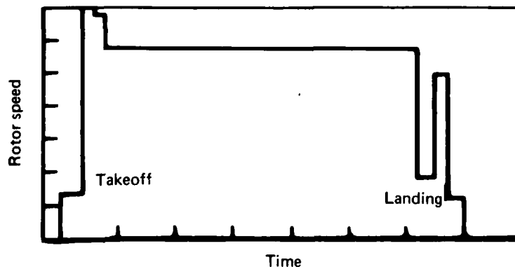
Fig. 3 - Typical mission sortie profile
