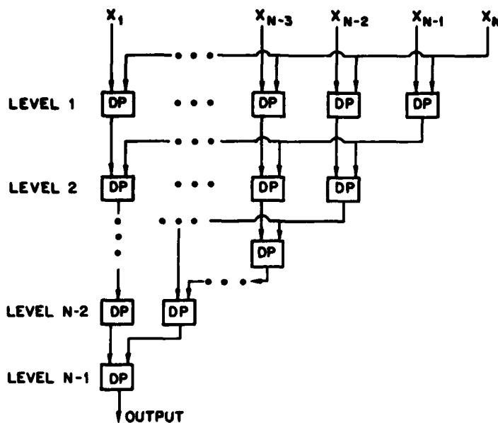
Fig. 2 - N -channel decorrelator
