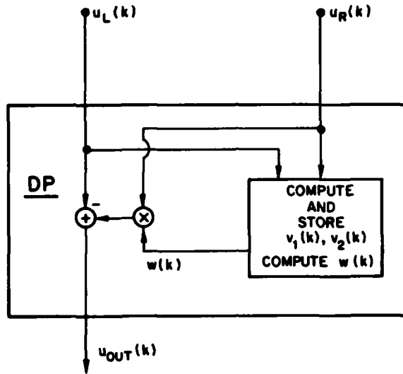
Fig. 7 - Recursive two-input decorrelator processor (DP)
