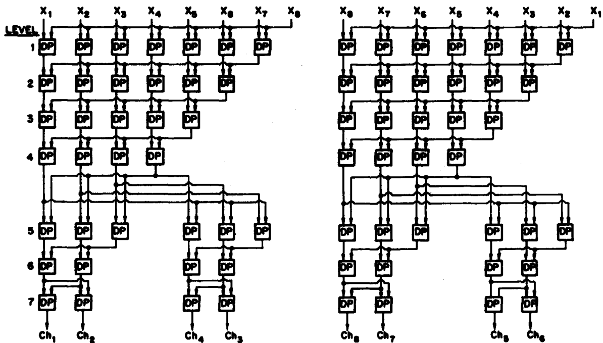
Fig. 6 - Complete realization of an eight-channel Fast Orthogonalization Network
