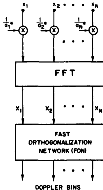
Fig. 10 — Adaptive doppler processor using a lattice filter
