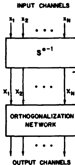
Fig. 3 - Multiple-channel adaptive lattice filter
