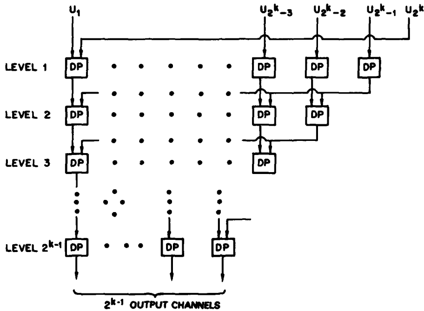
Fig. 9 - Partial orthogonalization, 2^k input channels to 2^{k-1} output channels
