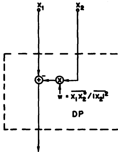
Fig. 1 - Decorrelation processor (DP)
