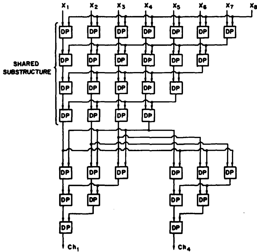
Fig. 5 - Example of substructure sharing
