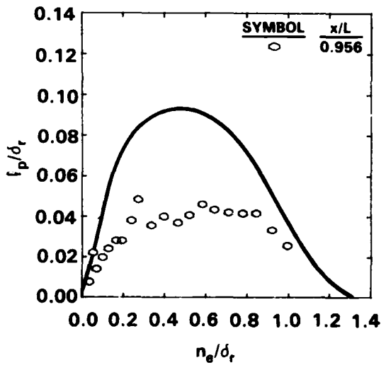
Figure 10c - 77 Degree
