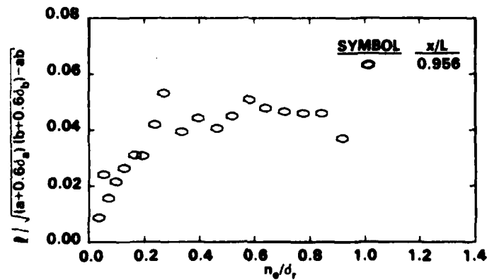
Figure 11c - 77 Degree
