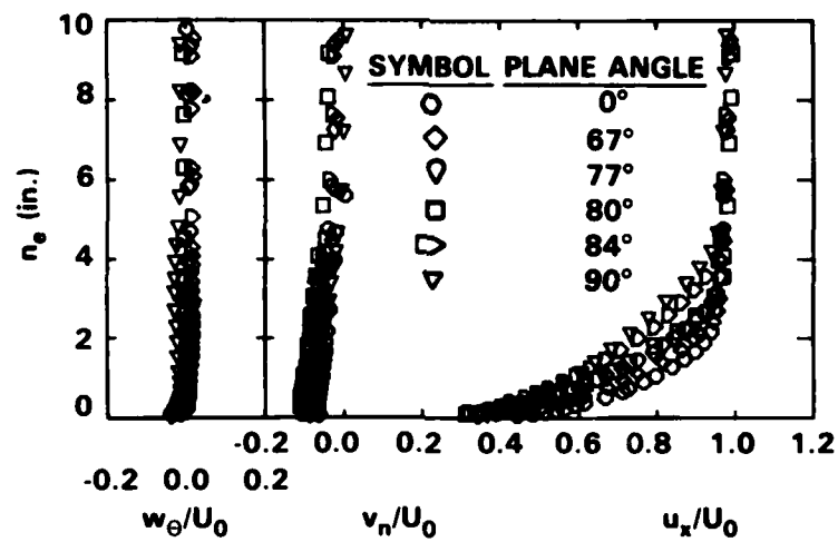
Figure 7j - x/L = 0.956
