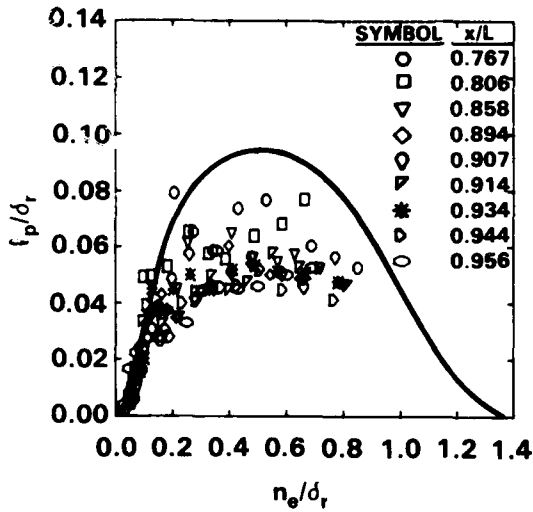
Figure 10a - 0 Degree
