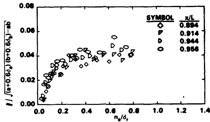
Figure 11b - 67 Degree
