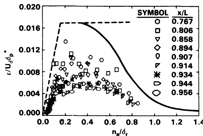
Figure 9a - 0 Degree
