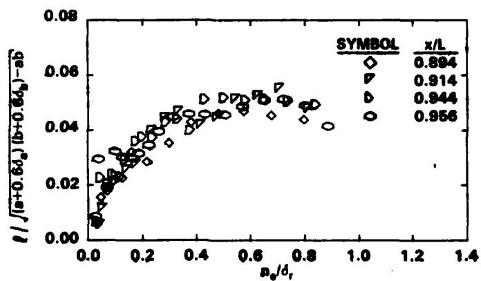
Figure 11e - 84 Degree
