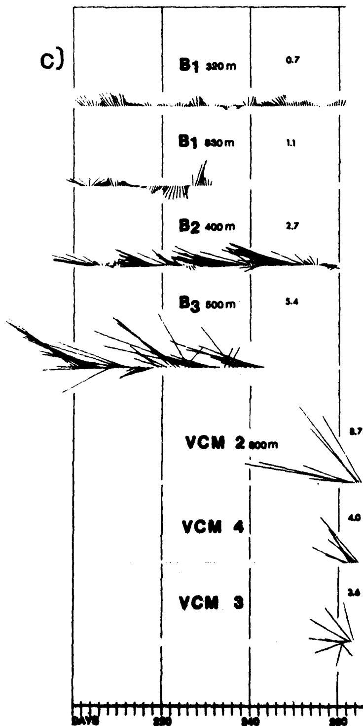
FIG. 14 (cont) c) Velocity vector time series of all currentmeters. Numbers at right signify the average speed of plotted data. Sampling interval is 12 hours for B 1 and B 2 and 24 hours for B 3 .
