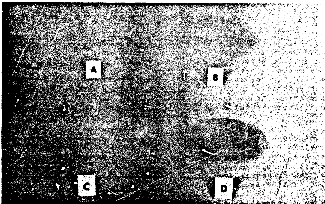
FIGURE 9. Present Earcup Pre- and Post-Impact (A and B) Experimental Earcup Pre- and Post-Impact (C and D)
