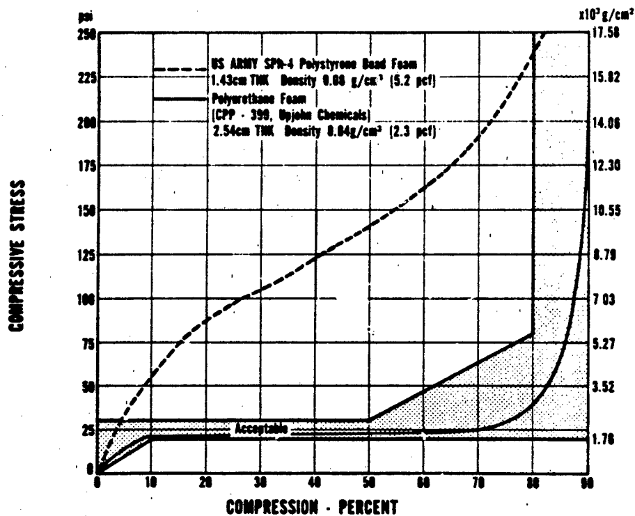
FIGURE 11. Compressive Stress-Strain Curve of Present and Experimental Foam.
