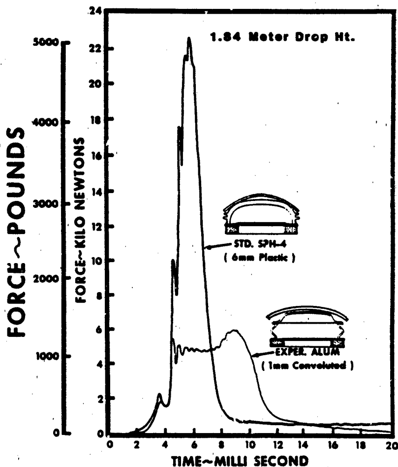
FIGURE 10. Force-Time Trace of 9.68 kg-m Drop Onto Standard and Experimental Earcup.
