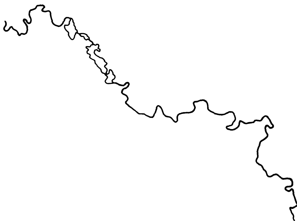
Fig. 3. An electron micrograph of the heteroduplex formed between the DNA of wild-type z and zmmP22 hybrid 1 is shown in the top portion of the figure. Below is a line drawing of the heteroduplex molecule. Homologous regions are indicated by a thick line and unhybridized single-stranded regions are indicated by thin lines. The bar in the electron micrograph represents 1.0 \mu m.
