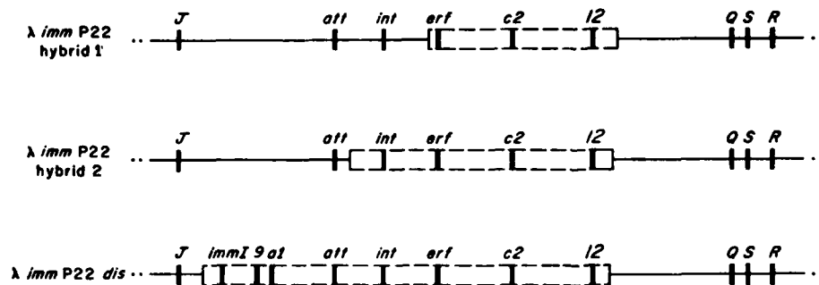
Fig. 2. Portions of the \lambda and P22 genome in the \lambda immP22 hybrids are shown at the top of the figure. Genetic characteristics of the \lambda and the P22 genome are positioned so that similar functions in both phages are aligned as described by Botstein, Chan and Waddell (1972). The P22 genes shown in the hybrids have been determined by genetic analysis to be present. The extent of the P22 segment in the hybrids is enclosed by dashed lines to indicate that the exact extent of the P22 segments in these hybrids has not been established by genetic means.
