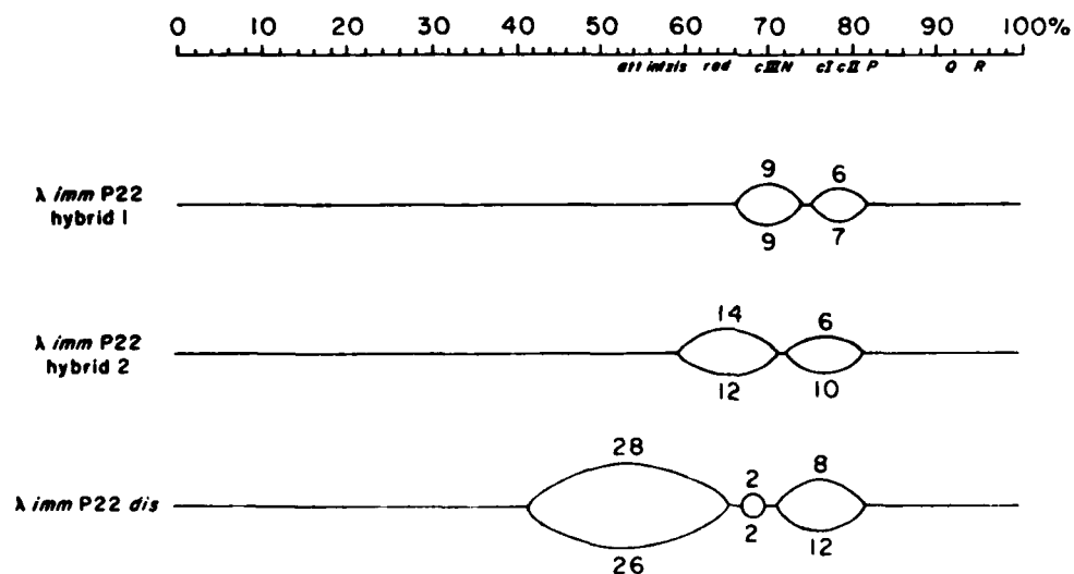
Fig. 5. The results of heteroduplex analysis of the zim P22 hybrids are summarized diagrammatically. The regions of homology between wild-type \lambda and the zim P22 hybrids are indicated by a single line. Nonhomologous portions of the molecule are indicated by loops. These loops correspond to single-stranded non homologous regions of the DNA heteroduplex molecules. The combined results from at least ten molecules of each heteroduplex type were used to establish the duplex regions in the representations of the molecules.
