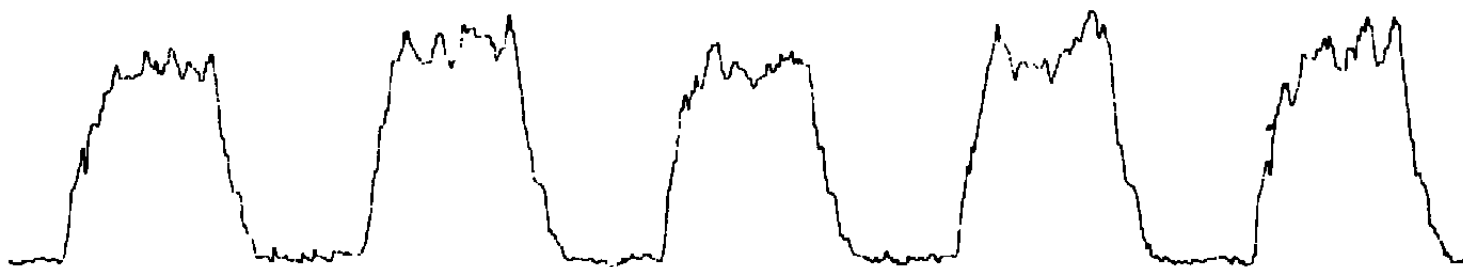
b. Response of the Capacitive Transducer (B&K Type 4136) Average Rise Time = 0.7 ms
