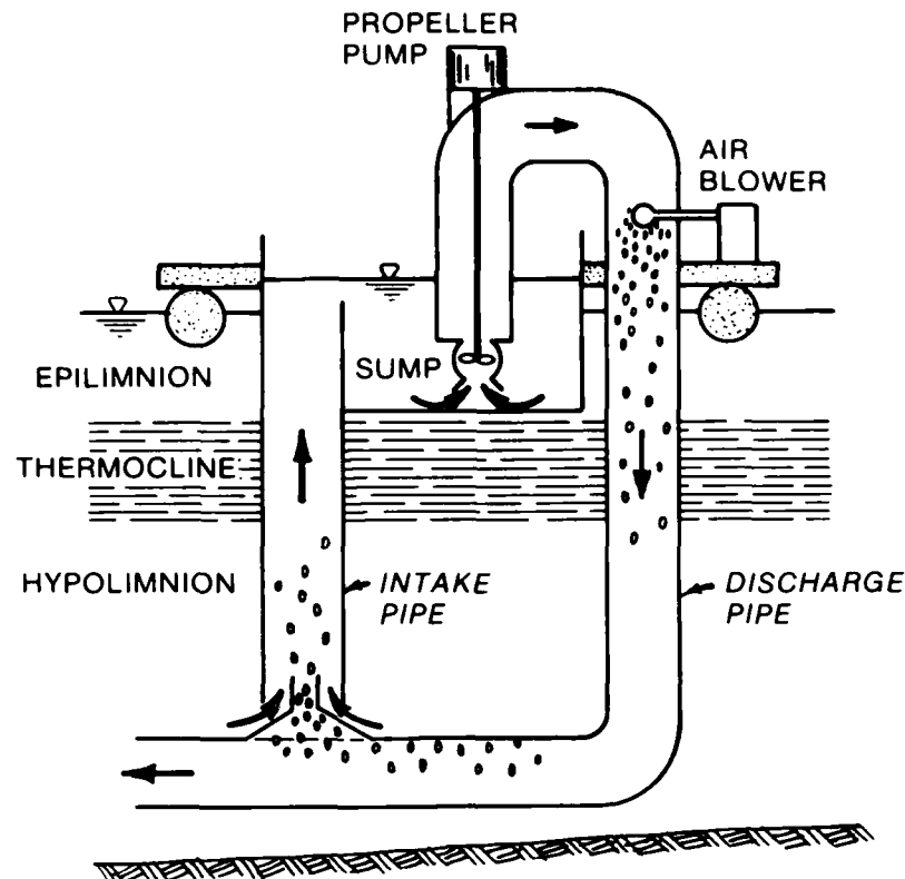
Figure A10. A proposed downflow air injection system which also incorporates the air lift feature
