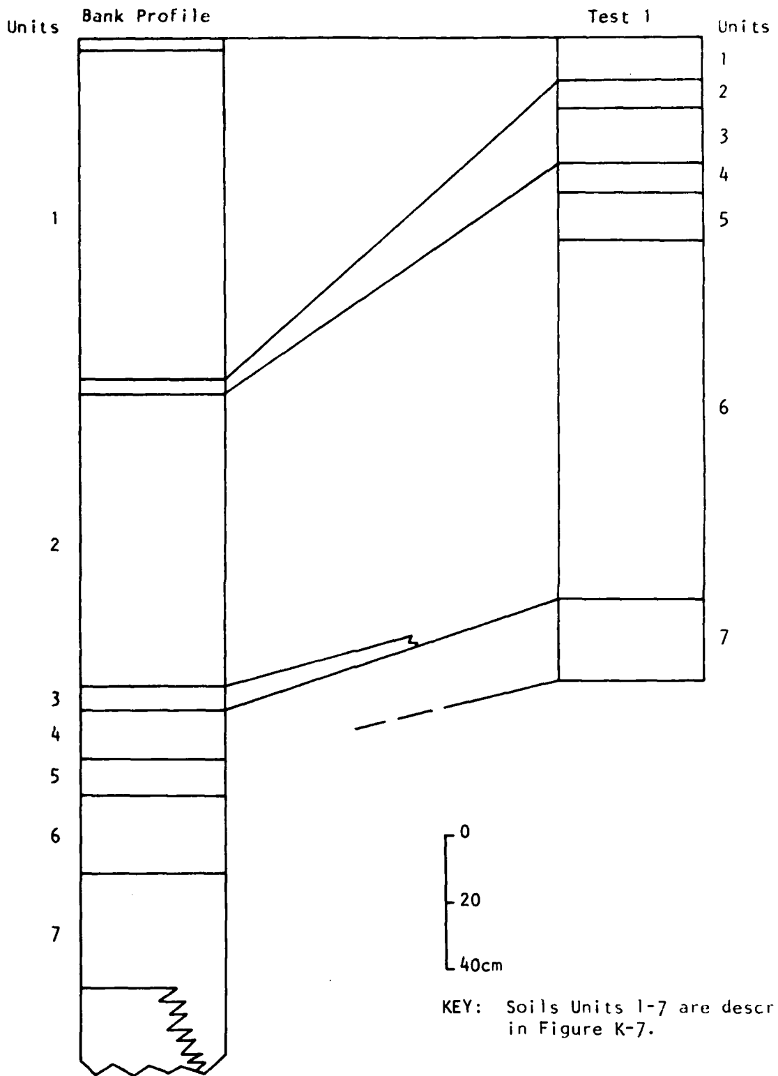
Figure K-8. Correlation of the Test 1 and bank profiles showing the correspondence of recognized units.
