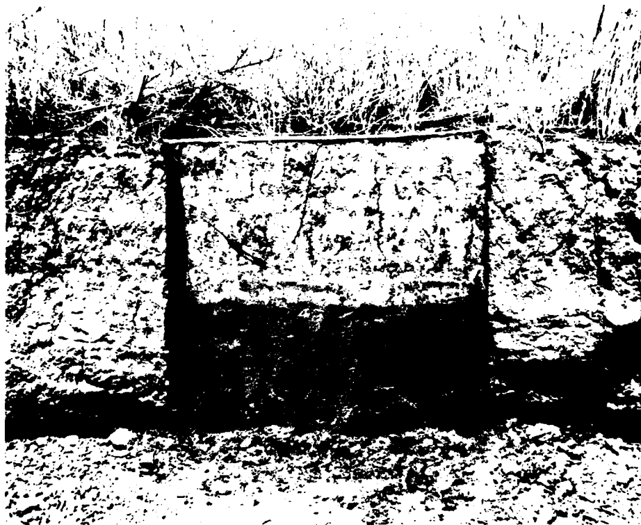
Figure K-10. A) Photographic view east toward the embayment of Lake Sharpe in an old stream valley heading on the lower slopes of MT-3 and cutting into MT-2. The site is in the center lower portion of the photograph and the bank profile near the accumulation of logs. B) Bank profile at wave cut bench in the embayment. The lower dark portion is typical of wetted loess.
