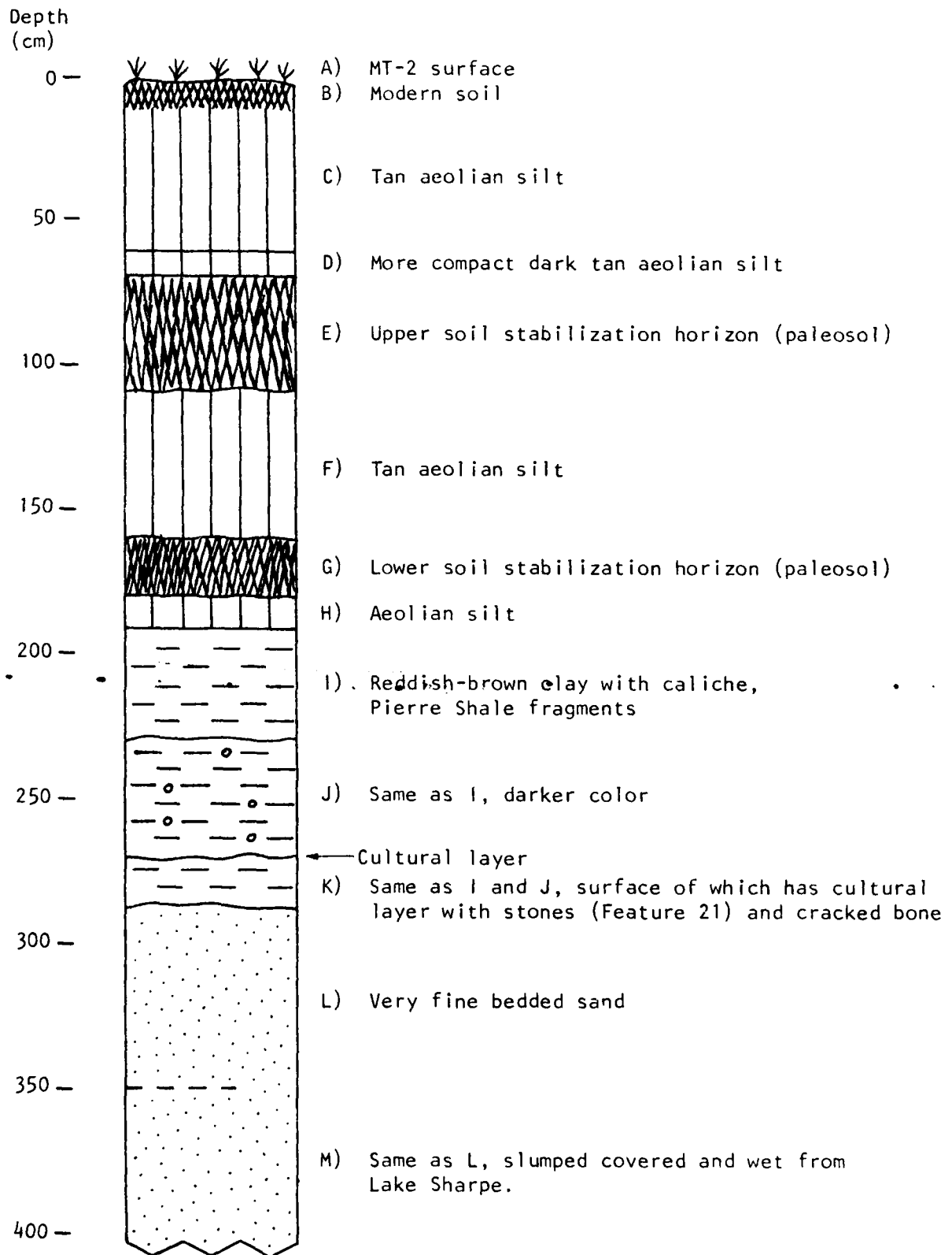
Figure K-41. The bank profile at the site.
