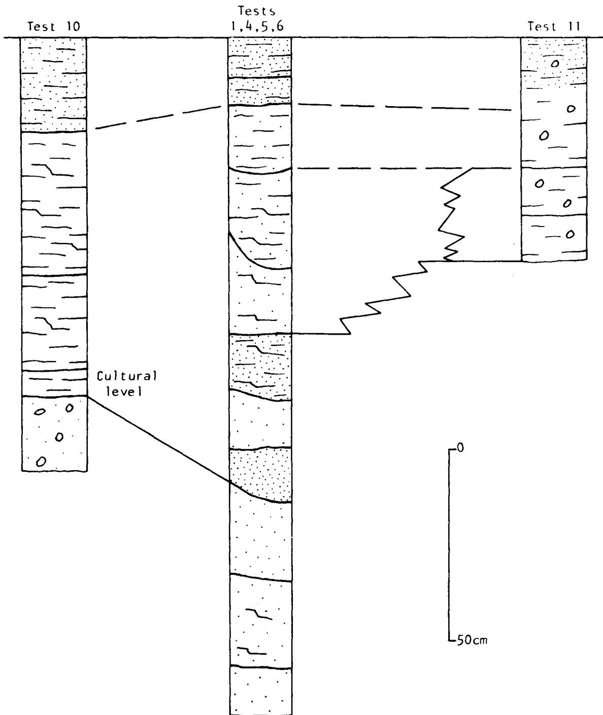
Figure K-26. Detailed correlation cross section of Tests 10, 1 and 11 using the present ground surface as the datum without regard to elevation. Test 2 is not shown because it cannot be correlated across the section. A change in lithology between Test 11 and 1 is shown indicating the change from mainly slope wash in Test 11 to mixed materials in Test 1. The level of the cultural layer in Test 1 (Unit 7 of Figure K-20) is shown as correlated to the cultural level in Test 10.
