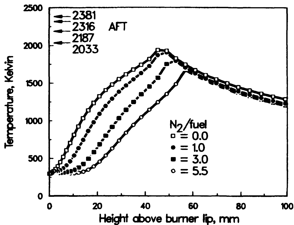
FIGURE 11 Calculated axial temperature profiles in ethylene-air diffusion flames, showing effect of nitrogen dilution. Ethylene flowrate \dot{V}_f = 3.4 std. \text{cm}^3/\text{sec} .
