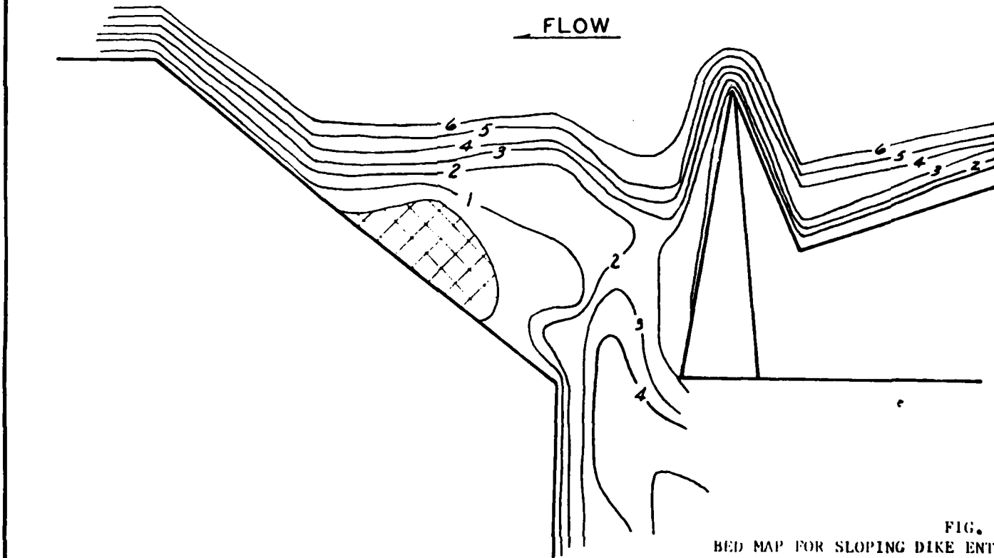
FIG. 1 BED MAP FOR SLOPING DIKE ENTRANCE FLOOD STAGE. RUN TIME = 25.
