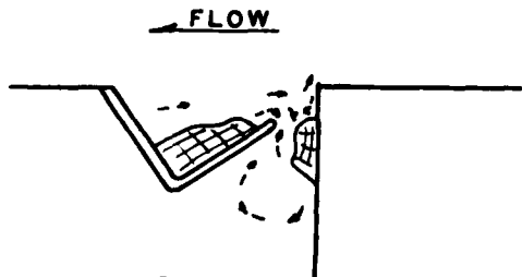
FIG 8 DIMENSIONS 2.0-2.0-1.0, FLOOD STAGE, 'L' STRUCTURE TOO CLOSE TO UPSTREAM WALL SEDIMENT DEPOSITED INTO BASIN WHERE IT DE- POSITED BLOCKED THE ENTRANCE
