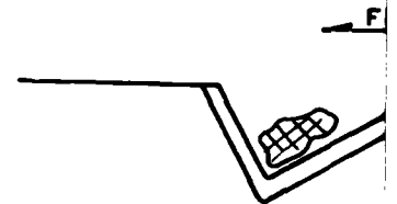
FIG 6 RUN 14D; DIMENSIONS 1.0-1.5-1.0; FLATTENED "L" ANGLE, FLOW DEFLECTS SEDIMENT TO TURN FLOW BUT LARGE DEPOSIT FORMS BEHIND BAFFLE
