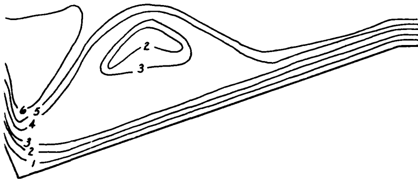
FIG 1 MAP FOR SLOPING DIKE ENTRANCE FLOWING RUN 34 BETWEEN FLOOD AND NORMAL STAGE. RUN TIME = 77.7 HOURS
