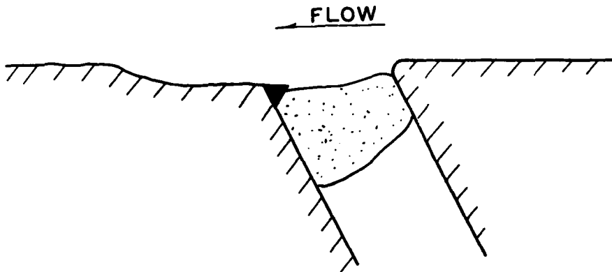
FIG. 5 SERIES 19, ANGLED ENTRANCE WITH BAFFLE DOWNSTREAM, FLOOD STAGE. FAIRLY UNIFORM DEPOSIT APPROXIMATELY 0.5 FOOT DEEP ACROSS ENTRANCE, PERFORMED BETTER THAN OTHER TRIALS
