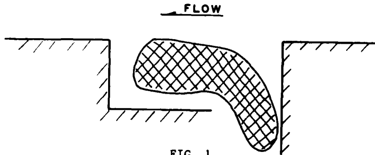
FIG 1 *RUN 11A, DIMENSIONS 1.0-1.5-1.0; LARGE BAR DEVELOPED IN ENTRANCE
