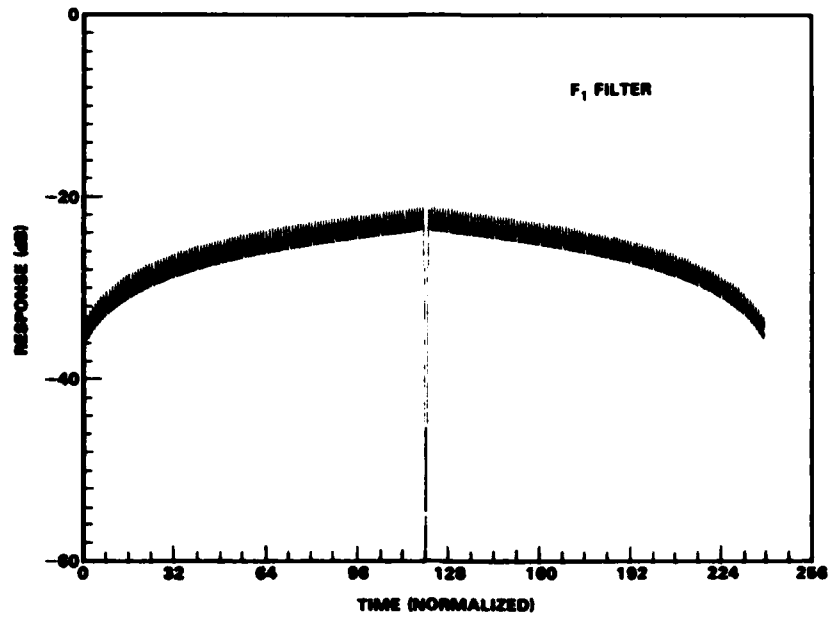
Fig. 3 — F_1 doppler-filter response for a random binary-phase code with the code element N = 127
