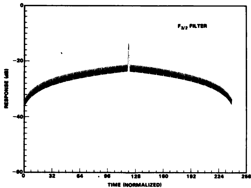
Fig. 4 — F_{3/2} doppler-filter response for a random binary-phase code with the code element N = 127
