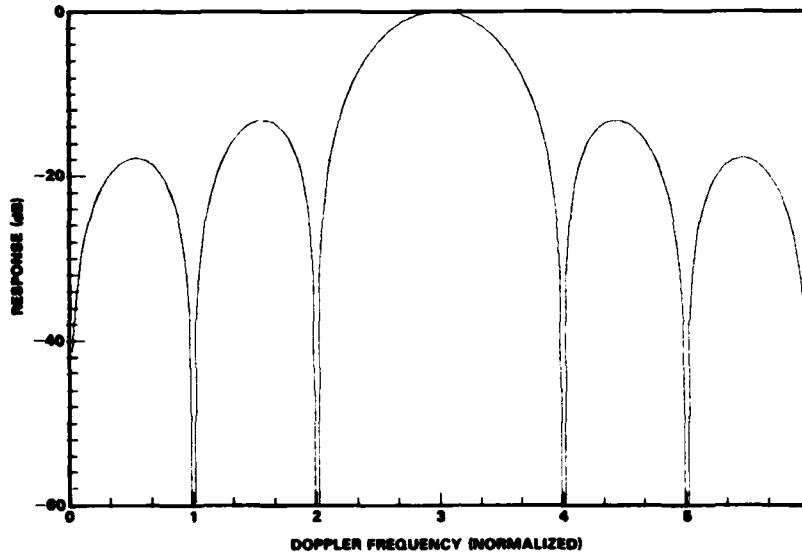
Fig. 7 — Ambiguity function frequency response for a random binary-phase code with the code element N = 4800
