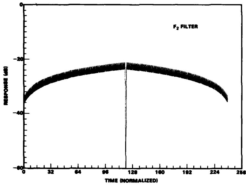
Fig. 5 — F_2 doppler-filter response for a random binary-phase code with the code element N = 127
