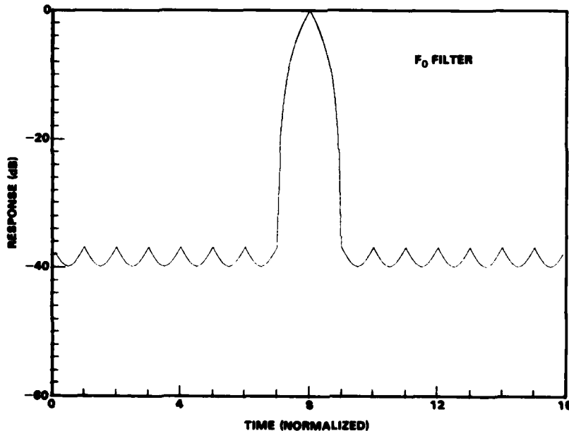
Fig. 6 — F_0 doppler-filter response for a random binary-phase code with the code element N = 4800
