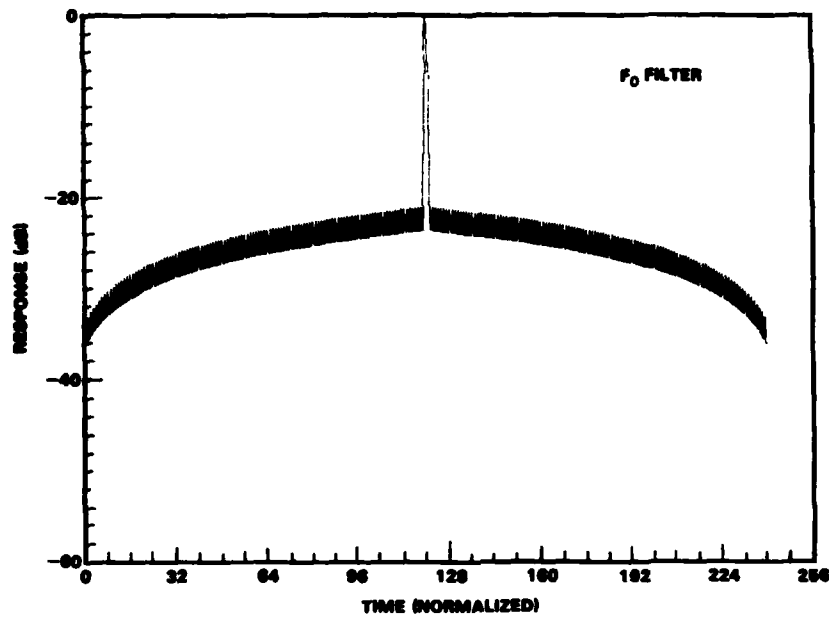
Fig. 1 — F_0 doppler-filter response for a random binary-phase code with the code element N = 127
