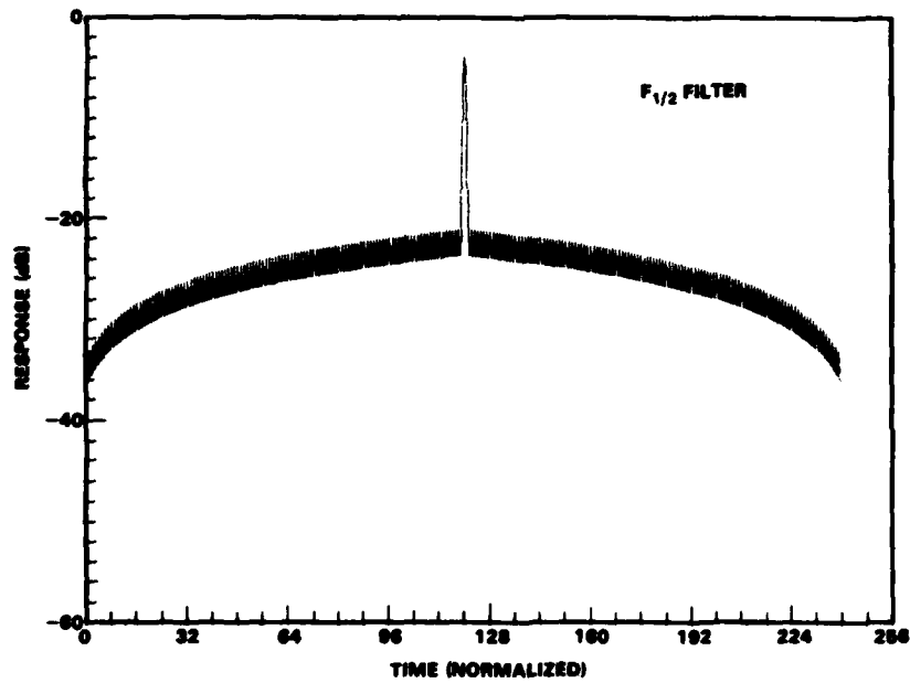
Fig. 2 — F_{1/2} doppler-filter response for a random binary-phase code with the code element N = 127
