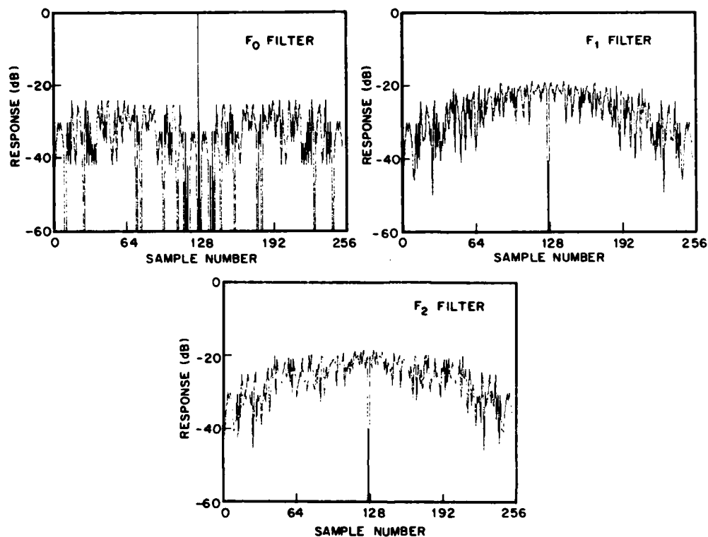
Fig. 8 — Responses of the doppler filters with a zero doppler target for a 127-element maximum-length pseudorandom binary code
