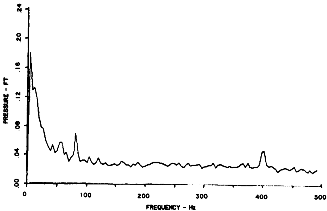
b. FFT plot
