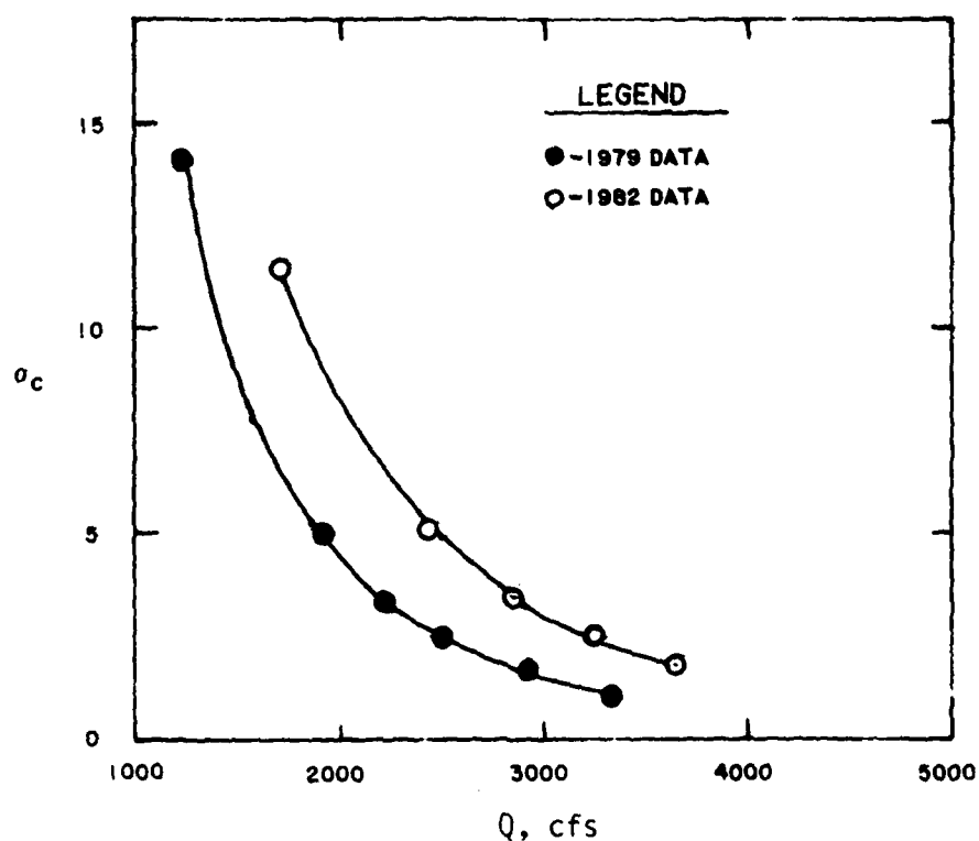
Figure 2. Cavitation index (1979 and 1982 data)
