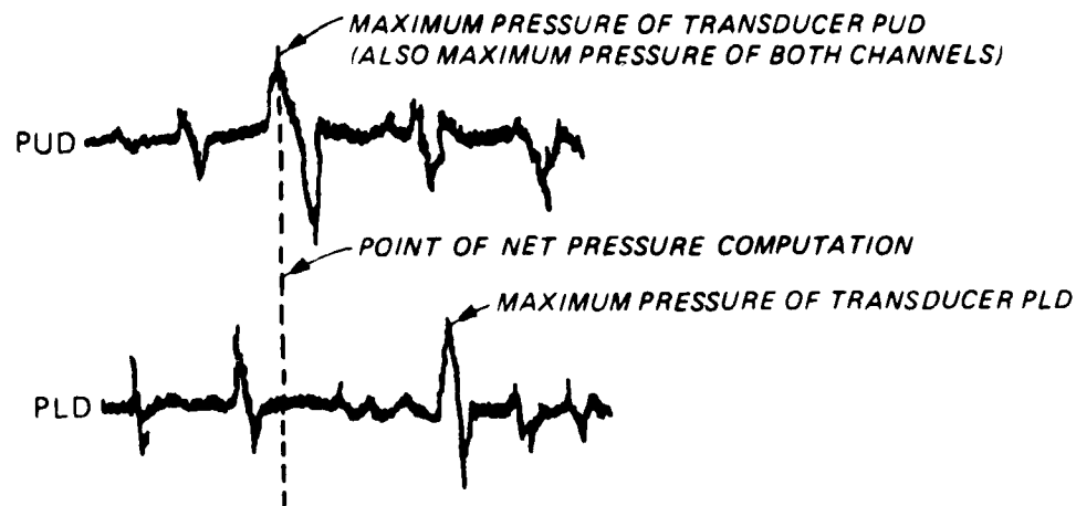
Figure 5. Determination of net pressures
