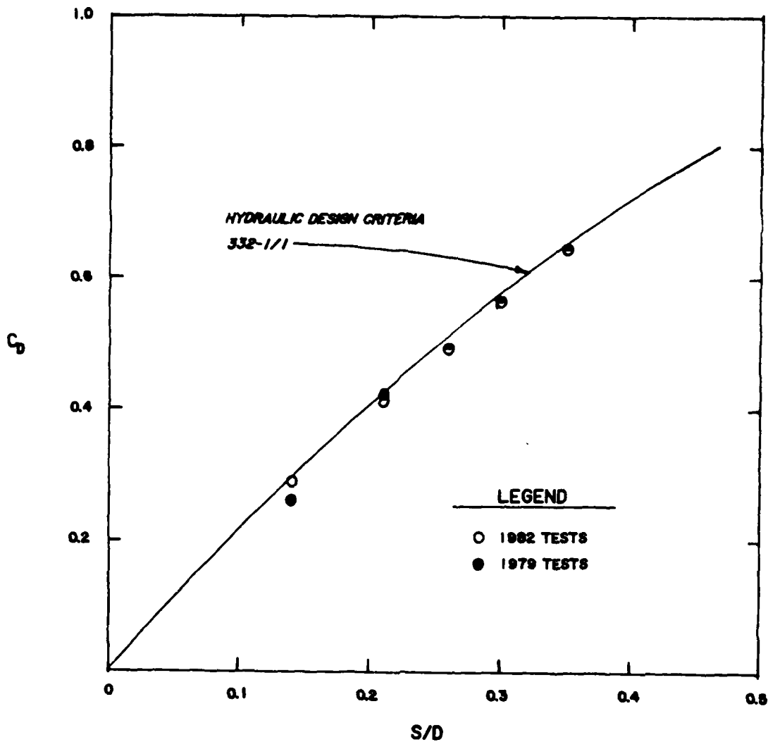
Figure 1. FC&I valve discharge coefficients
