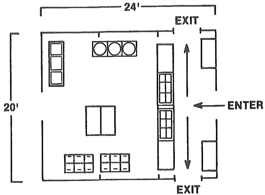
Figure 7. Large Modular Field Kitchen (451 to 1,100 troops) for T Rations
