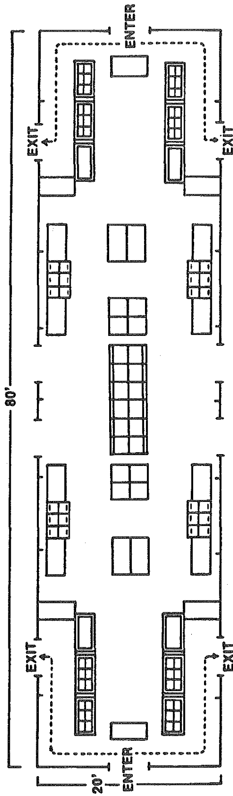
Figure 6. Complex of two Large Modular Field Kitchens (1,551 to 2,200 troops) for A, B, or T Rations.
