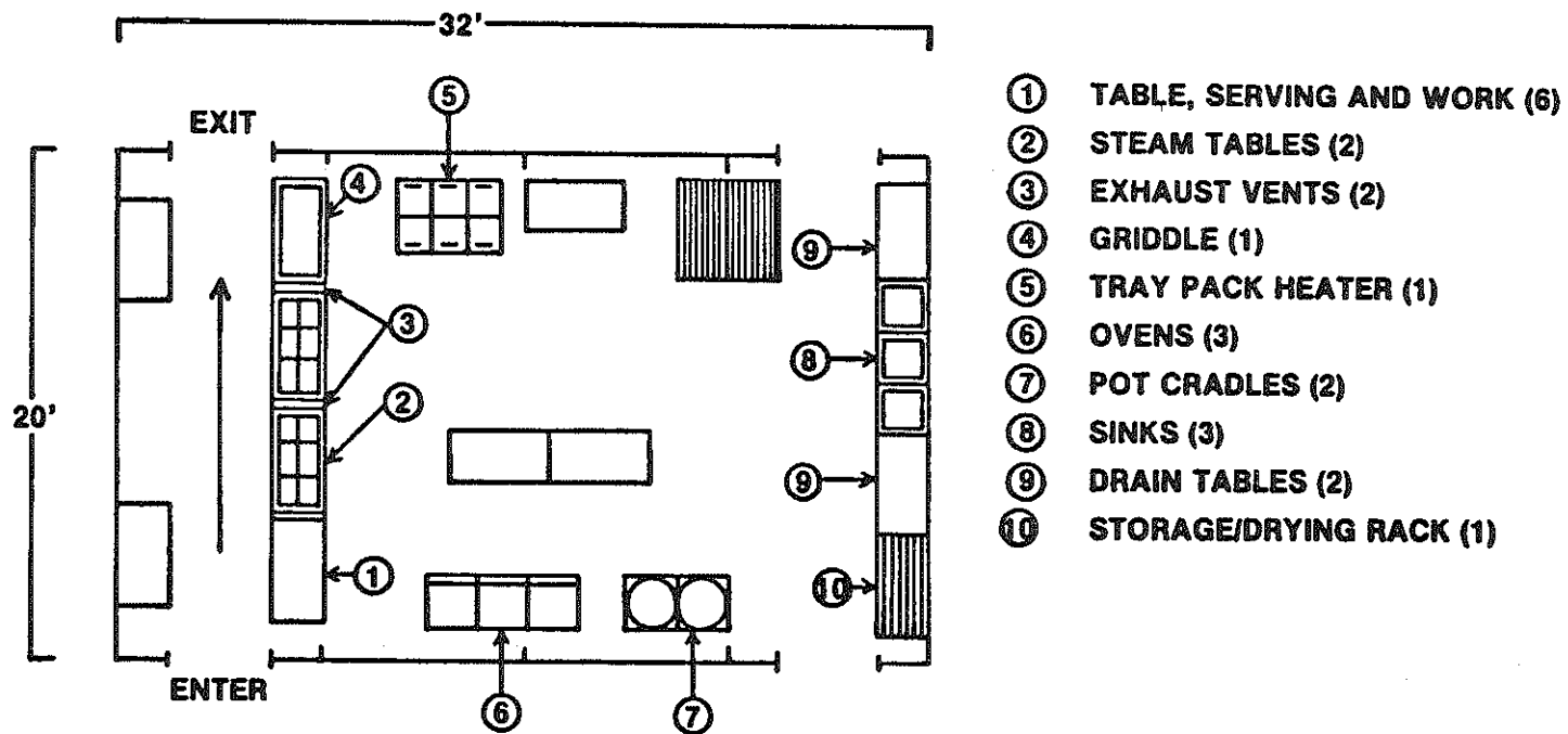
Figure 3. Medium Modular Field Kitchen (261 to 450 troops) for A, B, or T Rations.
