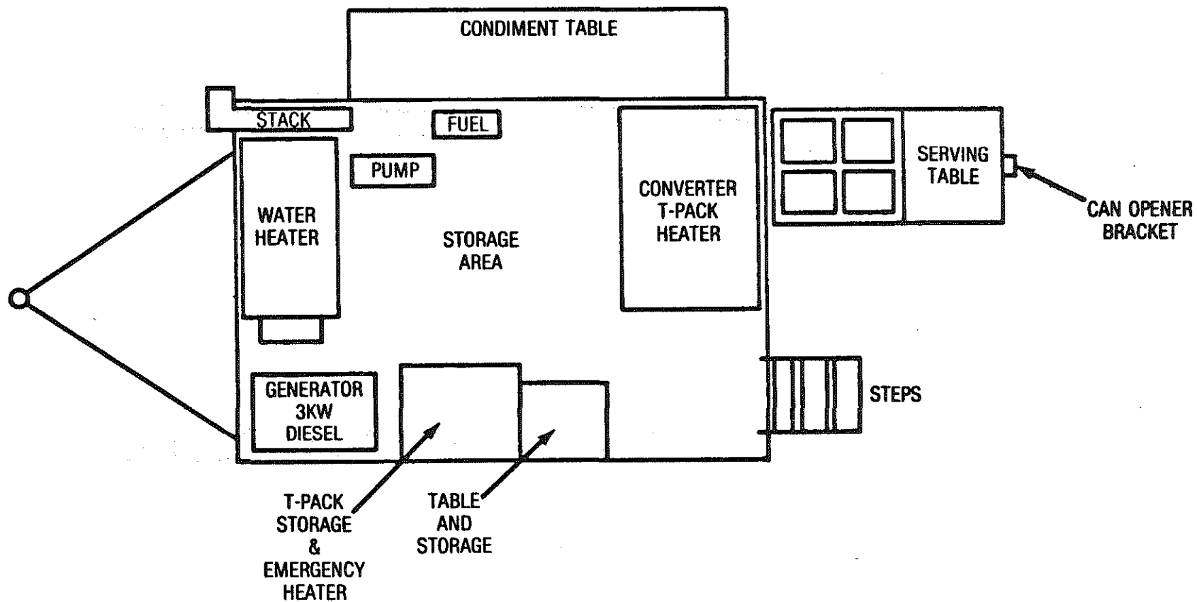
Figure 2. Typical Mobile Food Service Unit layout (T Rations).
