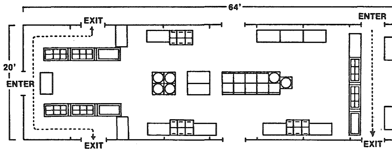
Figure 5. Complex of one Large and one Medium Modular Field Kitchen (1,361 to 1,550 troops) for A, B, or T Rations.
