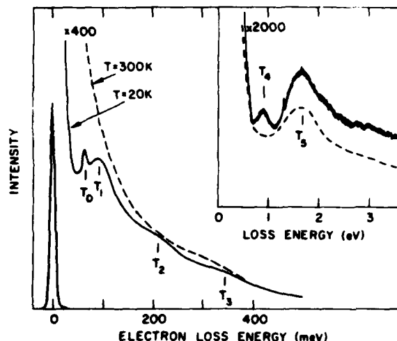
FIG. 2. Electron-energy-loss spectra for E_0 = 15 eV at T = 300 K (dashed lines) and T = 20 K (solid lines). In the inset the resolution has been degraded to 20 meV (FWHM).
