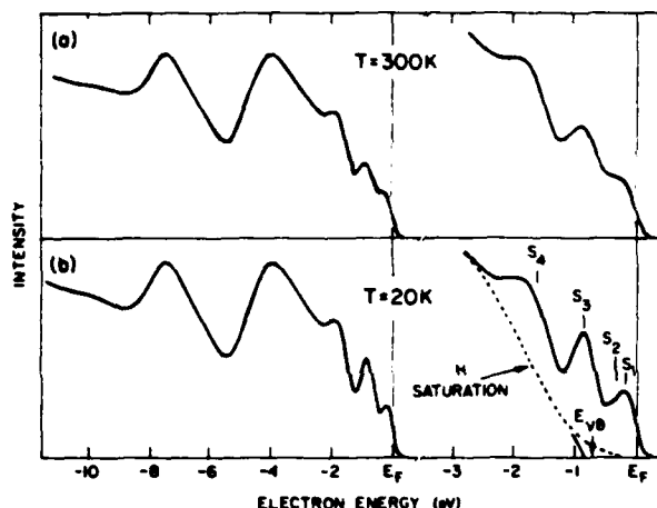
FIG. 1. Ultraviolet photoemission spectra ( h\nu = 21.2 eV) for Si(111)- 7 \times 7 at (a) 300 K and (b) 20 K under identical conditions. The right panels show an expanded view of the surface states near the top of the valence band.
