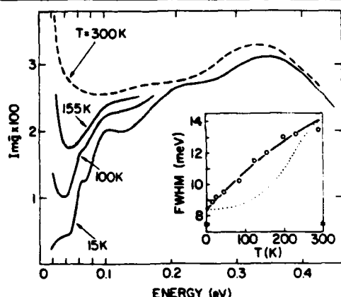
FIG. 3. The surface loss function, \text{Im}\bar{\epsilon}(E) , at several temperatures as derived from data with E_0 = 12 eV, \theta_i = \theta_f = 45^\circ , a measured angular acceptance of 2^\circ , and a total instrumental resolution of 8.5 meV (FWHM). For T = 15 K, the integral of \text{Im}\bar{\epsilon} up to \sim 0.5 eV has an oscillator strength corresponding to 4–5 electrons per 7 \times 7 unit cell (Ref. 13) while the “foot” below 40 meV may reflect band tailing or other phonons which we have neglected in our analysis. The inset shows the temperature-dependent variation of the elastic beam (circles) and two possible processes for beam broadening. The solid line corresponds to a constant free-carrier concentration while the dotted line corresponds to thermally activated free carriers associated with a 40-meV surface-state gap.
