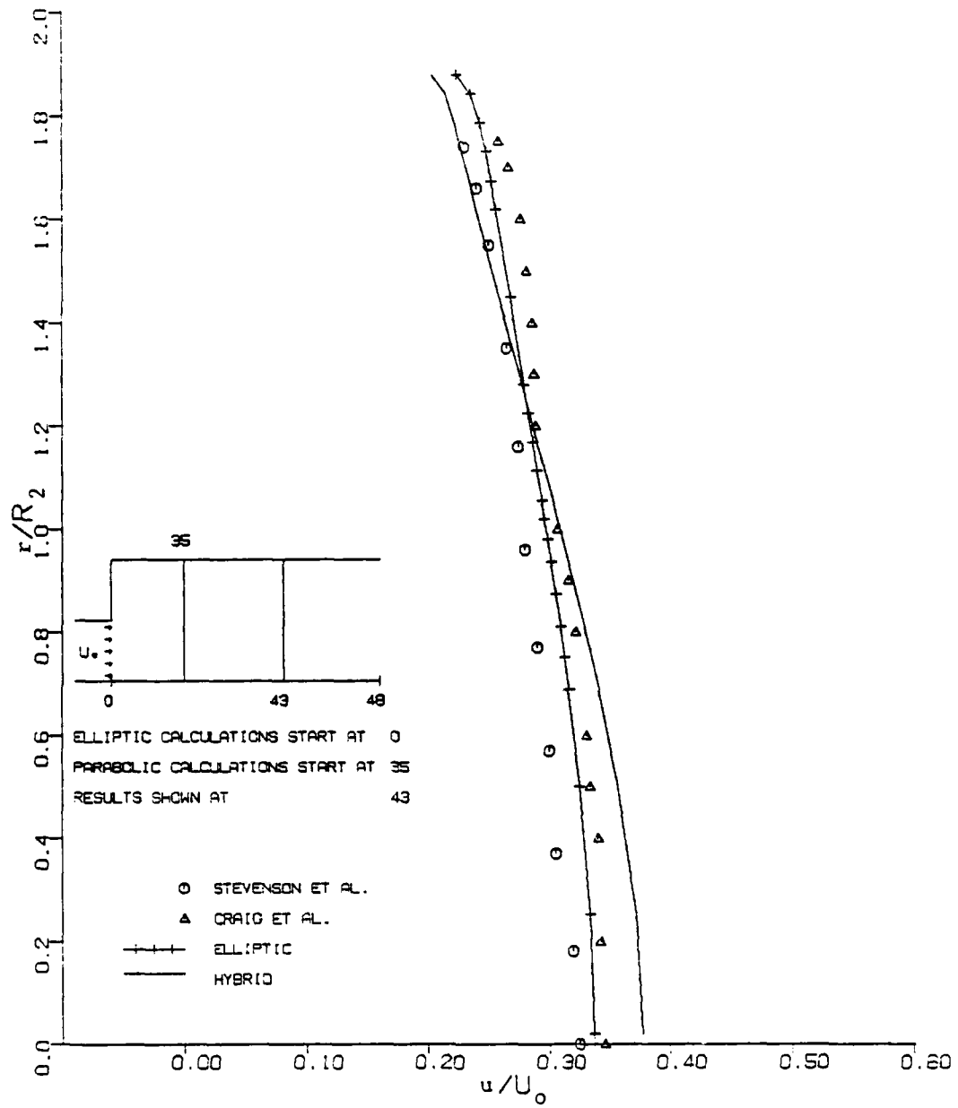
Fig. 3. Axial Velocity Results for the Hybrid Method, Elliptic Method, and Experimental Data at Station 43
