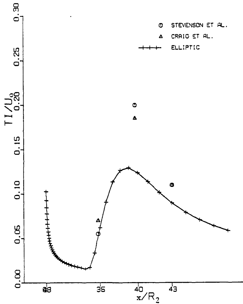
Fig. 10. Centerline Turbulent Intensity for Elliptic Calculations and Experimental Data at Each x Station
