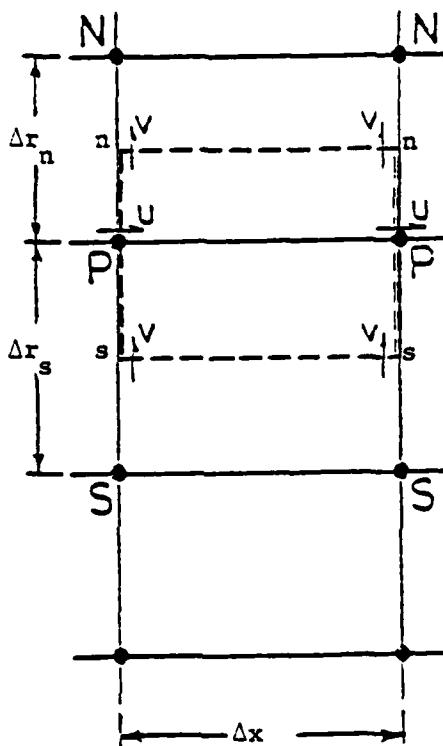
Fig. 2. Interior Parabolic Control Volume
