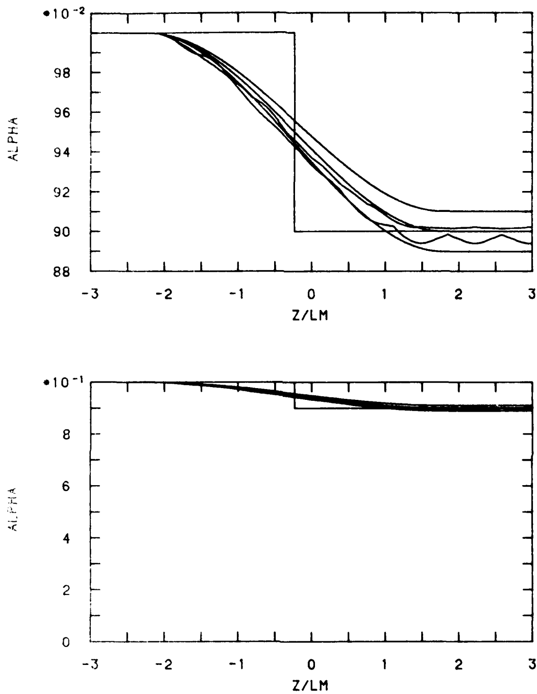
Figure 25. Extreme Values and Estimated Bounds of Gas Volume Fraction at a Particle Aggregate Boundary
