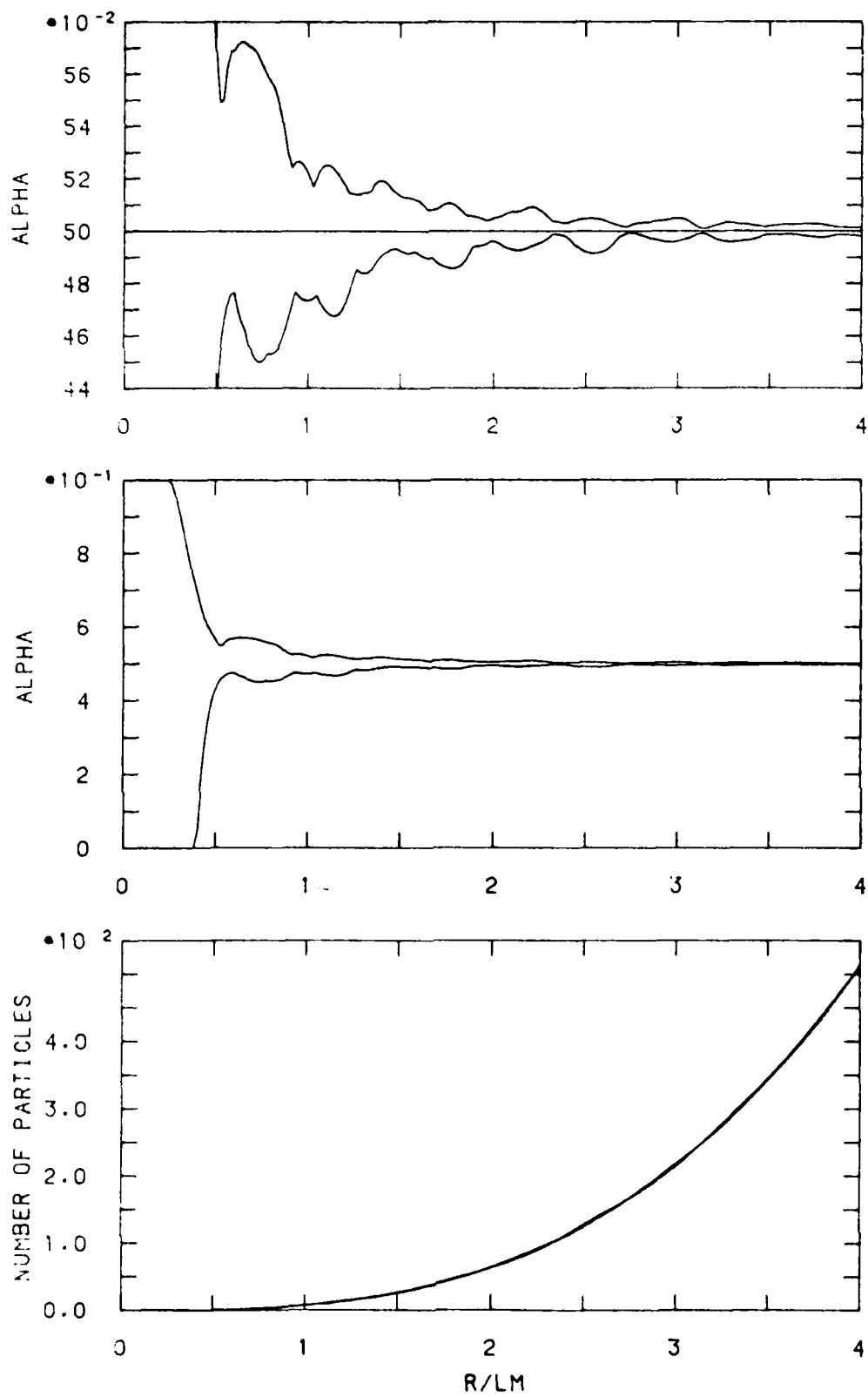
Figure 9. Extremes of Gas Volume Fraction as Functions of Averaging Radius Triangular Cylinder Lattice, \bar{\alpha} = 0.5 ; s/L_m = 0.3969
