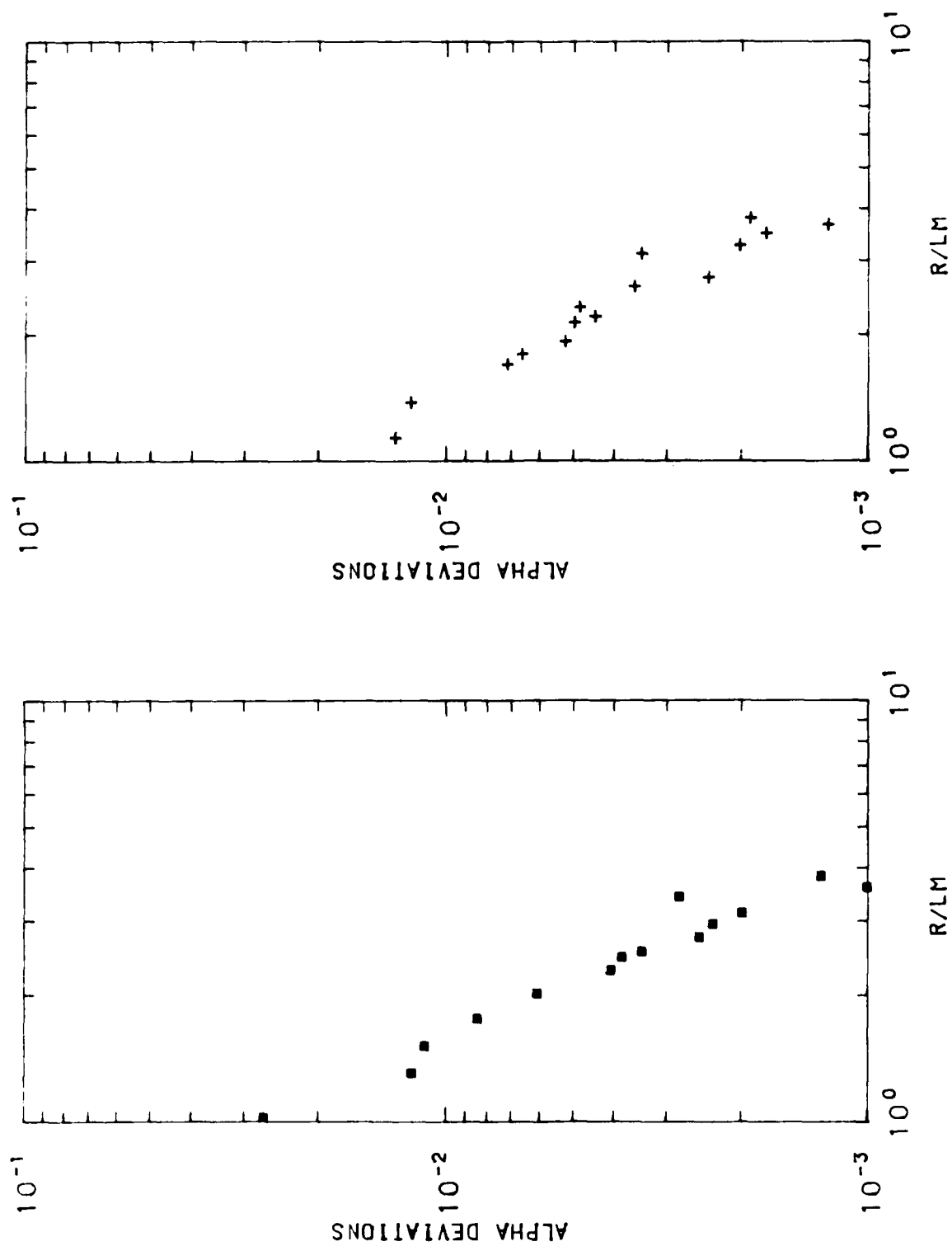
Figure 16. Extreme Deviations of Gas Values Fraction
