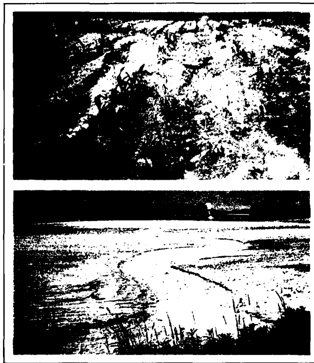
Figure 5 Soil Erosion in Lake Erie Basin.
