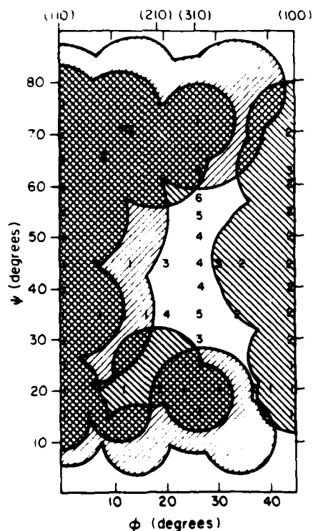
Fig. 11. Plot of regions where third layer atoms are hidden by first layer atoms (\\\\) and second layer atoms (///) as a function of \phi and \psi . For comparison an intensity map for \text{Ne}^+ scattering from clean Fe is also shown.
