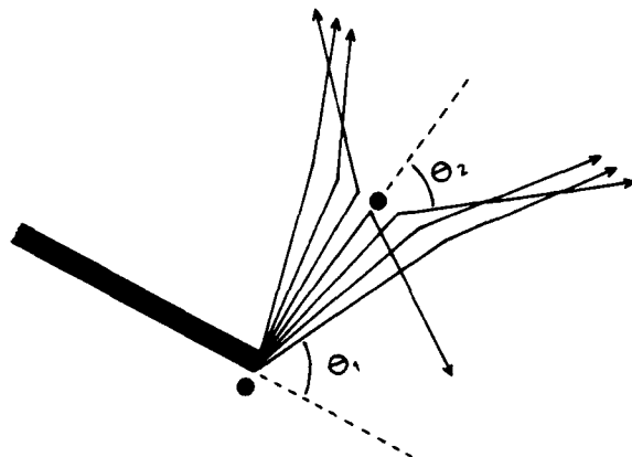
Fig. 8. The trajectories of ions scattered from an atom, showing blocking by a second atom.
