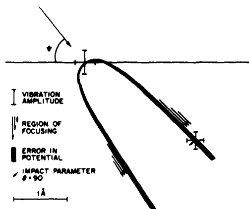
Fig. 12. Shadow cone calculated for 9.5 keV \text{Ne}^+ scattering from Fe showing the magnitude of various sources of error in this analysis. The error in the potential refers to the discrepancy between the dimensions calculated using the Firsov and Molière-Thomas-Fermi potentials.
