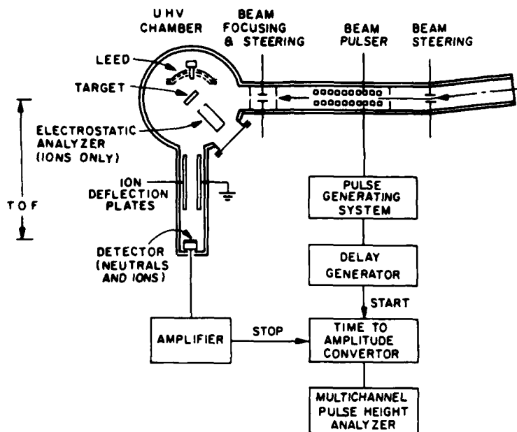
Fig. 3. Diagram of the system used for LEIS measurements.
