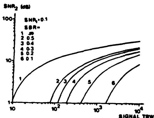
Fig. 2. Effect of SBR and signal TBW on output SNR_2 for a time-integrating correlator.
