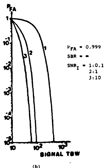
Fig. 3. Effect of input SNR_1 and signal TBW on detection performance for a time-integrating correlator: (a) P_D (for P_{FA} = 0.001 ) and (b) P_{FA} (for P_D = 0.999 ).
