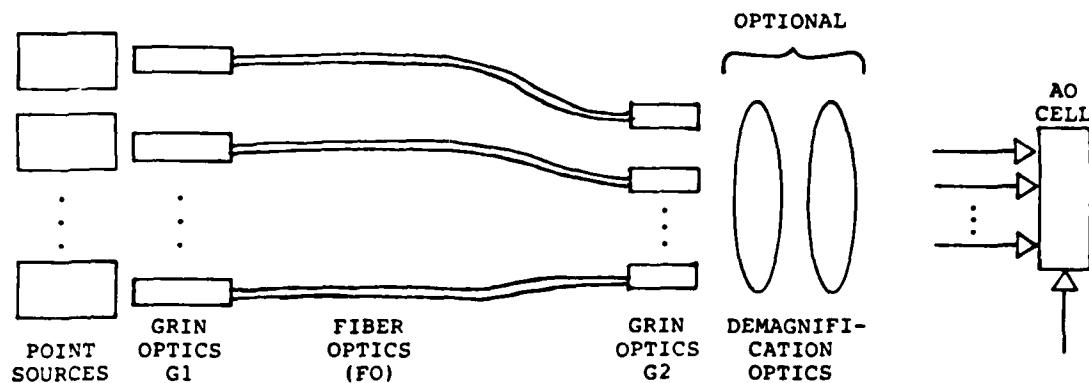
FIGURE 4: GRIN Optics Source and AO Cell Coupling Using Fiber Optics (FO).
