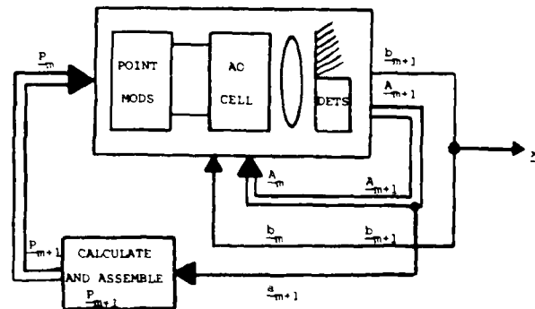
Fig. 11. Simplified schematic of an optical processor for the direct solution of a system of LAEs (a combined version of Figs. 10 and 7 or 9)
