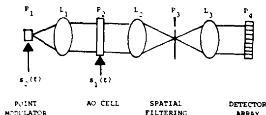
Fig. 1. Schematic diagram of a time-integrating acoustooptic correlator.
