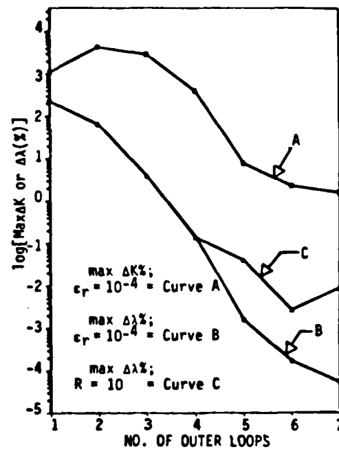
FIGURE 3 Variation of the error measures \Delta K_{\max}(\%) and \Delta \lambda_{\max}(\%) with the number of outer-loop iterations K for different inner-loop iteration stopping criteria for the third-order HPG3 F100 model
