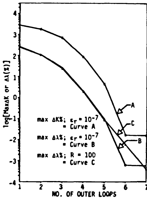
FIGURE 2 Variation of the error measures \Delta K_{\max}(\%) and \Delta \lambda_{\max}(\%) with the number of outer-loop iterations K for different inner-loop iteration stopping criteria for the fifth-order HPG3 F100 model
