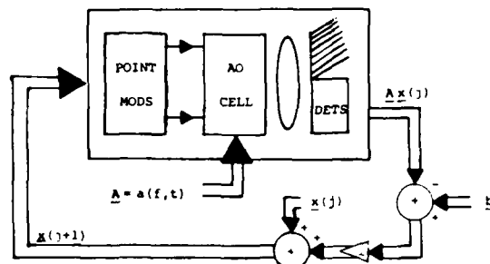
Fig. 6. Simplified schematic of an optical processor [13] to solve LAEs with general matrices using indirect algorithms
