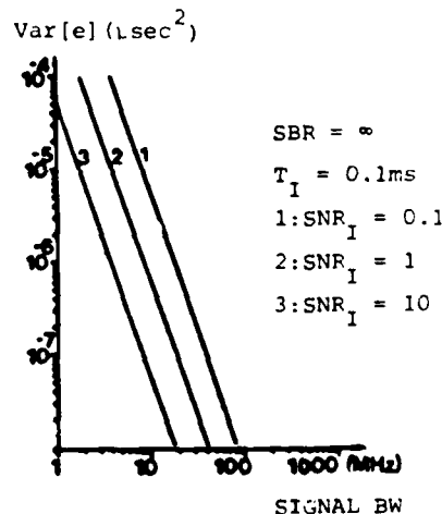
Fig. 6. Effect of \text{SNR}_I and signal BW on the variance \text{var}[e] of the delay estimation error e for a time-integrating correlator.
