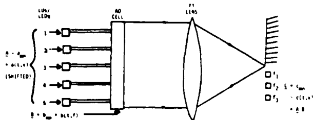
Fig. 1. Schematic diagram of a frequency-multiplexed acousto-optic systolic array processor. 3
