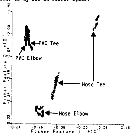
FIGURE 2 Multiclass Node-0 Fisher Projection for the Database of 9 Pipe Parts.
