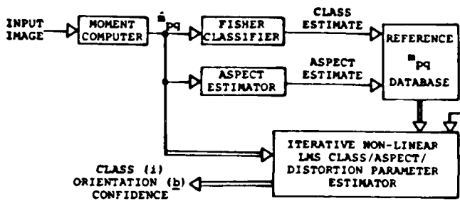
FIGURE 1 Block diagram of our Two-Level Moment-Based Classifier.
