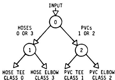
FIGURE 5 Hierarchical Node Tree for Class Estimation in the Level-One Classifier.
