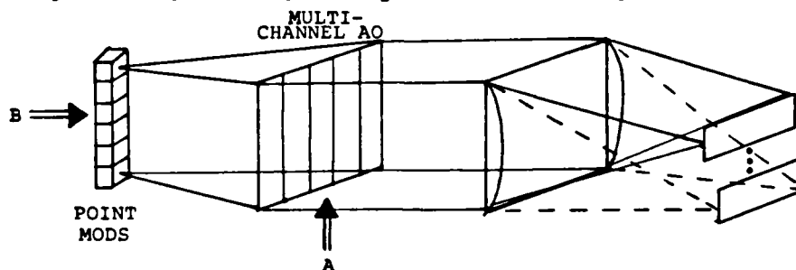
FIGURE 3: Multi-Channel AO Modulator/Deflector Frequency-Multiplexed AO systolic processor.
