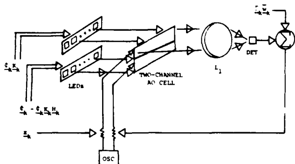
Fig. 1. Schematic diagram of an optical systolic processor for Kalman filter state estimation.
