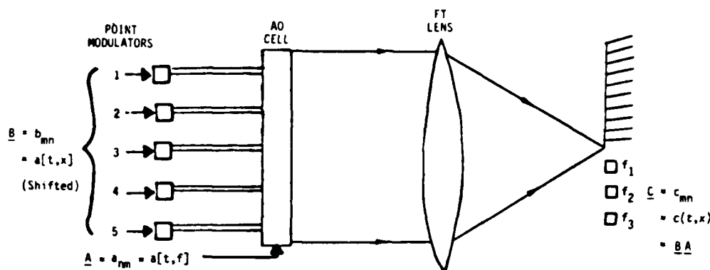
Fig. 4. Simplified schematic of a frequency-multiplexed general-matrix acoustooptic (AO) systolic processor [13] with both local and global interconnections and with a matrix-vector multiplication as its basic operation.
