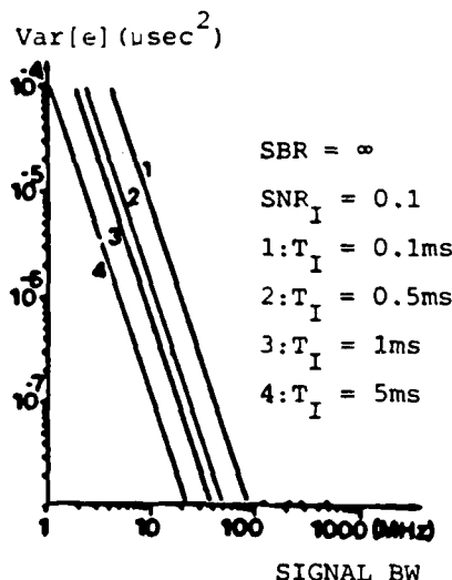
Fig. 5. Effect of integration time T_I and signal BW on the variance \text{var}[e] of the delay estimation error e for a time-integrating correlator.
