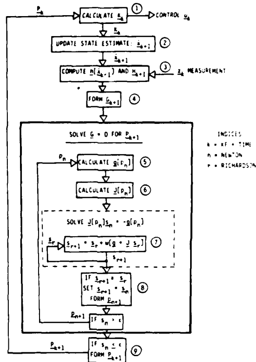
Fig. 2. Triple-nested discrete-time EKF algorithm.
