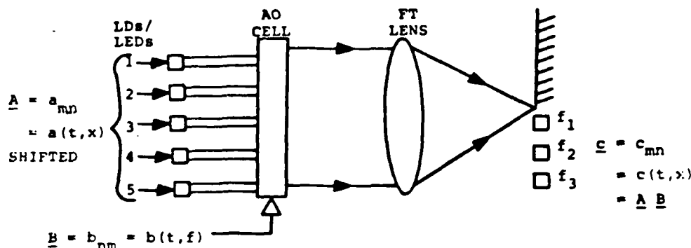
FIGURE 1 Schematic diagram of a frequency-multiplexed AO systolic array processor.
