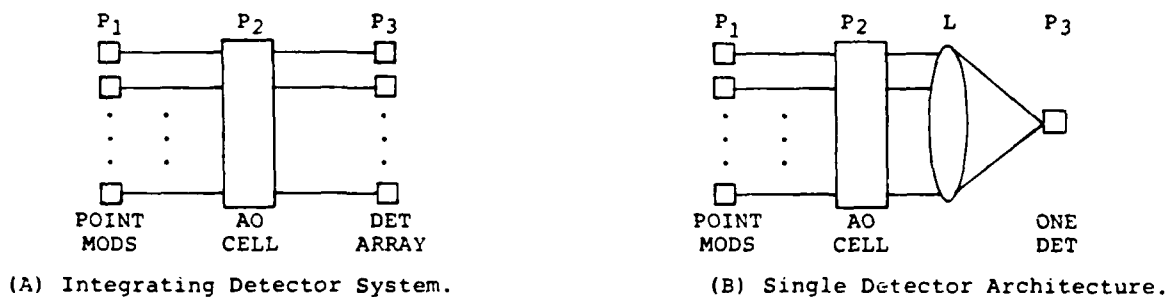
FIGURE 1: Two Basic Acousto-Optic Modulator Vector Inner Product Processors.
