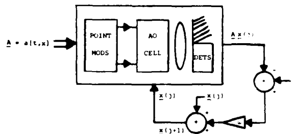
Fig. 5. Simplified schematic of an optical systolic processor [10] to solve banded-matrix LAEs by indirect algorithms
