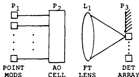
FIGURE 2: Frequency-Multiplexed Modulator/Deflector Acousto-Optic Matrix-Vector Processor.
