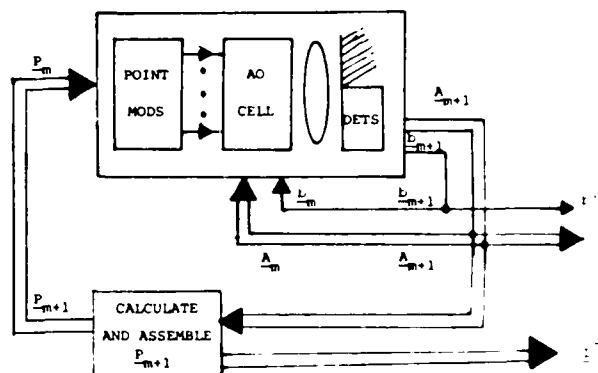
Fig. 7. Simplified schematic of an optical systolic processor [28] to perform LU matrix decomposition of a general matrix by Gaussian elimination
