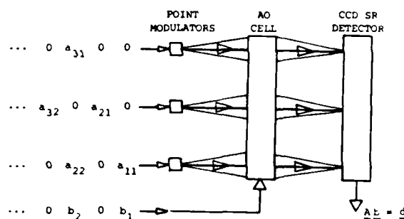
Fig. 1. Simplified schematic of a banded-matrix optical systolic processor using CCD shift register (SR) detector readout (adapted from [9]).
