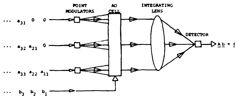
Fig. 2. Simplified schematic of a banded-matrix and Toeplitz-matrix optical systolic processor [10] with only a single detector. This architecture exhibits local and global interconnections and performs a vector inner product as its basic operation
