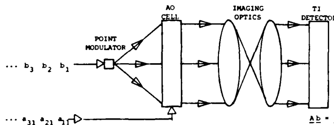
Fig. 3. Simplified schematic of a Toeplitz-matrix optical systolic processor [10] for matrices with large bandwidths
