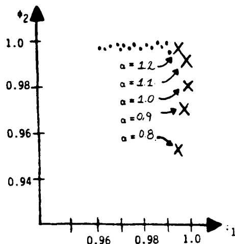
FIGURE 2. Intensity-Only WRD Fourier Transform Features Projected onto Dominant Tank/Truck Eigenimages (for 25 Image Database). \phi_1 =Dominant Truck Eigenimage; \phi_2 =Dominant Tank Eigenimage; \bullet =Tank Images; \times =Truck Images.
