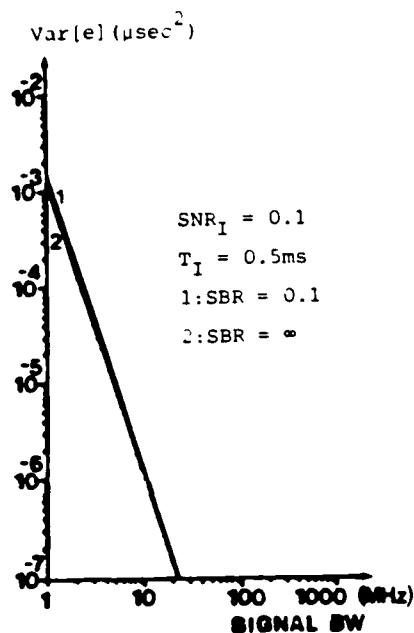
Fig. 7. Effect of SBR and signal BW on the variance \text{var}[e] of the delay estimation error e for a time-integrating correlator.
