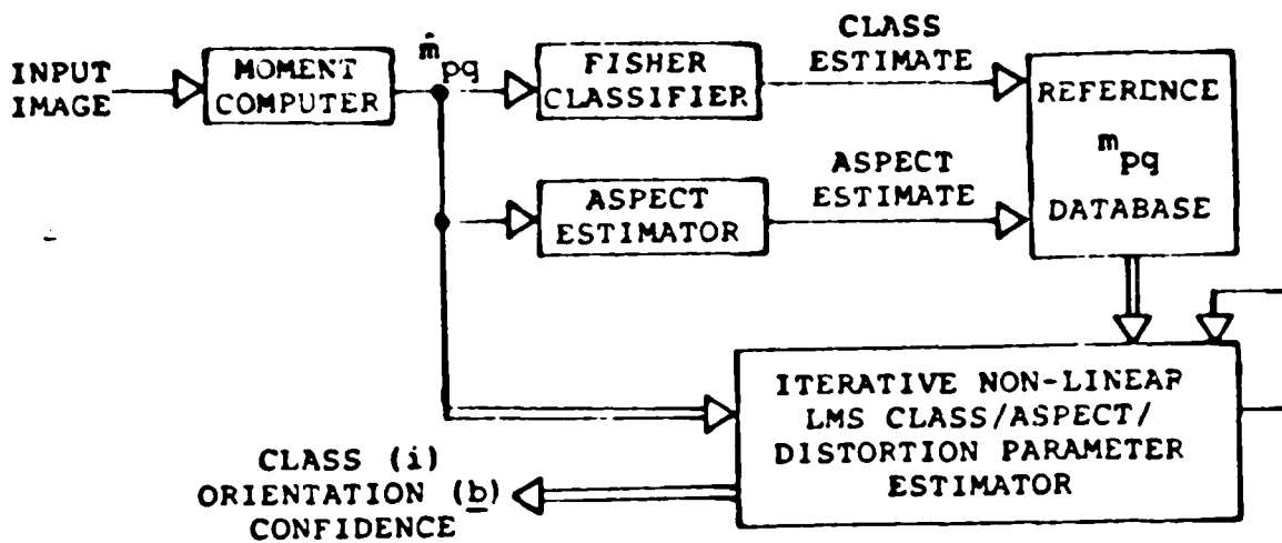
FIGURE 6 Full hybrid optical/digital moment feature-space two-level classifier pattern recognition system
