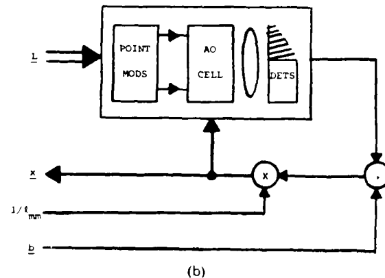
Fig. 10. Simplified (a) and detailed (b) schematic for an optical systolic processor [30] to solve triangular LAEs
