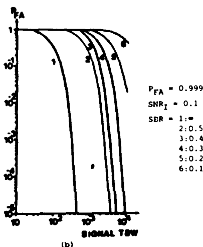
Fig. 4. Effect of SBR and signal TBW on the detection performance of a time-integrating correlator: (a) P_D (for P_{FA} = 0.001 ) and (b) P_{FA} (for P_D = 0.999 ).
