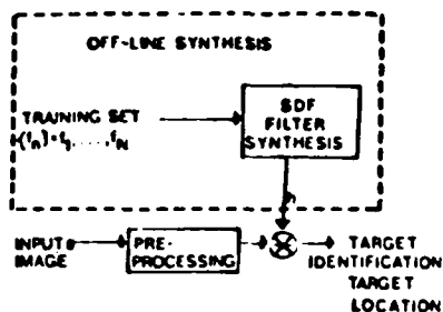
Fig. 2. Simplified block diagram of the off-line synthetic discriminant function synthesis from training set data and the use of such filters for on-line correlation of the SDF with unknown input imagery.
