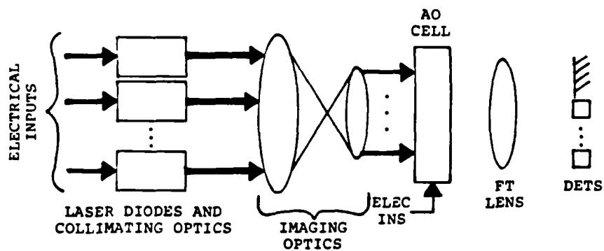
FIGURE 6: Architecture Using Separate Laser Diodes and Individual Collimating Optics.
