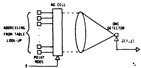
Fig. 3. Optical random-access AO storage/multiplier/summer for calculation of the Jacobian.
