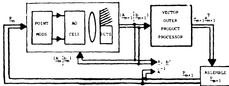
Fig. 9. Simplified schematic of an optical systolic processor [29] to perform QR matrix decomposition on a general matrix
