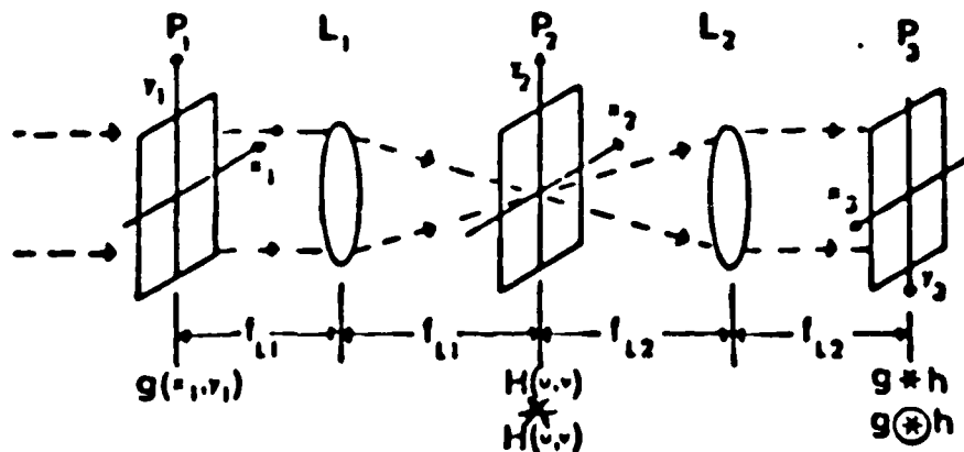
FIGURE 1 Coherent optical Fourier transform and correlation processor
