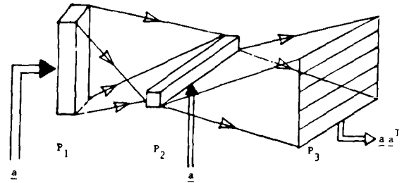
Fig. 8. Simplified schematic of an optical systolic vector outer product processor (adapted from [55])
