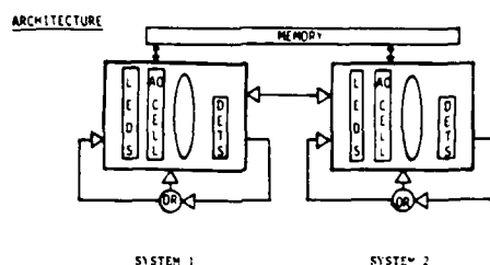
Fig. 4. Optical systolic discrete-time EKF processor architecture.
