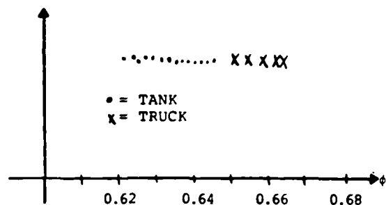
FIGURE 4. Projections of 25 Image/Class Tank/Truck Data on Best Foley-Sammon Vector.
