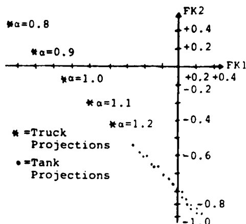
FIGURE 3. Intensity-Only WRD Fourier Transform Feature Projections for Tank/Truck Images onto FK Vectors (25 Images/Class).
