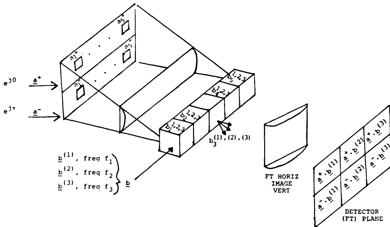
FIGURE 7: Bipolar and Complex-Valued Data Handling Using Space and Frequency-Multiplexing.
