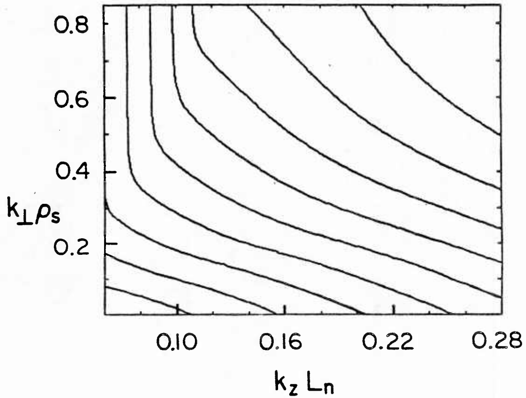
FIG. 11. Variation of (a) the real frequency and (b) the growth rate in the k_z L_n - k_\perp \rho_s plane. The parameters are \delta = 0.2 , (v_\perp)_0 / U_b = 0.5 , \Delta = 0.0 , and v_{ti} / U_b = 0.20 . The contour interval in (a) is 0.883 \omega_{\max}^* with the maximum of 0.9936 \omega_{\max}^* occurring to the right; the contour interval in (b) is 0.00552 \omega_{\max}^* with a maximum of 0.0552 \omega_{\max}^* .
