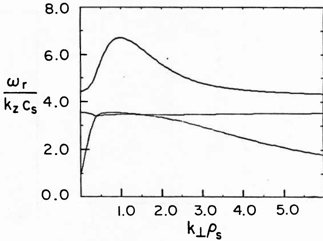
FIG. 2. Real frequencies for a numerical solution for a typical set of parameters; \delta = .1 , U_b/c_s = 4.0 , v_{n1}/U_b = 0.05 , v_{j1}/U_b = 0.0 , and k_z L_n = .1 . The peak in the growth rate occurs just after the intersection of the real frequencies.
