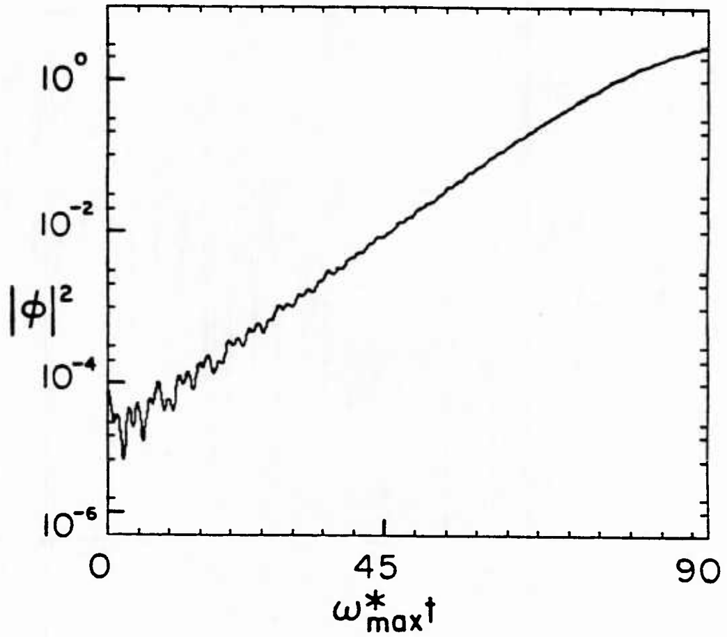
FIG. 9. Time histories of (a) the square of the mode amplitude and (b) the square of the real portion of the potential for a given position in z . For this simulation v_{ii}/U_b = 0.19 . Random excitation was used to initialize the simulation.
