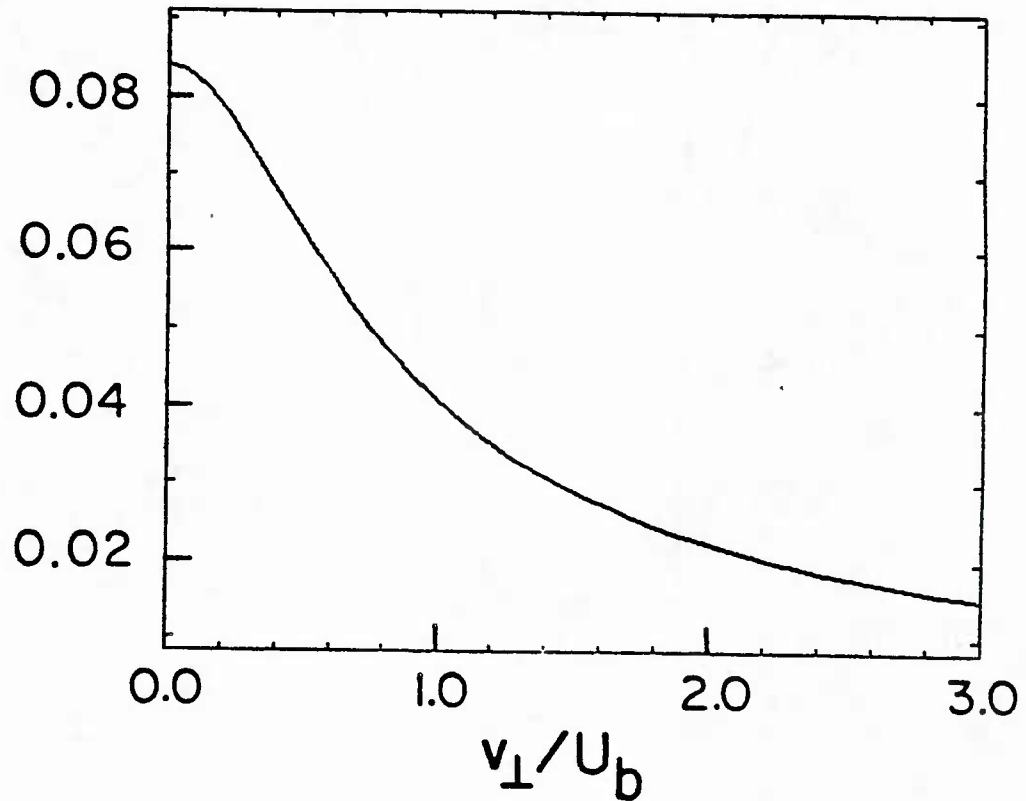
FIG. 4. (a) Normalized maximum growth rate maximized over the \mathbf{k} vector as a function of v_{\perp}/U_b and the corresponding values for (b) the normalized real frequency \omega_r/\omega_{\max}^* , (c) k_{\perp}\rho_s and (d) k_{\perp}L_n .
