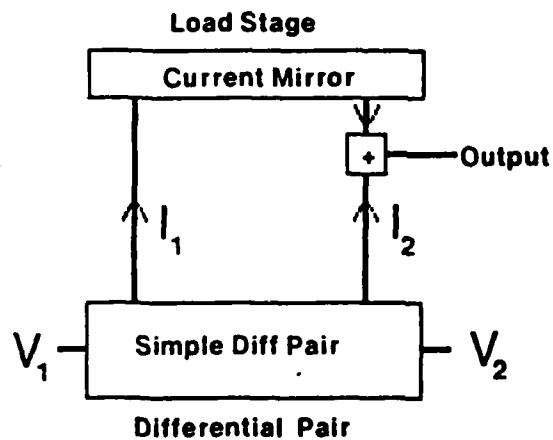
Fig. 7. Abstract First Stage The first stage of an operational amplifier is usually composed of a differential pair with a load.
