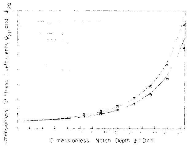
Figure 7 - Stiffness coefficients \psi_{2c} and \psi_{2o} versus \phi for double-notched stringers under two-point load. Dimensions (see fig. 2): l = 48 inches, h = 3.75 inches, t = 1.5 inches, s = 44 inches, W = 9 inches, a = 9 inches, m = 4.5 inches, and q = 8.5 inches. (ML84 5502)
