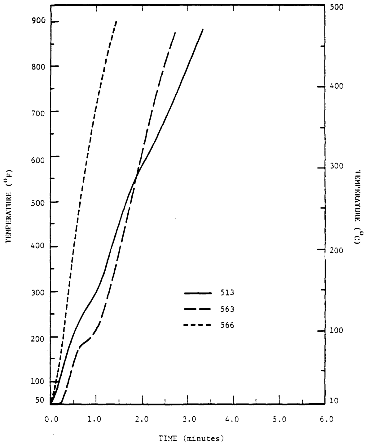
Figure 4-3. Glauber's Salt
