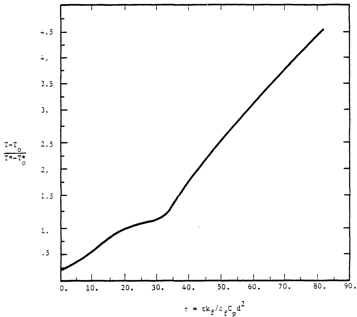
Figure 3-5. Model Prediction of Substrate Thermal Response - Large Endotherm
