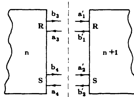
FIG. 4. Cascading of two successive scattering networks.
