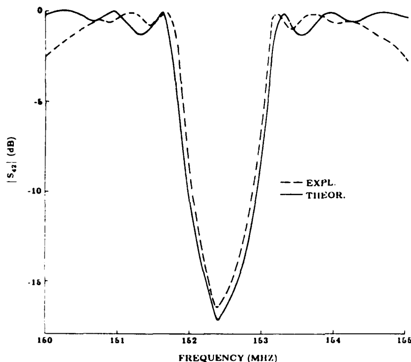
FIG. 5. Theoretical and experimental plot of |S_{42}| vs frequency ( h = 1088 \text{ \AA} ).
