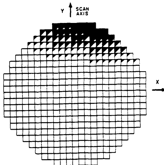
Figure 66. Phase Error at Feed Array (12 GHz) \xi = 90^\circ , \phi = 90^\circ , R4 = 4 in., Single Lens Design Case.
