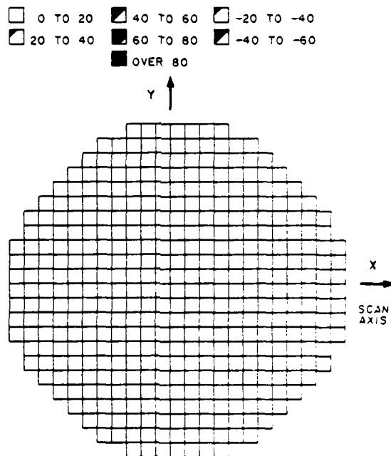
Figure 79. Phase Error at Feed Array (12 GHz) \xi = 81.3^\circ , \phi = 0^\circ , R_4 = 7 in., Optimized Feed Array, Minor Axis Lens Design.
