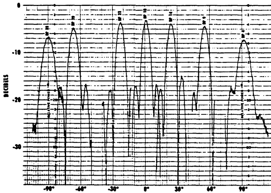
Figure A-8. WAAFL Measured Radiation Patterns (15 GHz).
