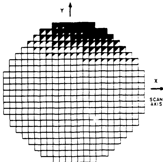
Figure 67. Phase Error at Feed Array (12 GHz) \xi = 90^\circ , \phi = 0^\circ , R4 = 4 in., Three Lens Design Case.
