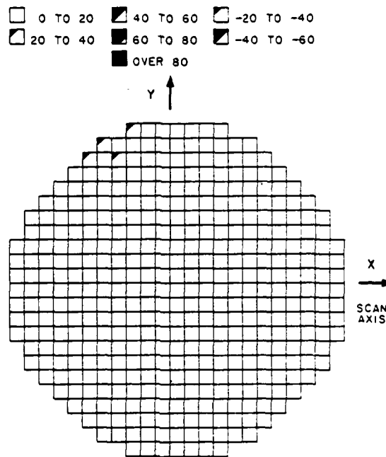
Figure 78. Phase Error at Feed Array (12 GHz) \xi = 71.2^\circ , \phi = 0^\circ , R_4 = 7 in., Optimized Feed Array, Minor Axis Lens Design.
