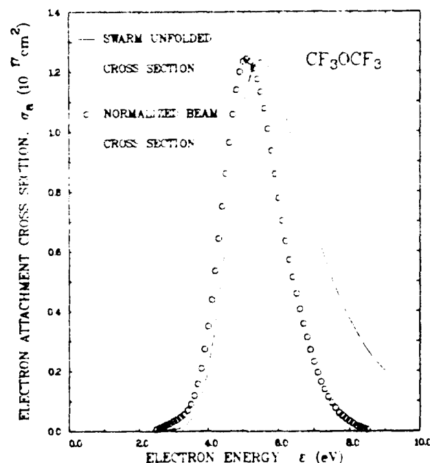
FIG. 6. Swarm unfolded total electron attachment cross section \sigma_a(\epsilon) for \text{CF}_3\text{OCF}_3 in comparison with the total negative ion cross section obtained in the TOFMS study. The TOFMS study cross section has been normalized to the peak in the unfolded cross section.
