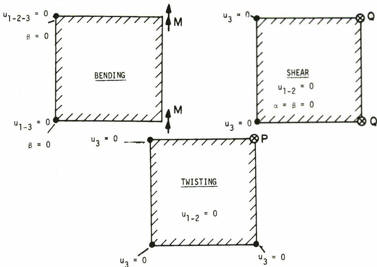
Figure 4 Patch tests
