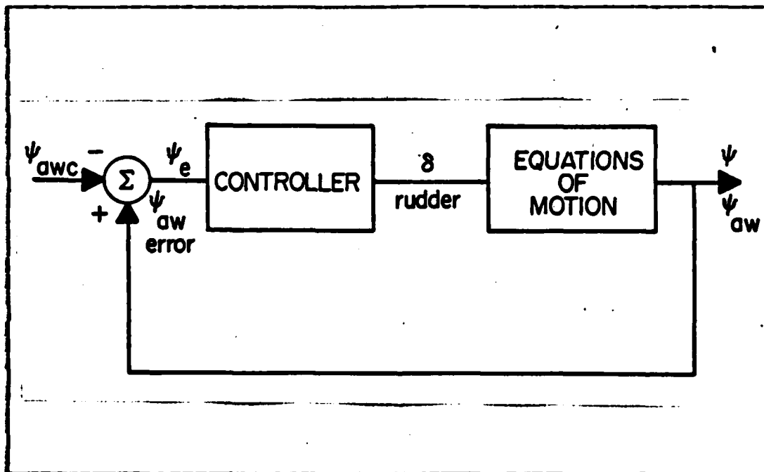
Figure 2.1 BLOCK DIAGRAM
