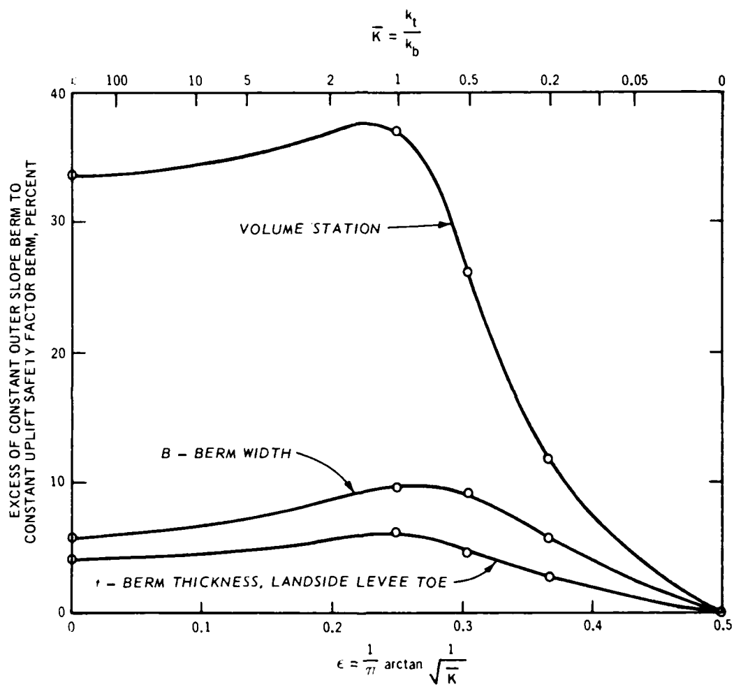
Figure 4. Percent excess of volume/station, berm width, and berm thickness at landside levee toe
