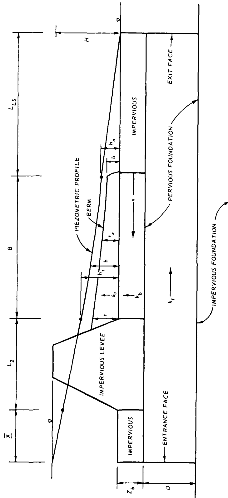
Figure 2. Transformed cross section
