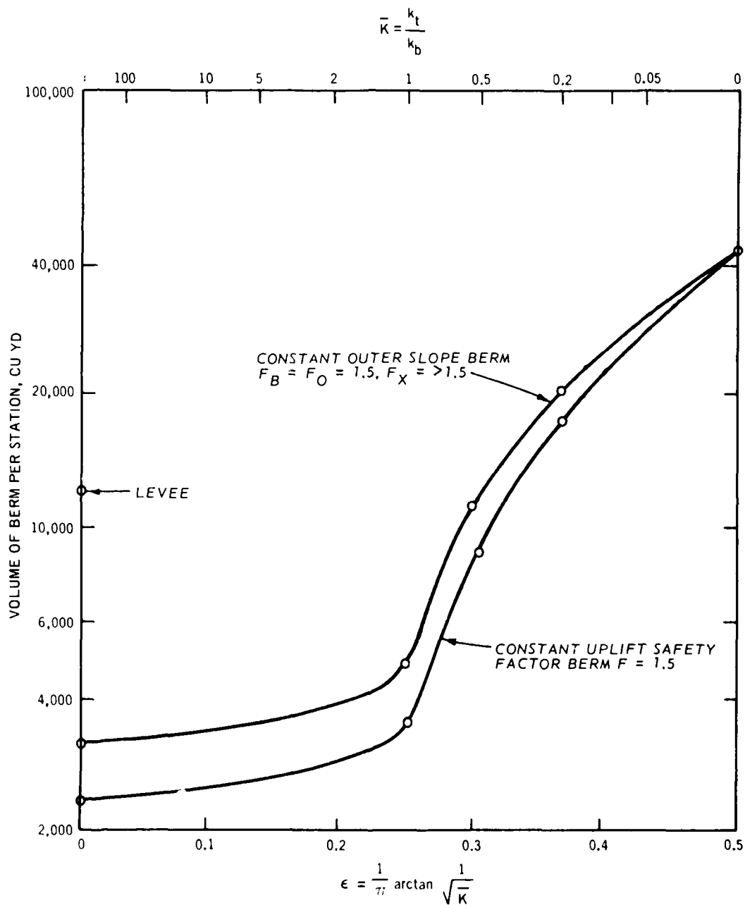
Figure 3. Volume of berm per station versus \bar{K}
