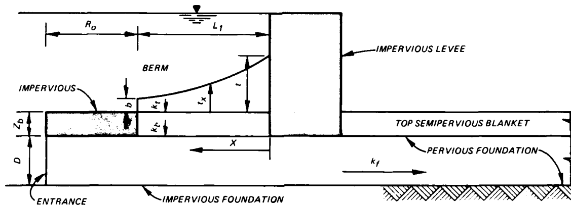
Figure 4. Constructed berm having a constant gradient
