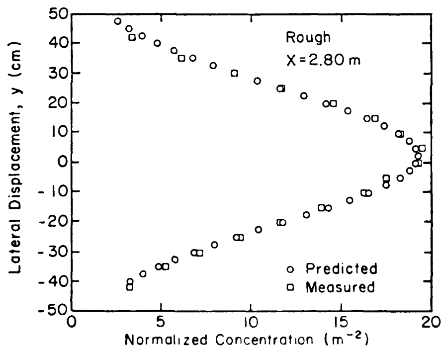
Figure 3-9. Horizontal concentration profiles for a ground-level source in neutral flow.
