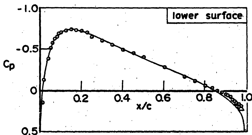
FIG. 7(a): C_p DISTRIBUTION - NACA 0020 AIRFOIL MODEL
