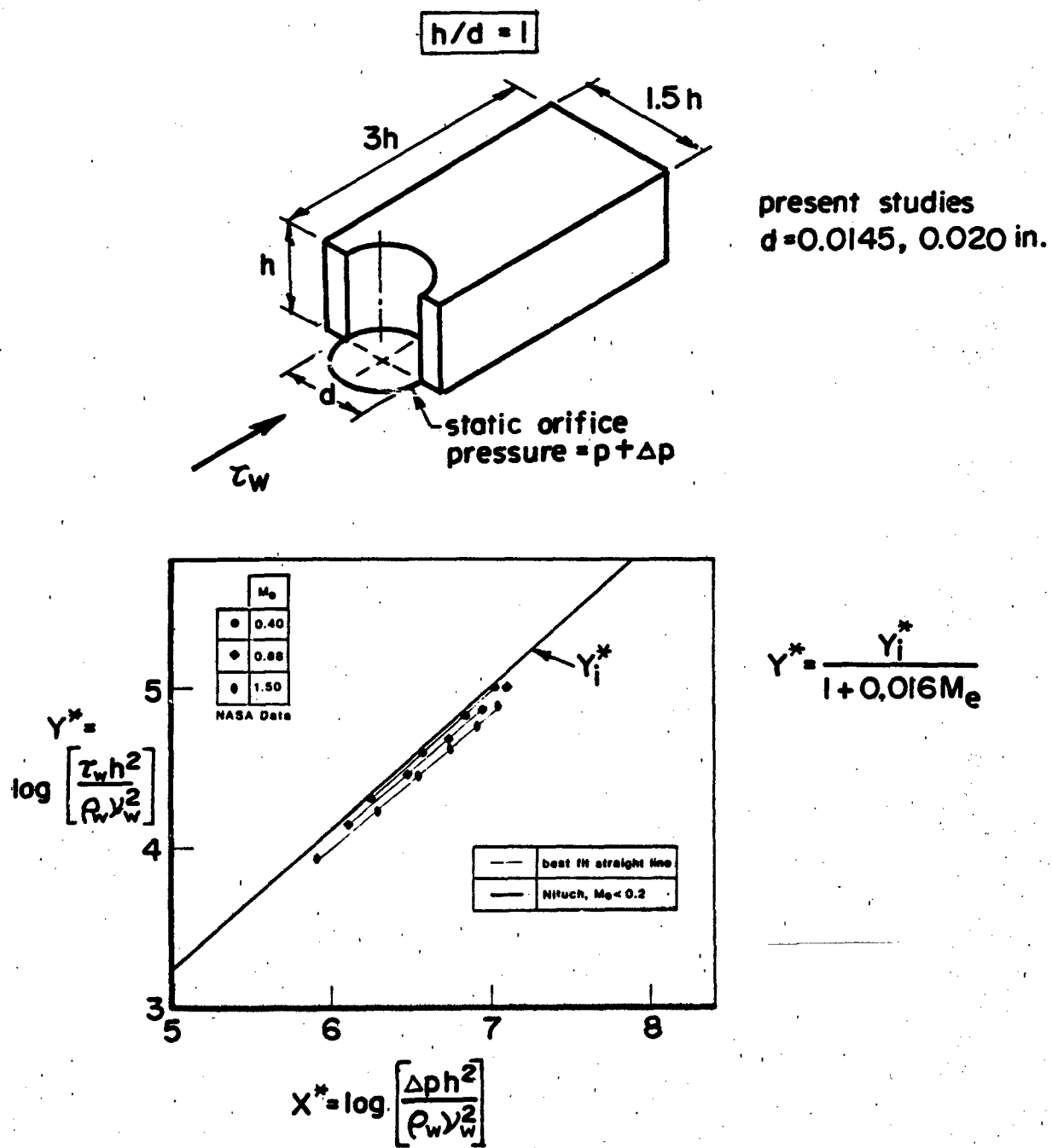
FIG. 6: THE CONGRUENT OBSTACLE BLOCK AS A SKIN FRICTION INDICATOR
