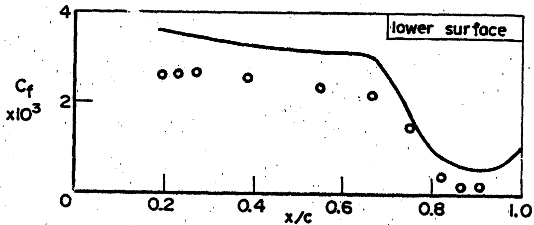
FIG. 13: CHECK ON GREEN'S C_f PREDICTION
