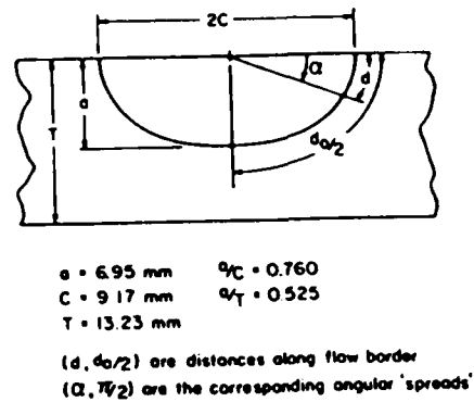
Fig. 11 Semi-Elliptic Surface Crack Geometry and Notation
