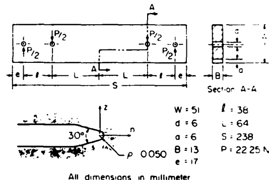
Fig. 7 Four Point Load Compact Bending Specimen
