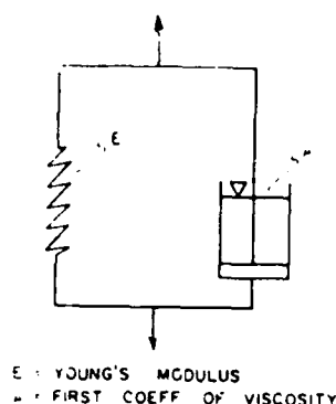
Fig. 1 Model of Kelvin Material
