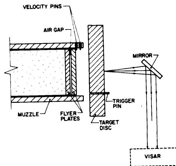
Figure 1. Double Flyer Geometry.
