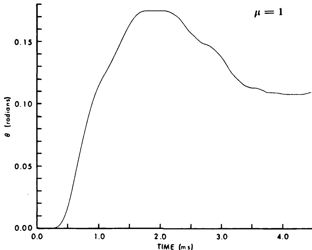
Figure 7. Predicted Rotation at Pinned End
