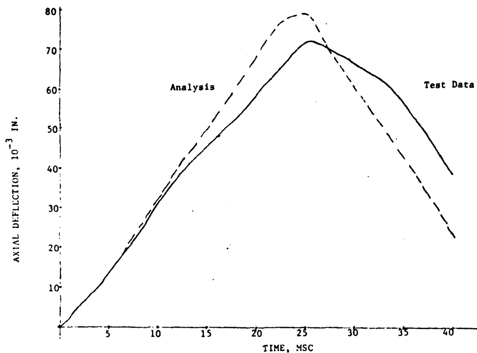
Figure 6. Axial Deflection of BRL Shock Tube for HATS Panel Test (Reflected Pressure = 14.5 psi)
