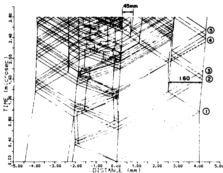
Figure 2. (x, t) Diagram for Double Flyer Impact, Shot 719.
