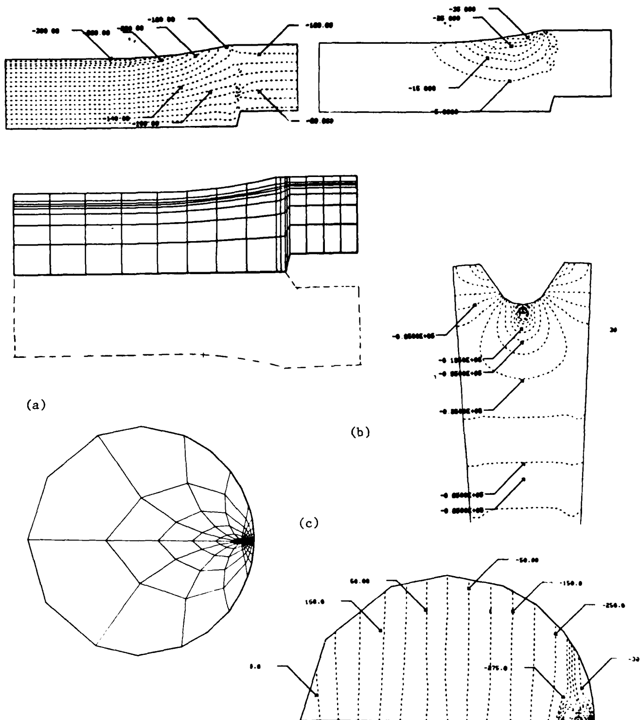
Figure 4 Torsional Stresses (a) Non uniform C.S., (b) Crack in Spline (c) Subsurface Crack in Shaft
