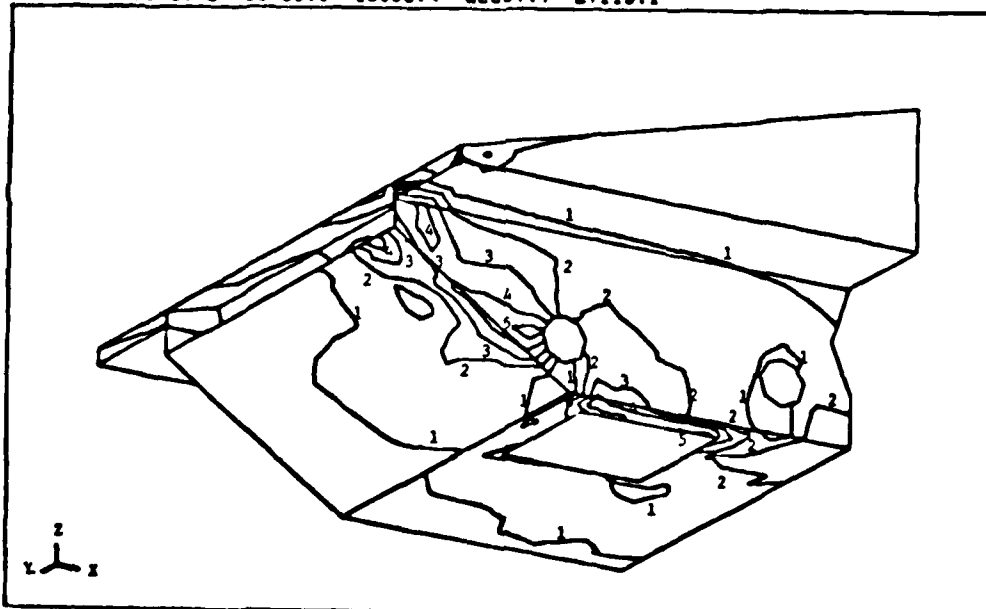
Fig. 6 - Front Idler Vertical Load Case Stress Contours
