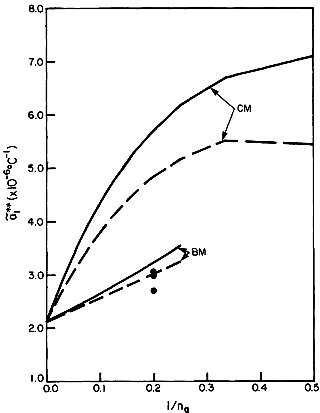
Figure 5 Comparison of theoretical predictions with the experimental results for 5 harness-satin graphite/epoxy composites. a/h = 3.75 ; —, a/h = 7.5 ; ---, and a_u/a = 1.0 . CM and BM indicate fiber crimp and bridging models, respectively. •: Experimental results at 300°K. n_g is defined in Sec. II.1.
