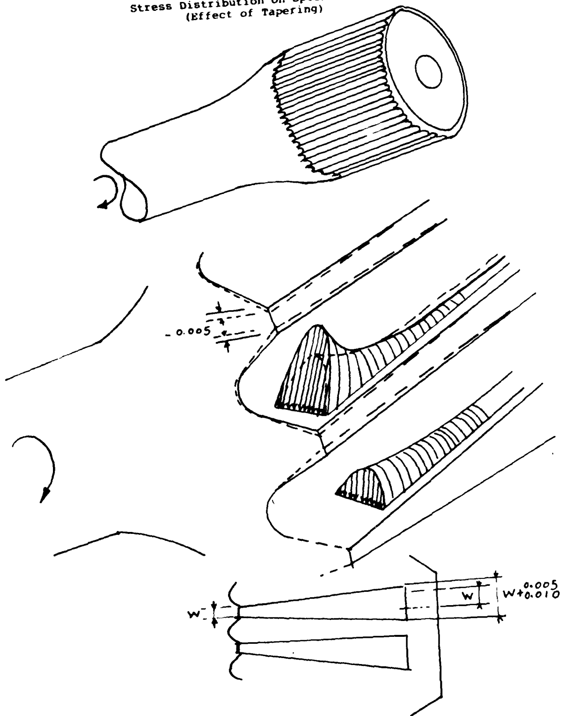
Figure 5 Redesign of Spline Teeth
