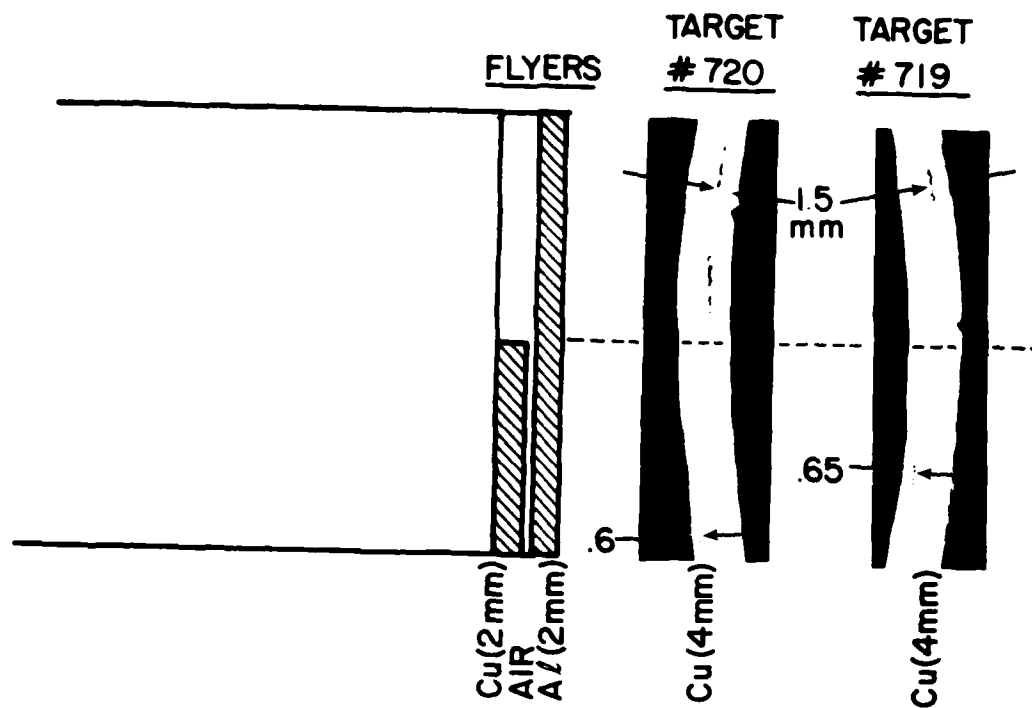
Figure 3. Damage Caused by Double and Single Flyer Impacts
