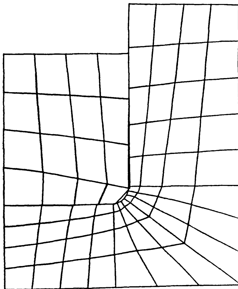
Figure 1. A finite element model for breech mechanism
