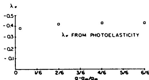
Fig. 9 \lambda_\sigma Distribution from Part Circular Flaw
