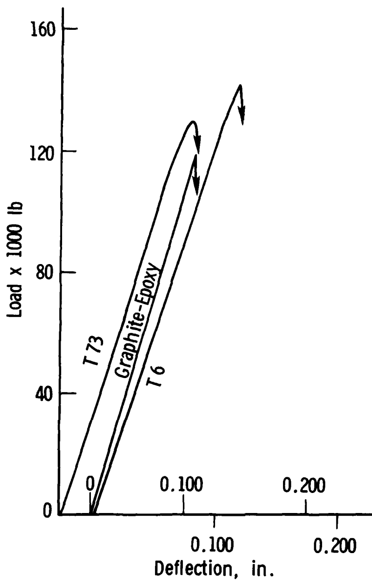
Figure 10. LOAD-DEFLECTION PLOTS OBTAINED FROM LUG SHEAR TESTS
