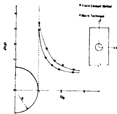
Figure 7. Comparison of stress concentration factors obtained by numerical and experimental techniques.
