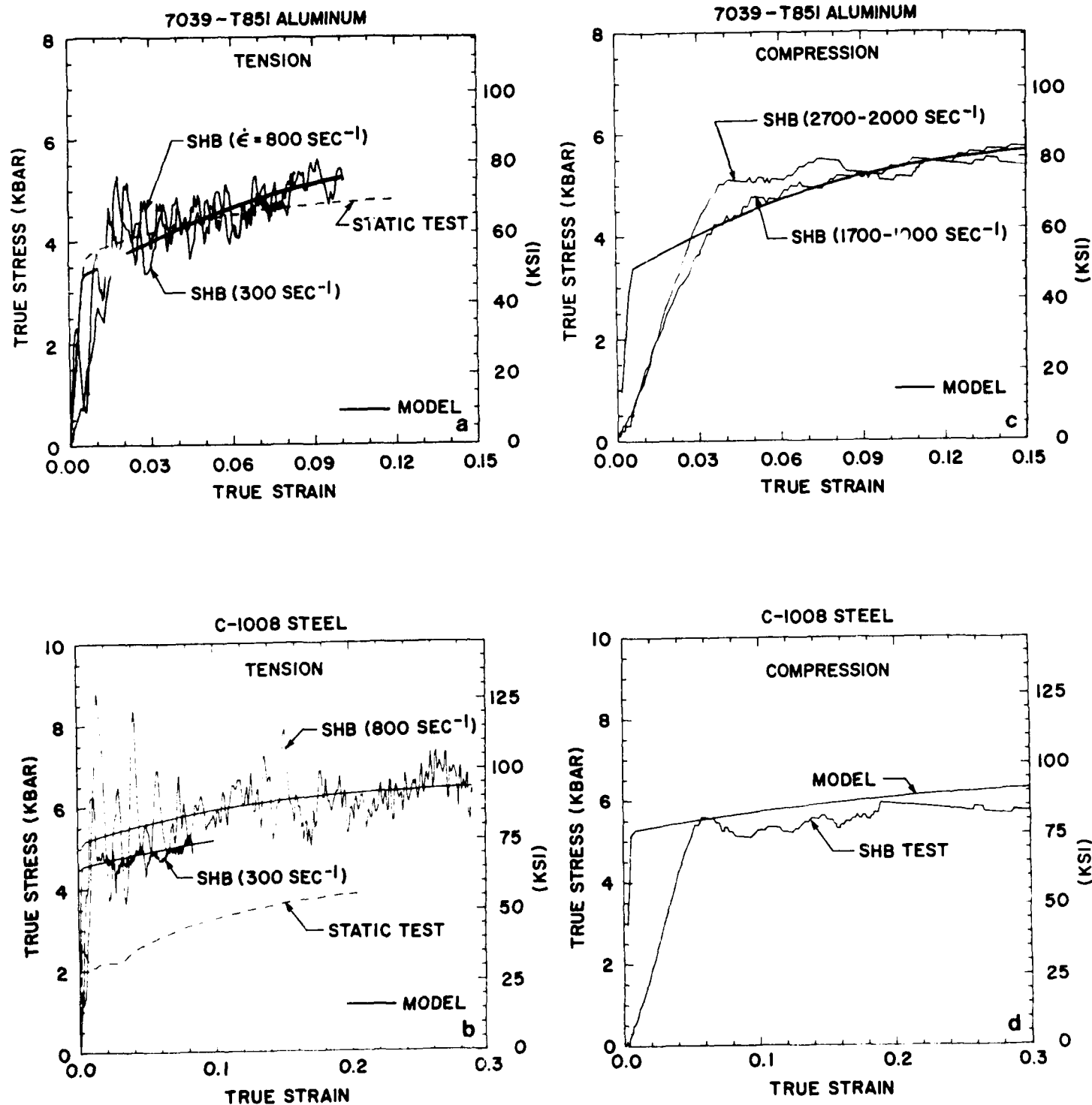
Figure 1. Comparison of Bodner-Partom Model Predictions With SHB Test Results.
