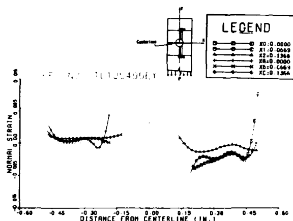
Figure 4. Strain parallel to load axis ( \epsilon_y ) along several lines in and opposite to the bearing region.
