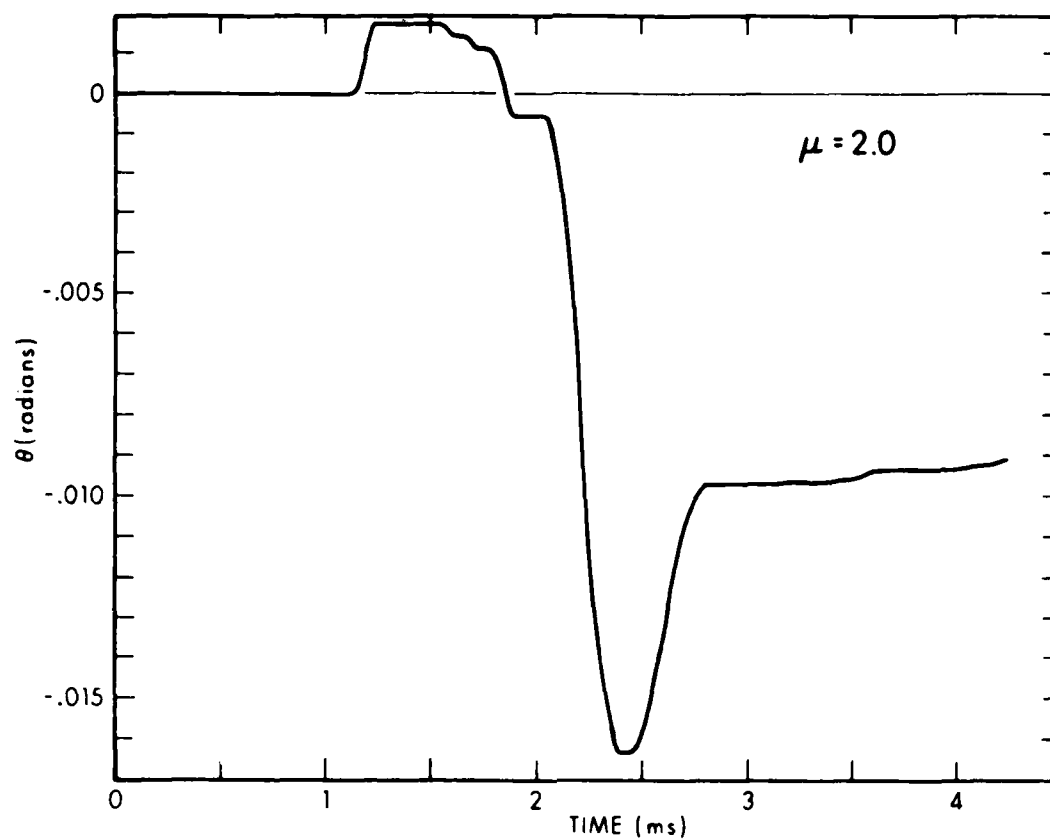
Figure 8. Rotation at Pinned End for Run J
