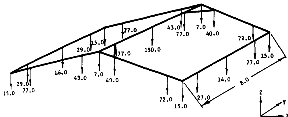
SNOW LOAD IN Z-DIRECTION
