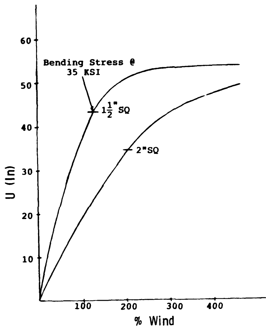
FIG. 19 MAXIMUM HORIZONTAL DISPLACEMENT UNDER WIND PRESSURE
