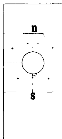
Figure 5. Distribution of tensile and compressive strain ( \epsilon_y ) near the fastener hole.
