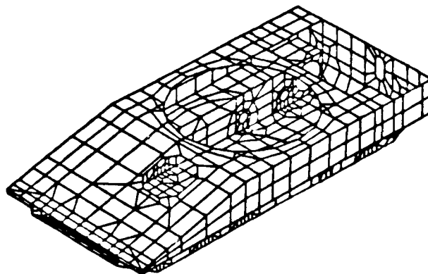
Fig. 2 - STM Hull System Model
