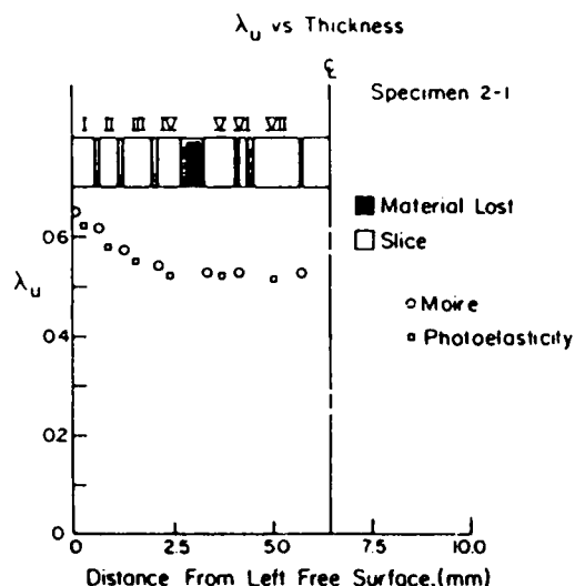
Fig. 8 \lambda_u Values from Moiré and Photoelastic Data
