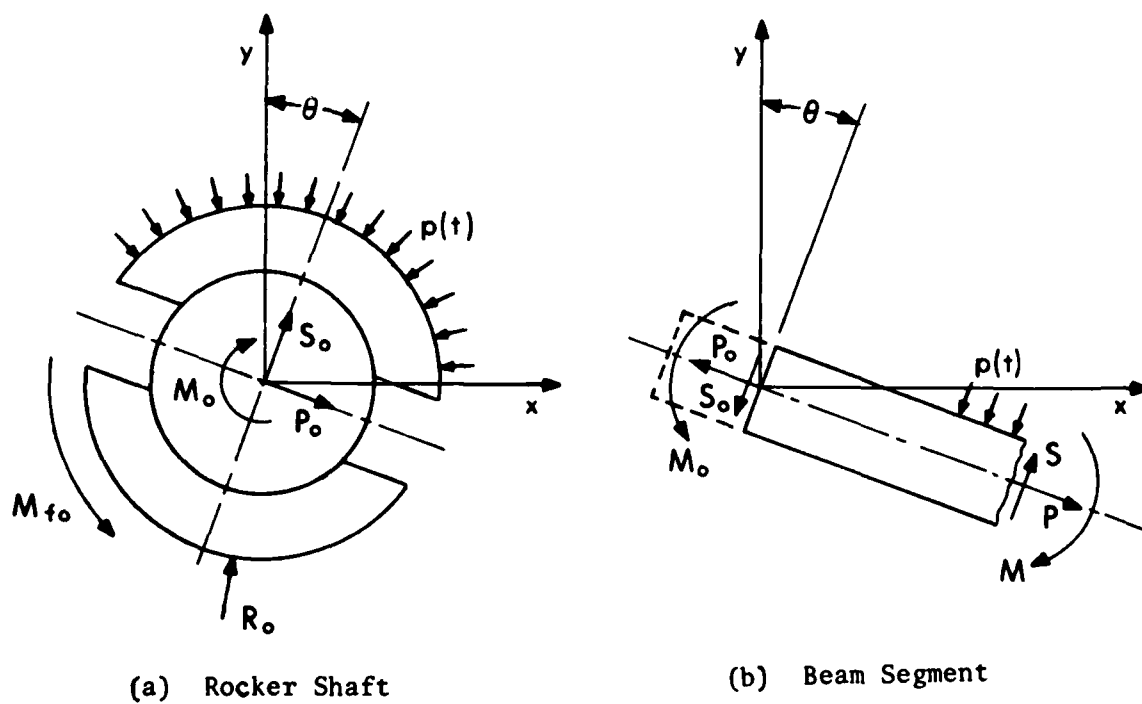
Figure 1. Pinned End Rocker Shaft Details
