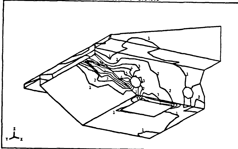
Fig. 5 - Front Idler Horizontal Load Case Stress Contours
