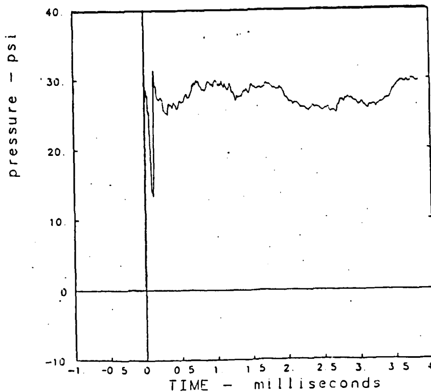
Figure 7. Reflected Pressure Loading for the Aluminum Sandwich Panel (Reflected Pressure = 27.5 psi)
