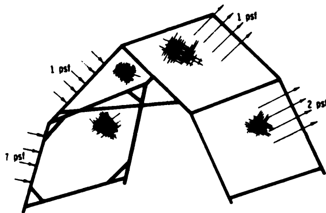
FIG. 4 WIND PRESSURE INTENSITY ON TEMPER TENT
