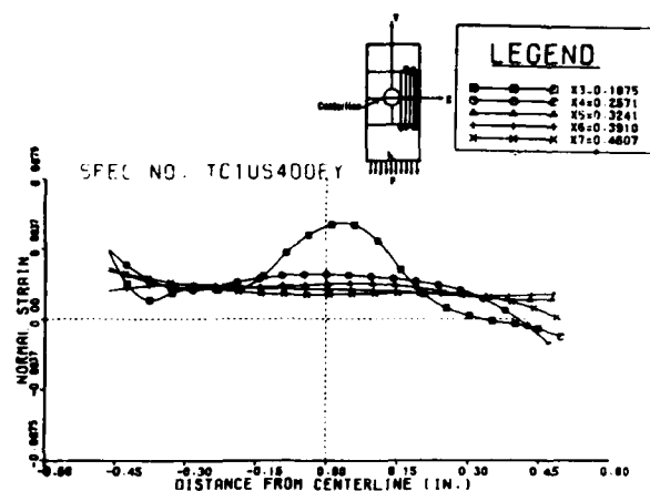
Figure 3. Strain parallel to load axis ( \epsilon_y ) along several lines encompassing a ligament region.
