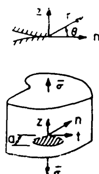
Fig. 2 General Problem Configuration and Notation
