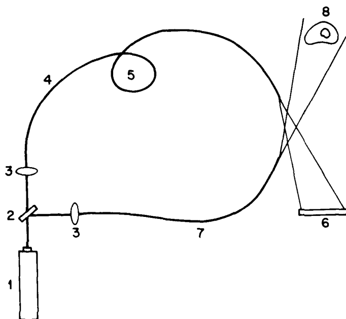
SET-UP FOR LOCAL FIBER OPTIC HOLOGRAPHY
