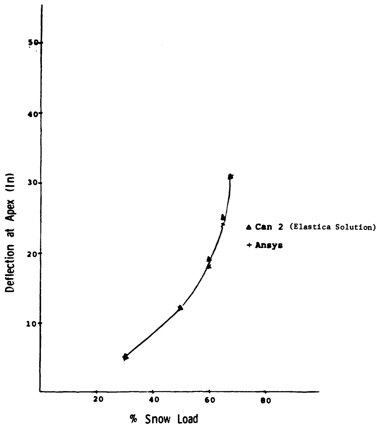
FIG 15 COMPARISON OF CAN 2 AND ANSYS SOLUTIONS 1-5" SQ
