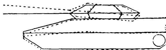
Fig. 10 - STM Bounce Mode @ 37.3 Hz
