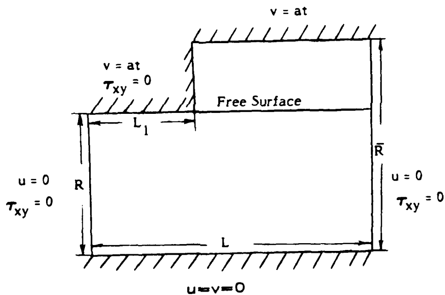
Figure 4. Boundary Conditions on Typical Section
