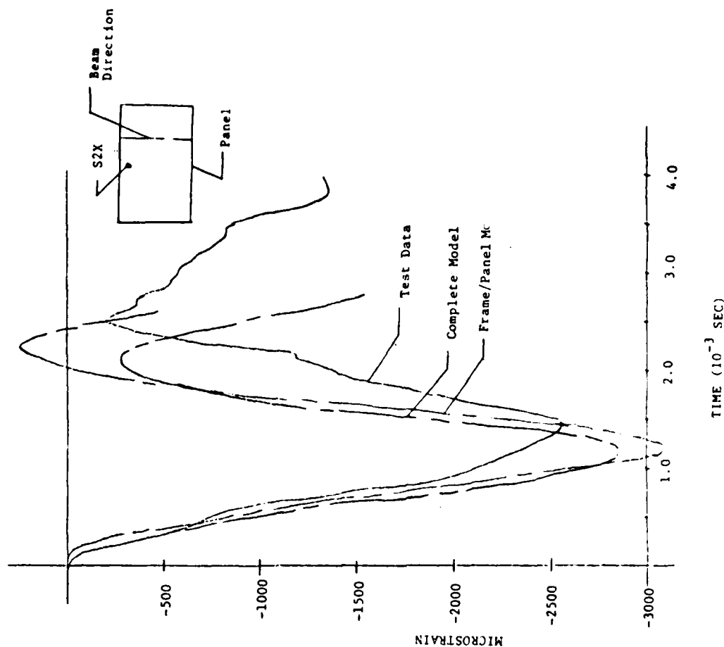
Figure 11. Graphite Sandwich Panel Face Strain at Panel Edge - Gage S2X (Reflected Pressure = 27.5 psi)
