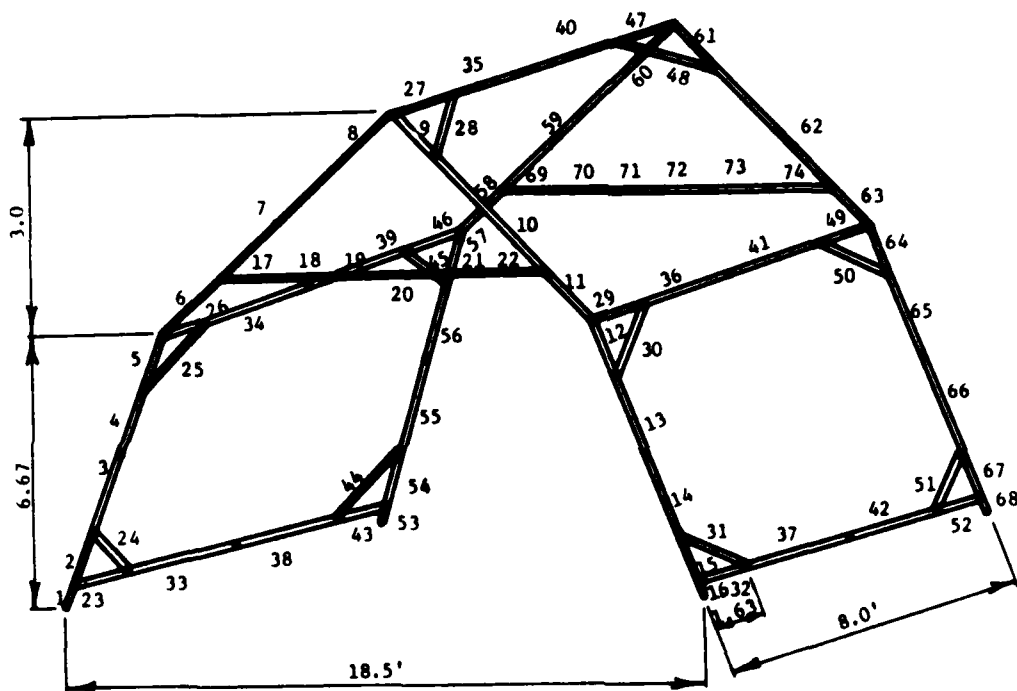
FIG. 3 LAYOUT OF TENT FRAME ELEMENTS
