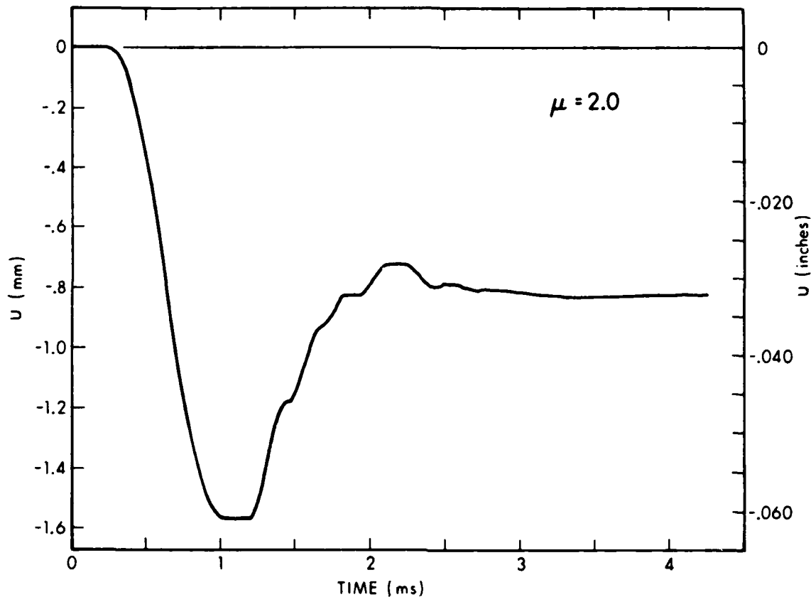
Figure 10. Displacement at Sliding-Hinged End for Run J
