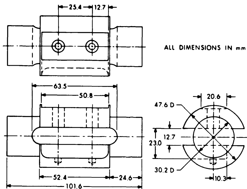
Figure 1. Pinned End Rocker Shaft Details
