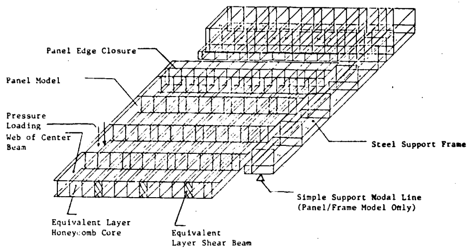
Figure 4. Sandwich Panel/Support Frame Model
