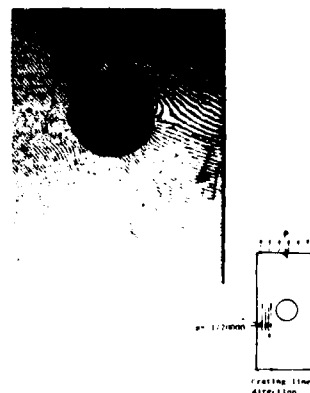
Figure 6. High sensitivity Moire fringes showing displacements perpendicular to the direction of loading for 130 lb. load with rotational mismatch.
