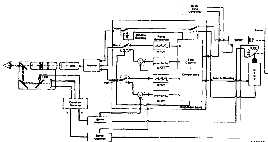
Figure 3-3 Functional Block Diagram of the Bright-Eye Concept
