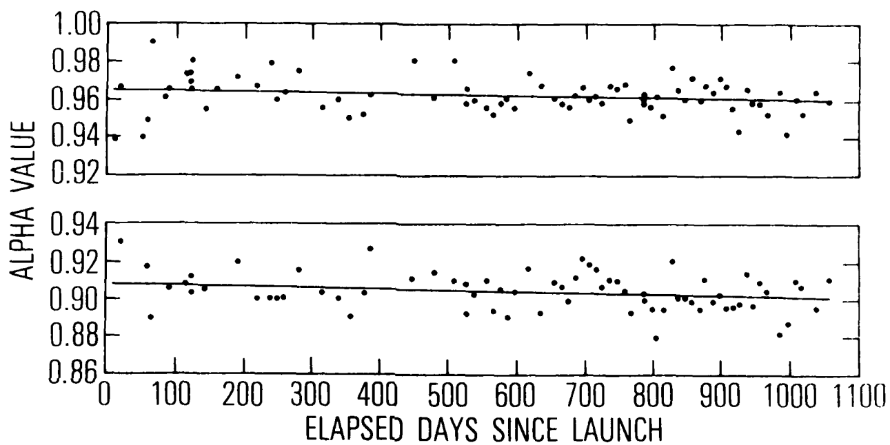
Fig. 6. Solar Absorptances of Black Paint Samples from Day of Launch
