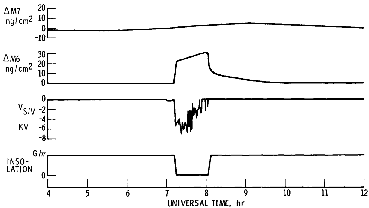
Fig. 17. ML-12 Mass Accumulation During Large P78-2 Charging in Eclipse on Day 114, 24 April 1979
