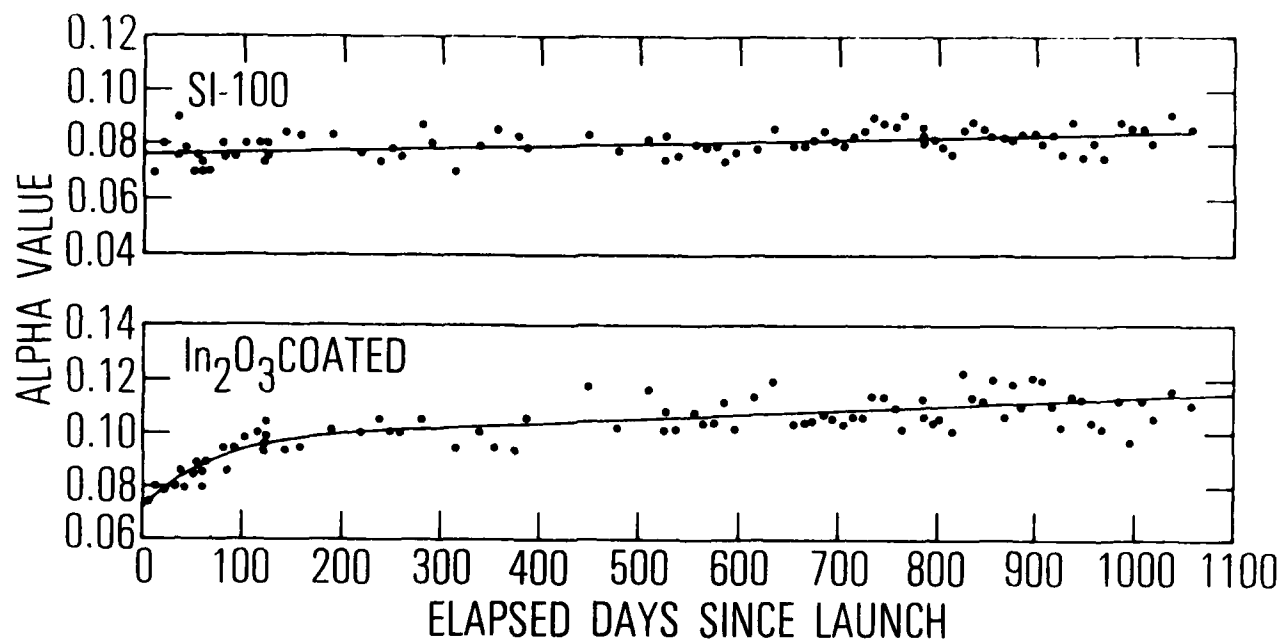
Fig. 8. Solar Absorptances of Standard and \text{In}_2\text{O}_3 -Coated Fused-Silica Mirror Samples from Day of Launch
