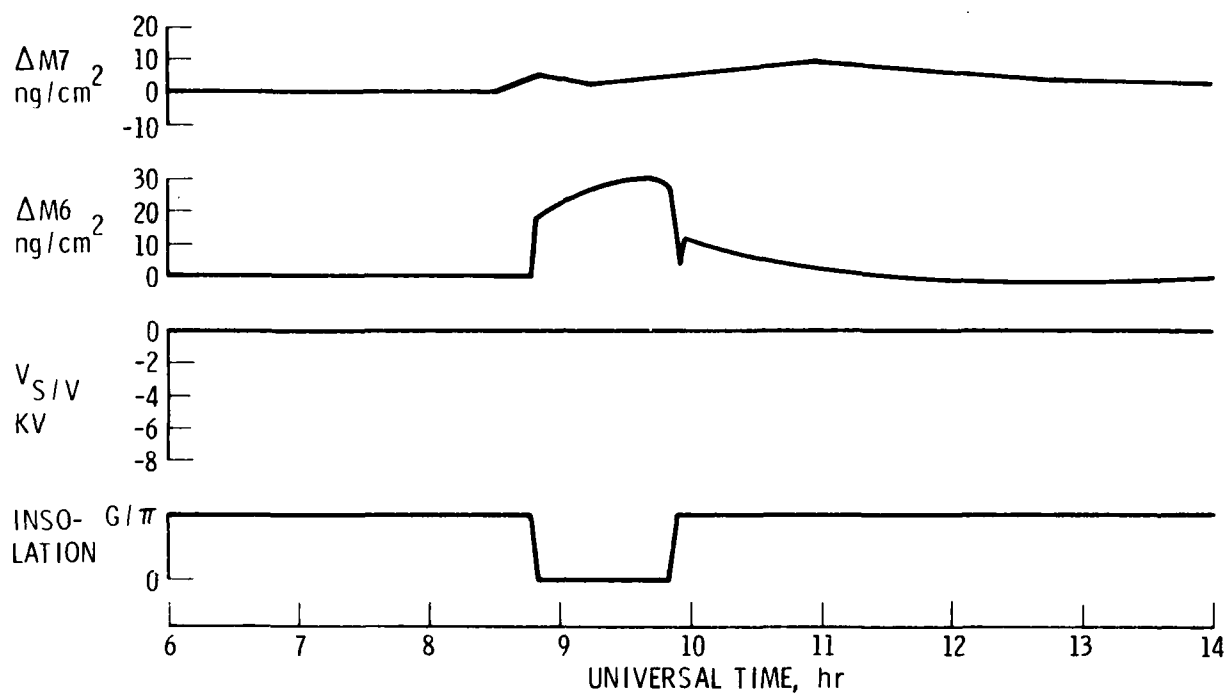
Fig. 18. ML-12 Mass Accumulation During Quiet P78-2 Eclipse on Day 109, 19 April 1979.
