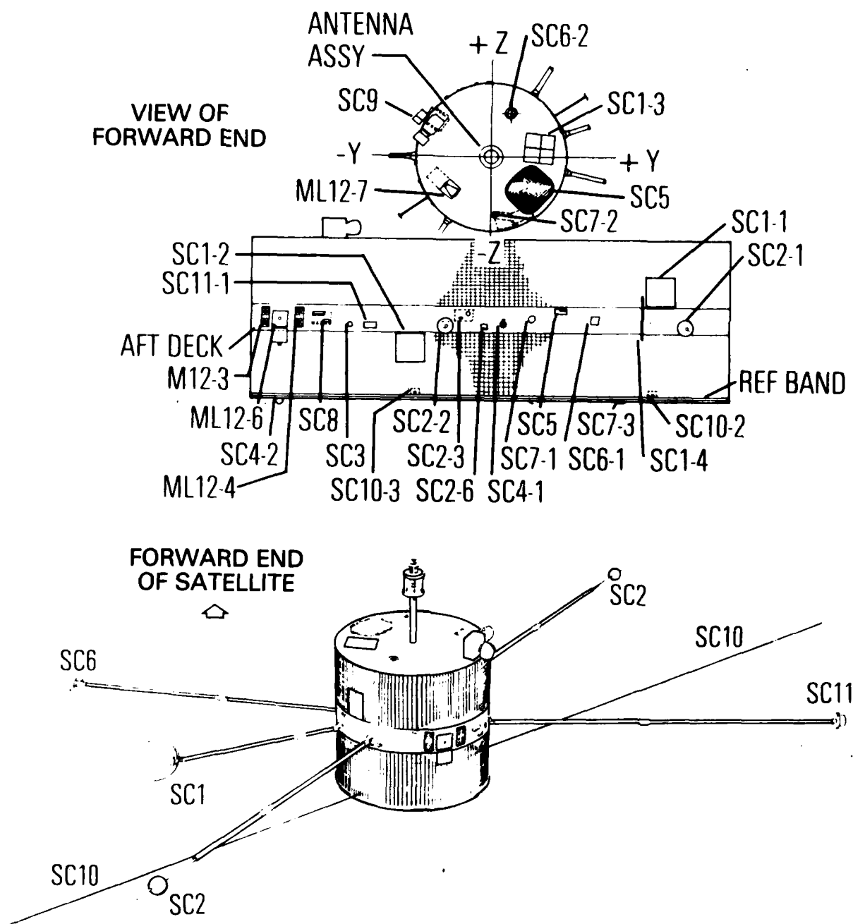
Fig. 2. P78-2 Space Vehicle
