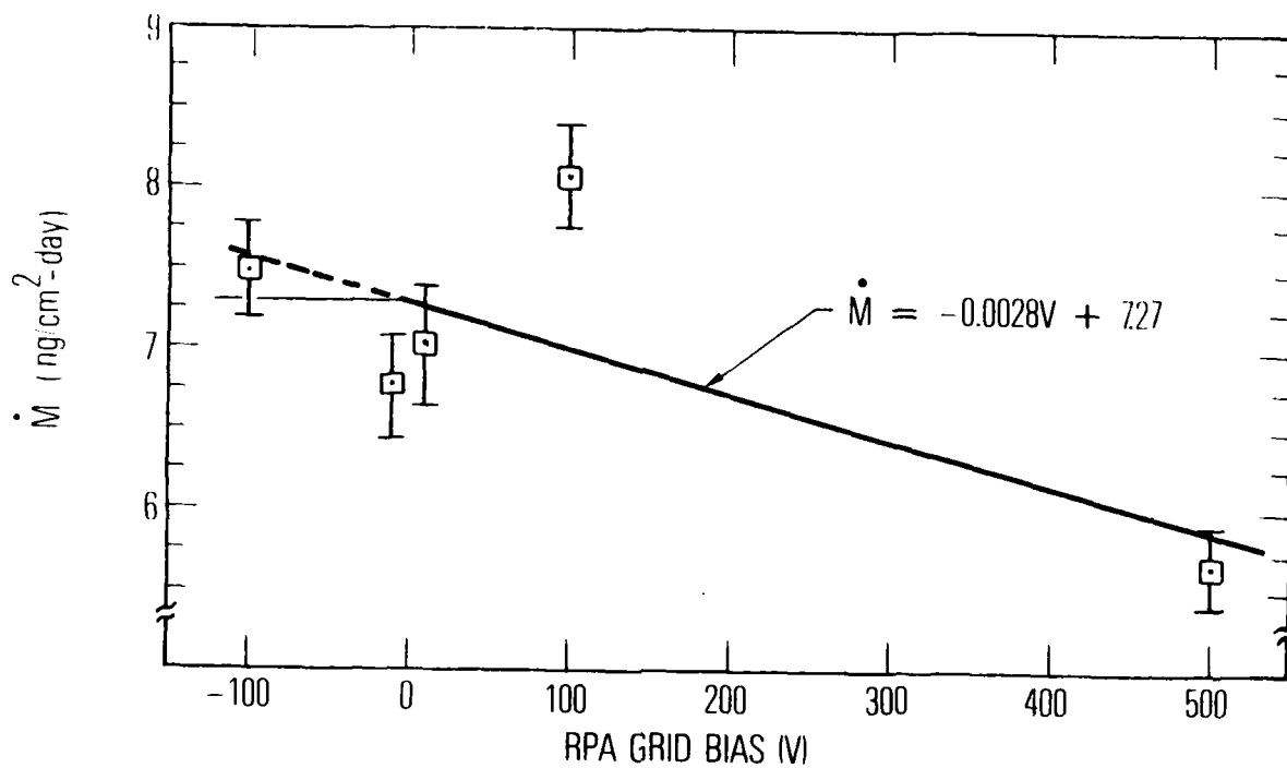
Fig. 19. ML12-6 TQCM Mass Accumulation Rates at Various RPA Grid Bias Potentials During Winter Experiment
