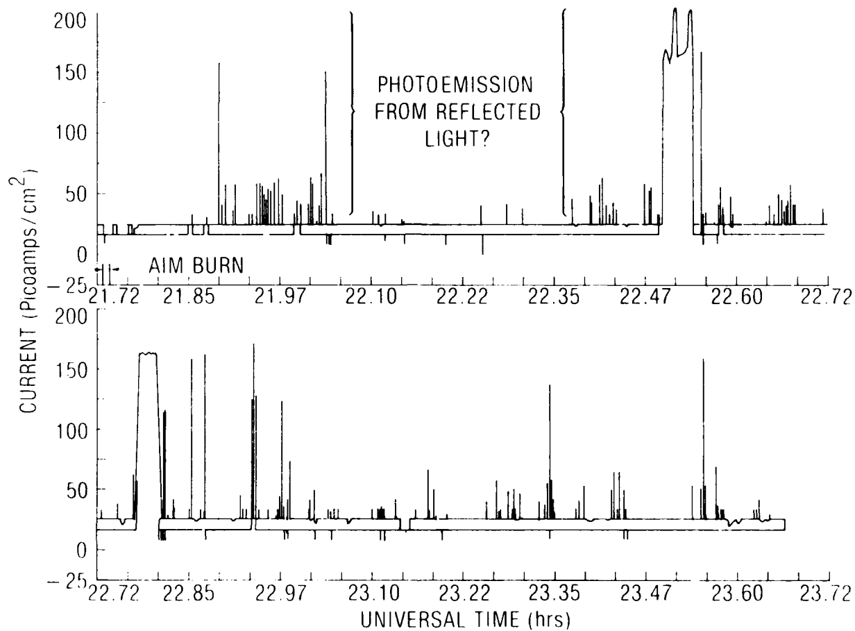
Fig. 21b. RPA Electrometer Current Density Vs. Time in the 2-Hr Period Commencing with the AIM Burn
