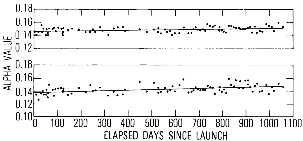
Fig. 7. Solar Absorptances of Polished Aluminum Samples from Day of Launch
