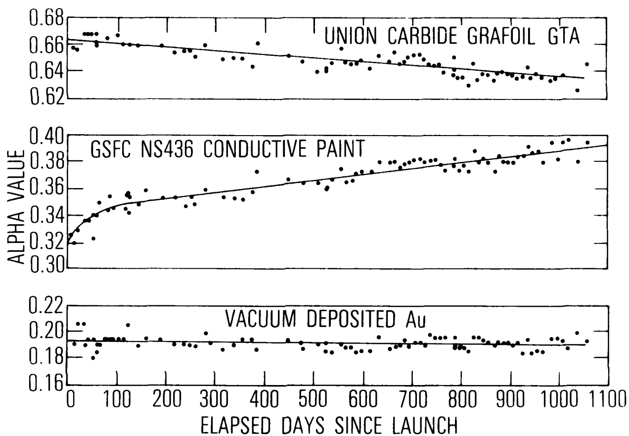
Fig. 12. Solar Absorptances of Grafoil, Conductive Yellow Paint, and Gold Samples from Day of Launch
