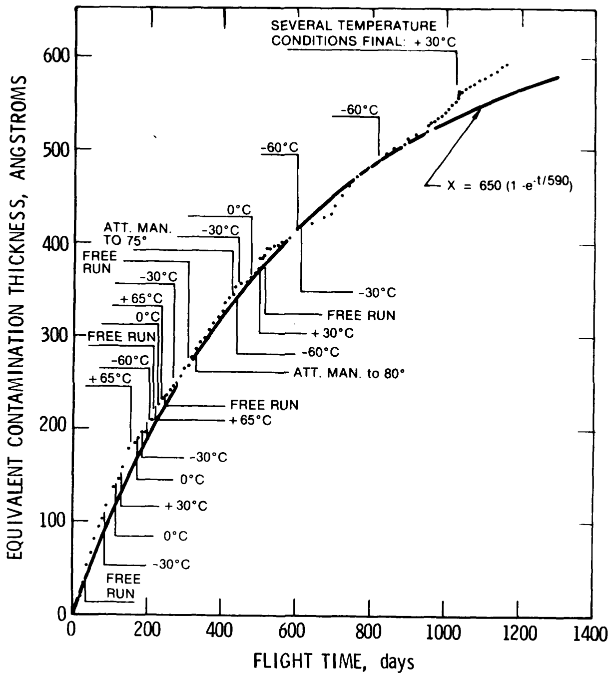
Fig. 24. Thickness of Contamination Collected on ML12-6 Temperature-Controlled Quartz-Crystal Microbalance, Assuming It Is a Uniform, Unity-Density Film. Sensor-temperature commands and curve fit are also shown.
