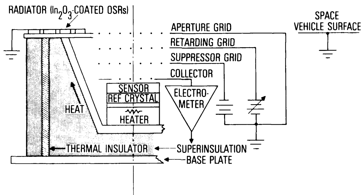
Fig. 13. Diagram of RPA/TQCMs (ML12-6 and ML12-7)
