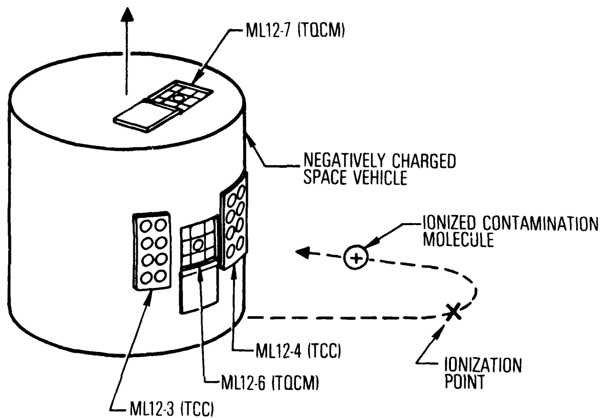
Fig. 1. Negatively Charged Vehicle Reattracting Contaminant
