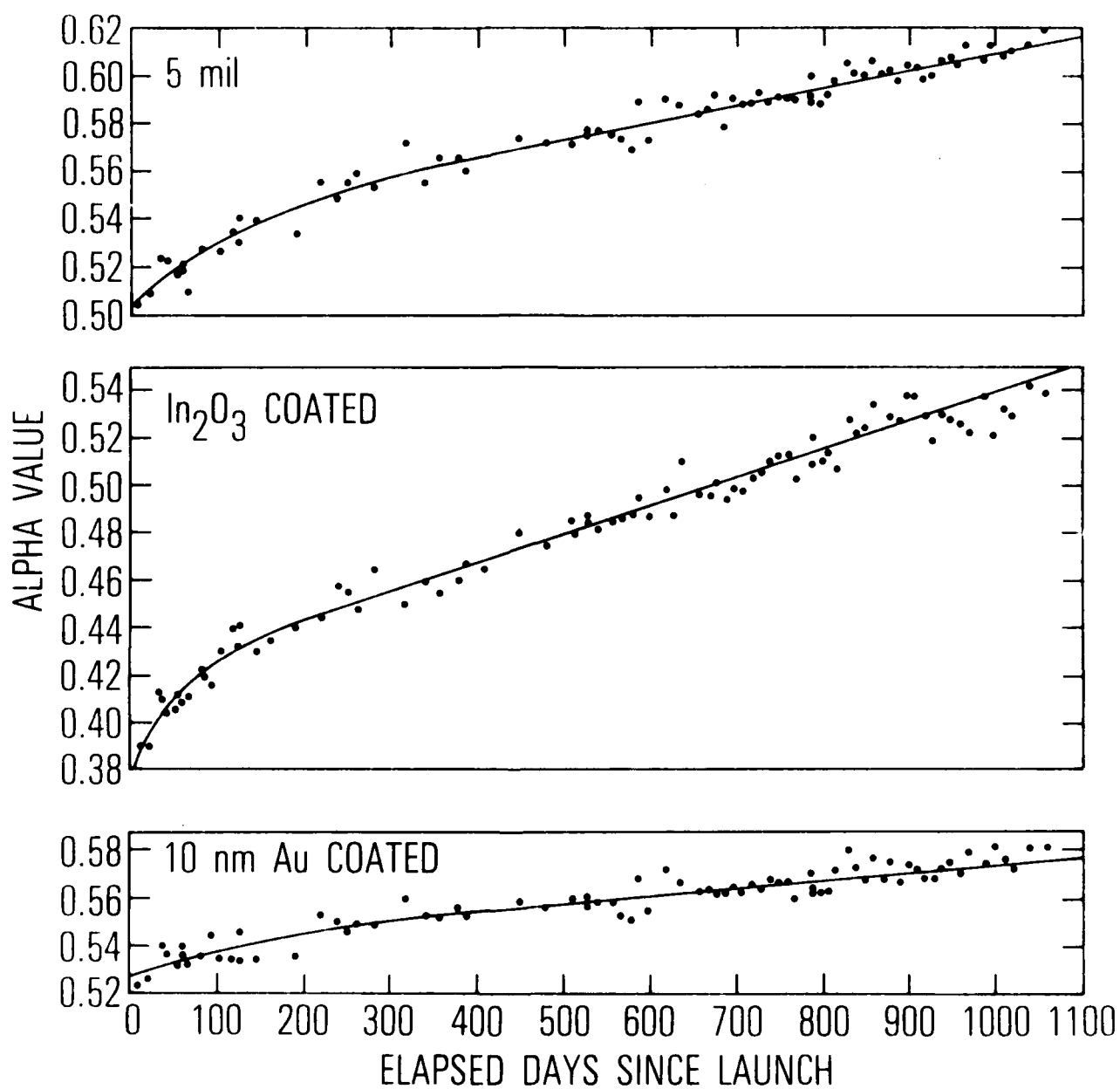
Fig. 10. Solar Absorptances of Plain, Gold-Coated, and \text{In}_2\text{O}_3 -Coated Aluminized Kapton Samples from Day of Launch
