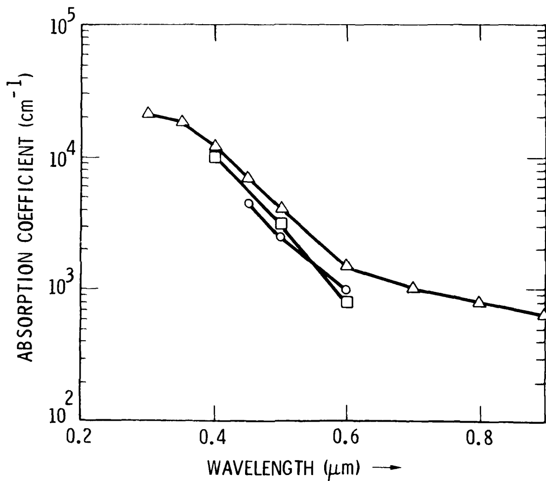
Fig. 26. Absorption Coefficient Vs. Wavelength of Irradiated Contaminants and Teflon FEP (after Champetier, Ref. 45). Curve denoted o was calculated from lab data (Ref. 46) on far-UV-irradiated simulated contamination. Curve denoted □ is data from Gemini XII flight transmission samples (Ref. 47). Curve denoted Δ was calculated from lab data (Ref. 48) on UV- and charged-particle-irradiated Teflon FEP.
