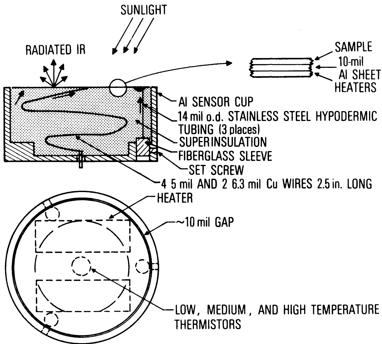
Fig. 5. Arrangement for Mounting TCC Sample Disks in Cup
