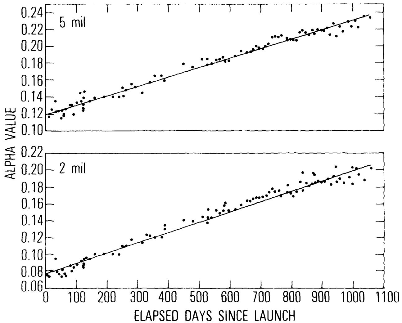
Fig. 9. Solar Absorptances of 2- and 5-Mil Thick Silvered FEP Teflon Samples from Day of Launch
