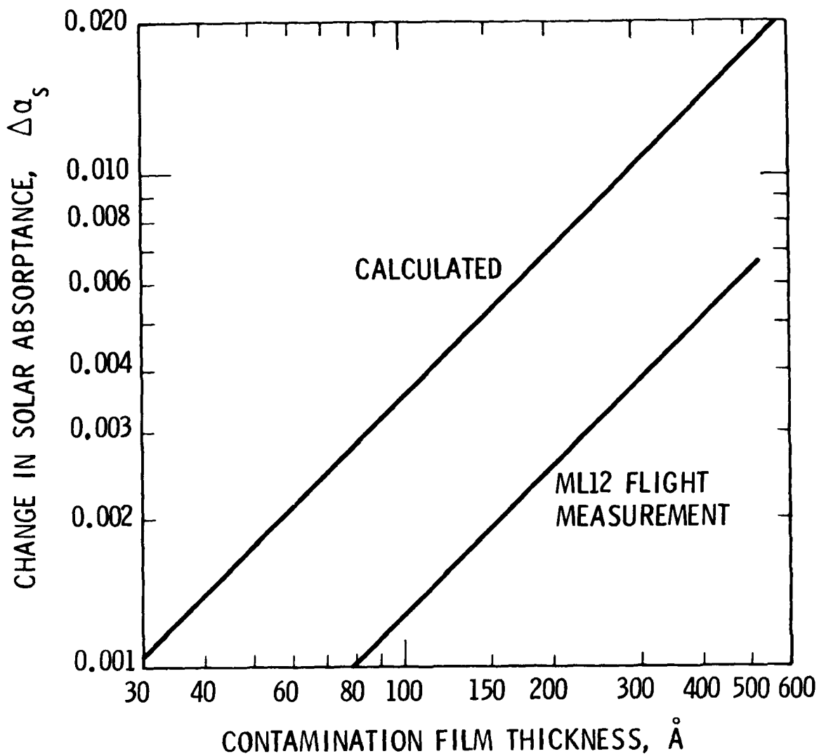
Fig. 25. Plot of Change in Solar Absorptance of Fused-Quartz Mirror (OSR) Vs. Thickness of Unity-Density Contamination Film, According to Theory (Ref. 44) and ML12 Flight Measurements
