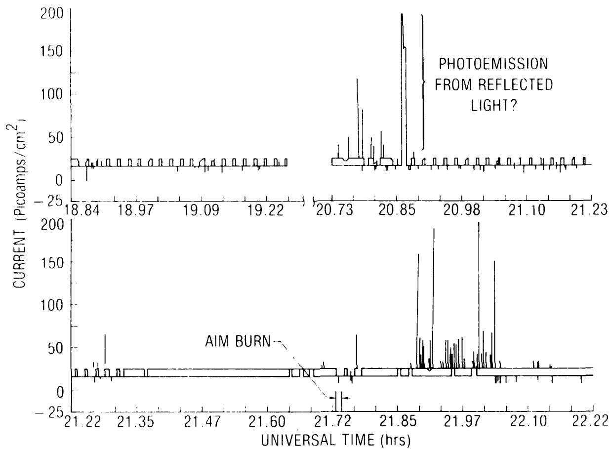
Fig. 21a. RPA Electrometer Current Density Vs. Time in the Period Preceding and Immediately Following the AIM Burn at 21.73 Hr
