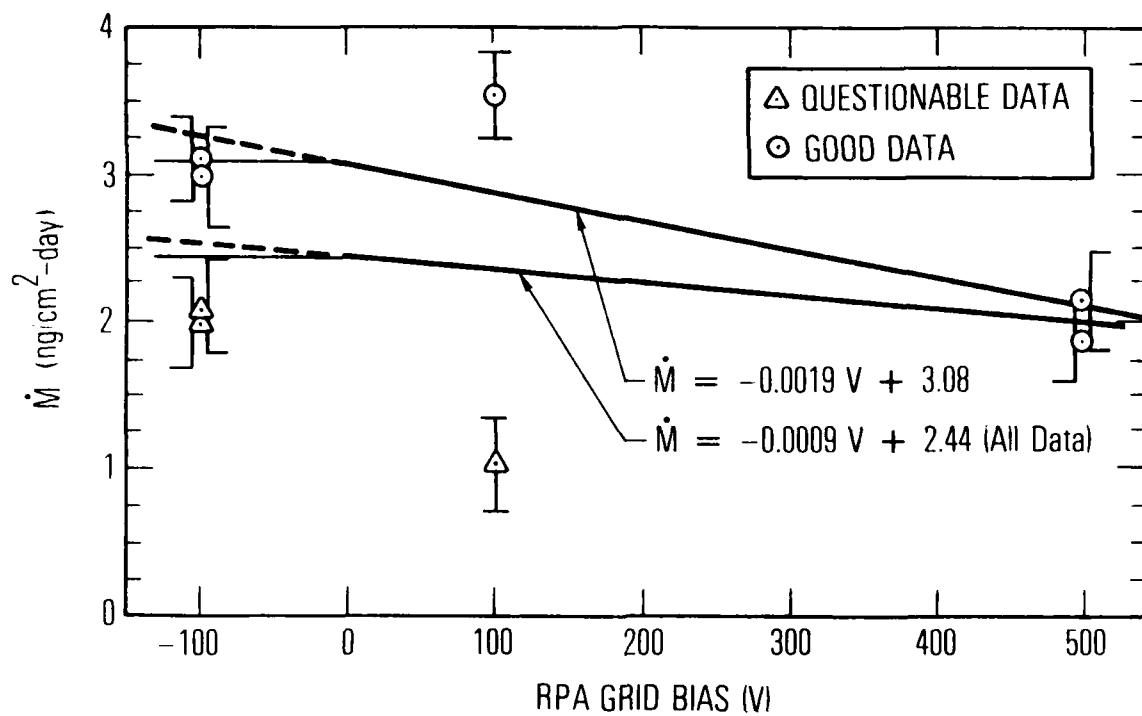
Fig. 20. ML12-6 TQCM Mass Accumulation Rates at Various RPA Grid Bias Potentials During Summer Experiment
