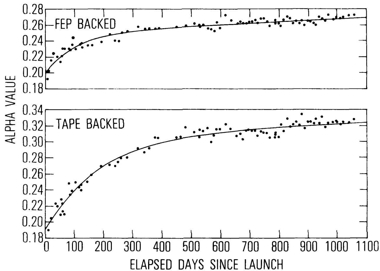
Fig. 11. Solar Absorptances of Astroquartz Fabric Samples Backed with Silvered-FEP Teflon and Double Adhesive Tape, Respectively, from Day of Launch (Day 30)
