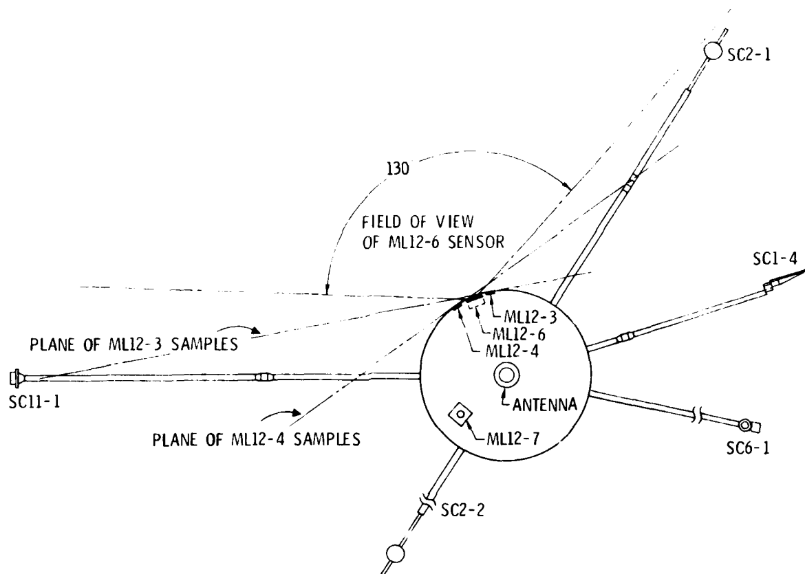
Fig. 23. Scale Drawing of P78-2 Viewed Along Vehicle Spin Axis Showing that ML12-3, -4, and -6 Sensors Have Nearly Free Fields of View
