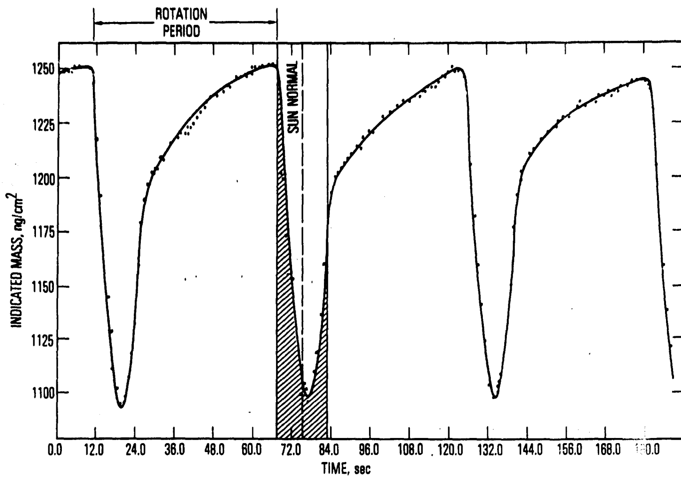
Fig. 16. ML12-6 Indicated Mass During Operations on Day 114 (24 April 1979)
