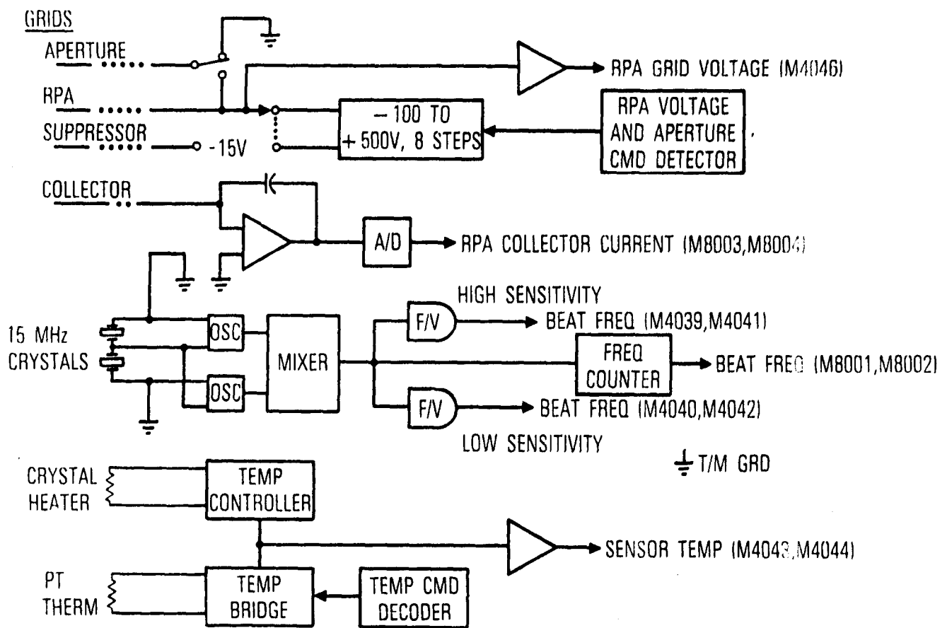
Fig. 15. RPA/TQCM Block Diagram
