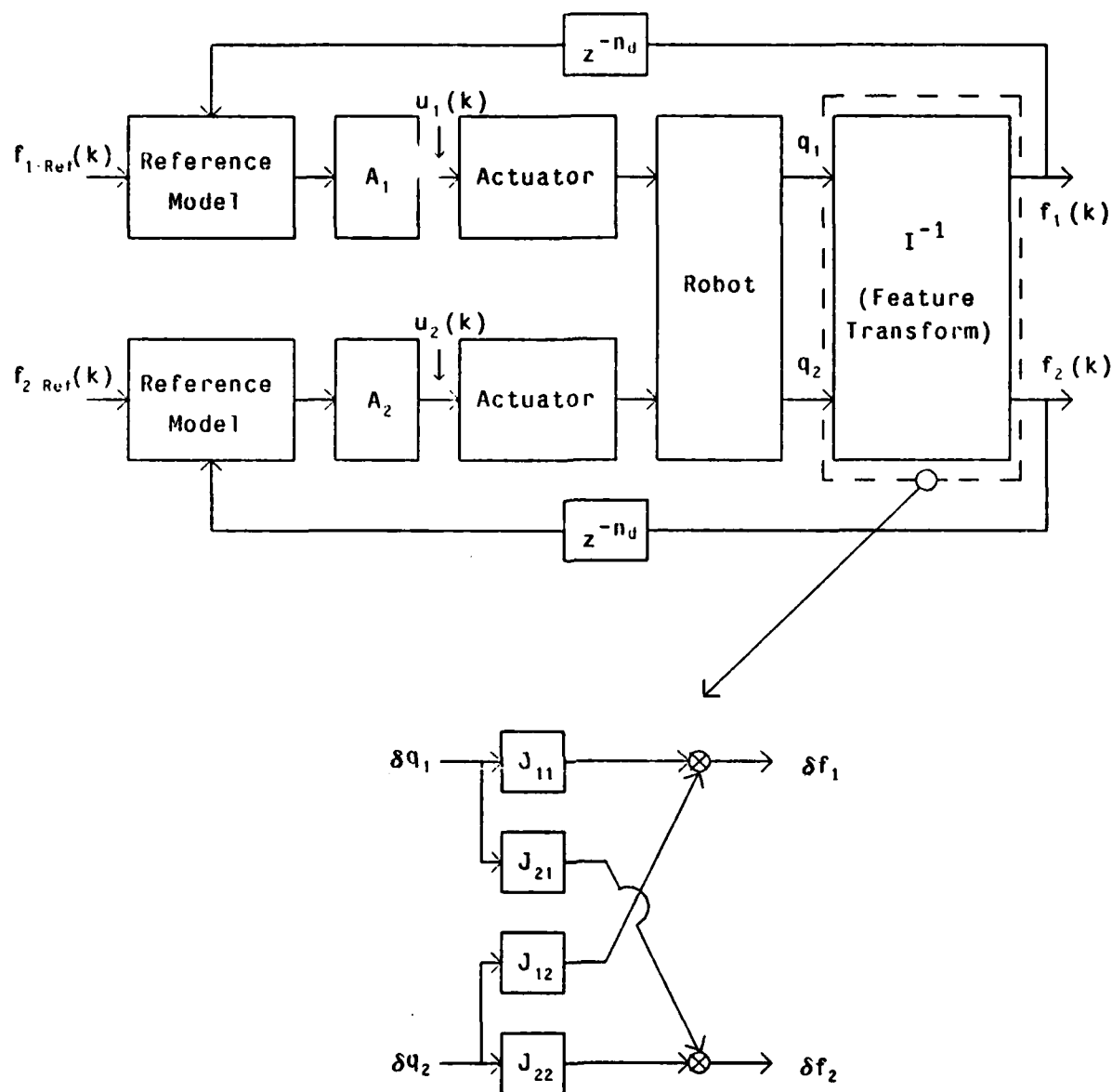
Figure 2-16: MRAC Control of an IBVS System
