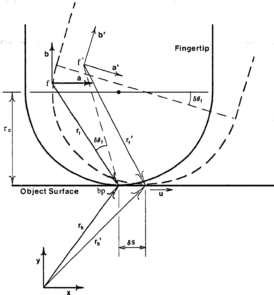
Figure 4-3: Cross section of a large-radius hemispherical fingertip on a flat object surface
