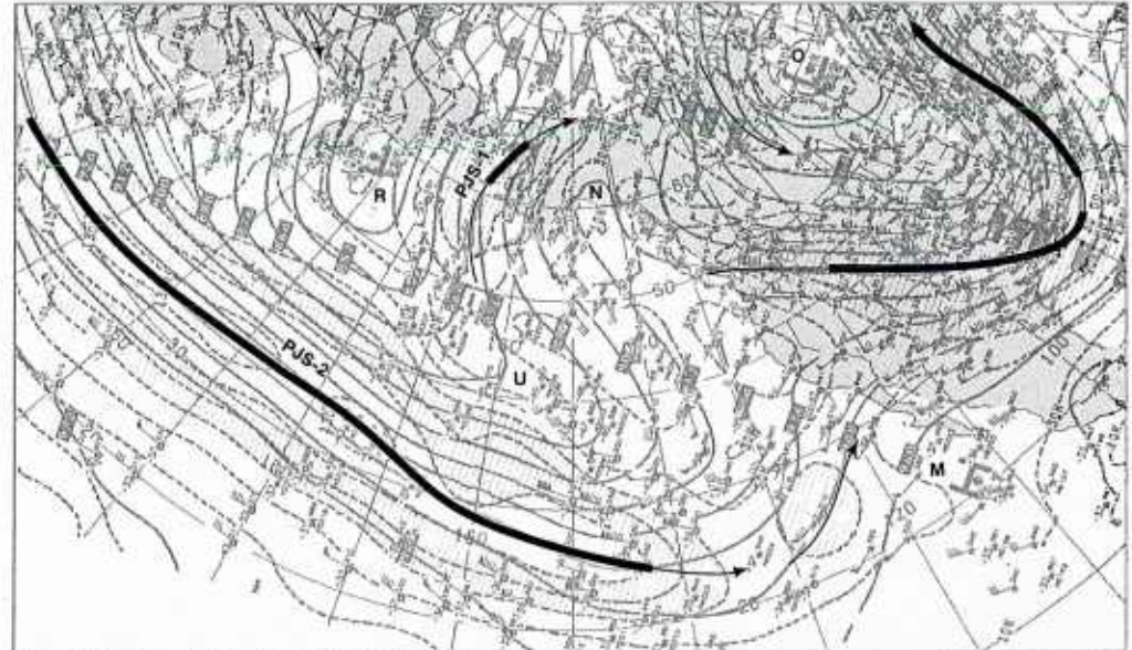
1B-34a. NMC 300-mb Analysis. 0000 GMT 3 January 1979.
