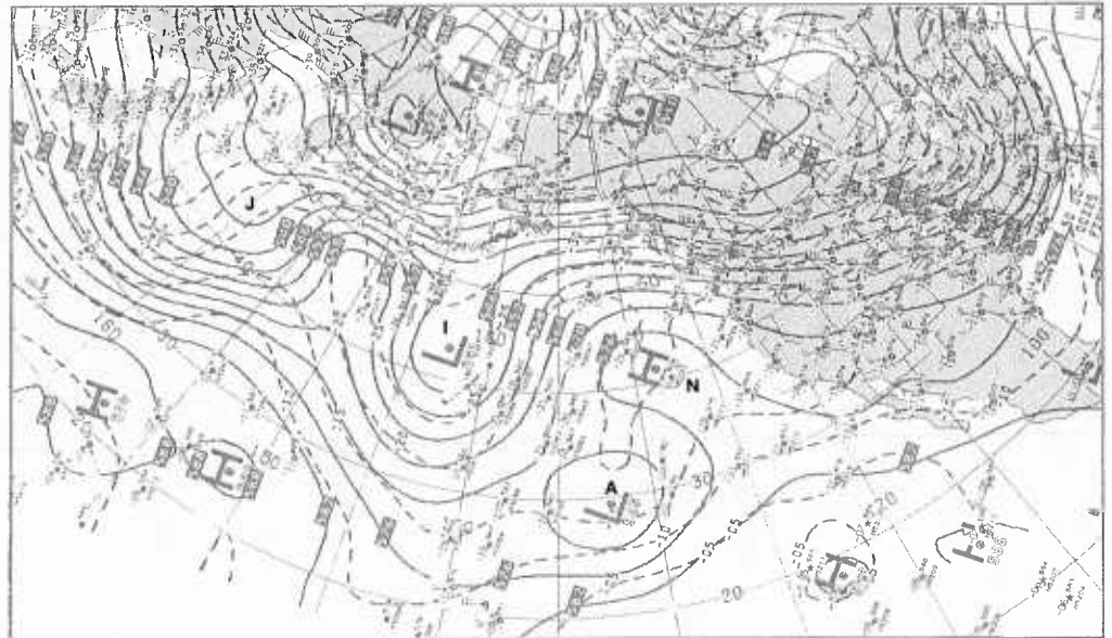
1B-10b. NMC 500-mb Analysis. 0000 GMT 25 December 1978.
