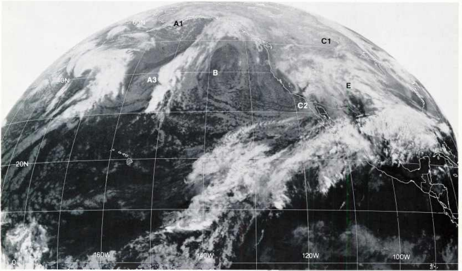
1B-70a. GOES-W. Infrared Picture. 1815 GMT 25 January 1979.
