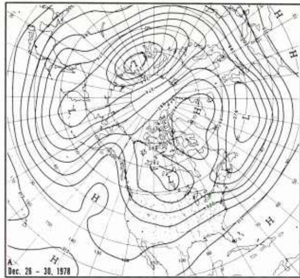
1B-28b. Mean 700-mb Contours for 26-30 December 1978. (After Taubensee, 1979.)
