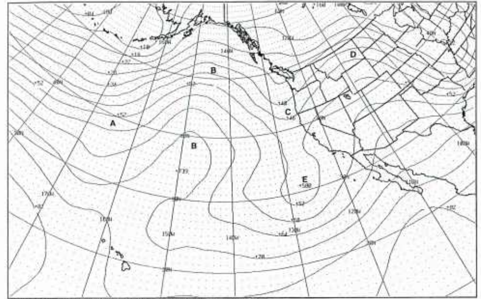
IB-65c. FNOC PE Initial 500-mb Analysis, 1200 GMT 24 January 1979.
