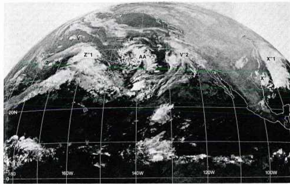
1B-47c. GOES-W. Infrared Picture. 1215 GMT 7 January 1979.
