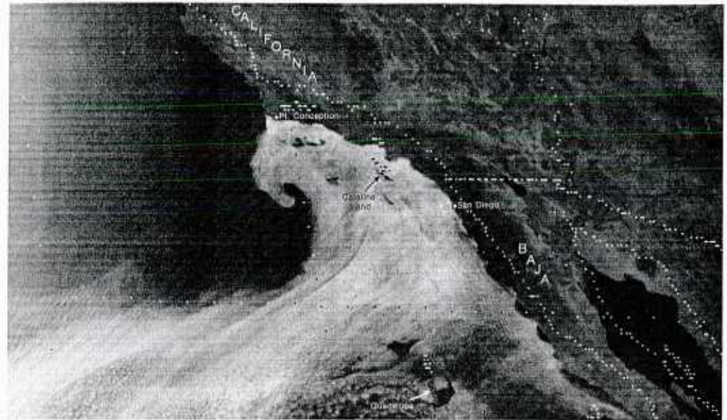
3B-10a. GOES-W. Visible Picture. 1915 GMT 29 August 1977.
