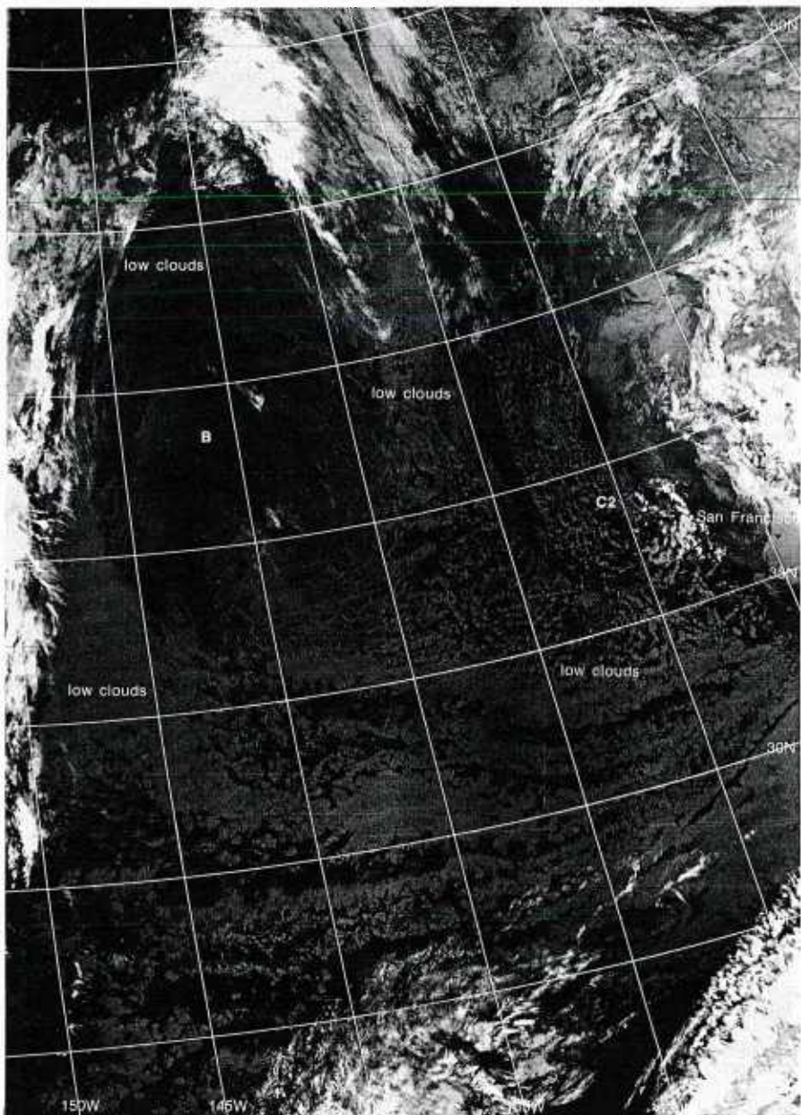
IB-69a. F-1. DMSF TF T-Expand Enhancement. 0847 GMT 25 January 1979.
