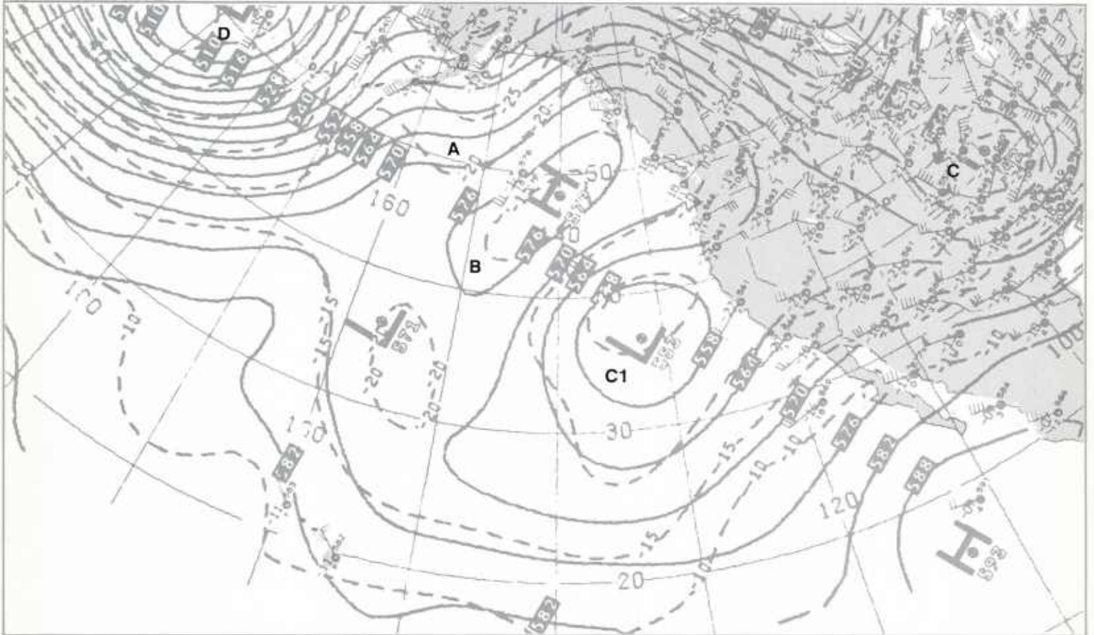
1B-80b. NMC 500-mb Analysis. 1200 GMT 23 March 1979.
