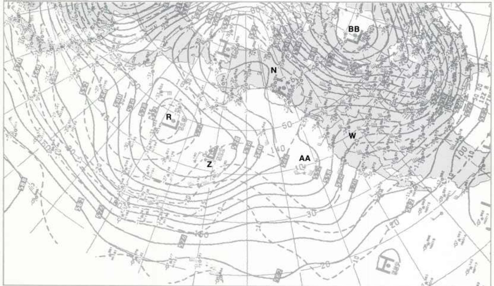
1B-49b. NMC 500-mb Analysis. 1200 GMT 8 January 1979.
