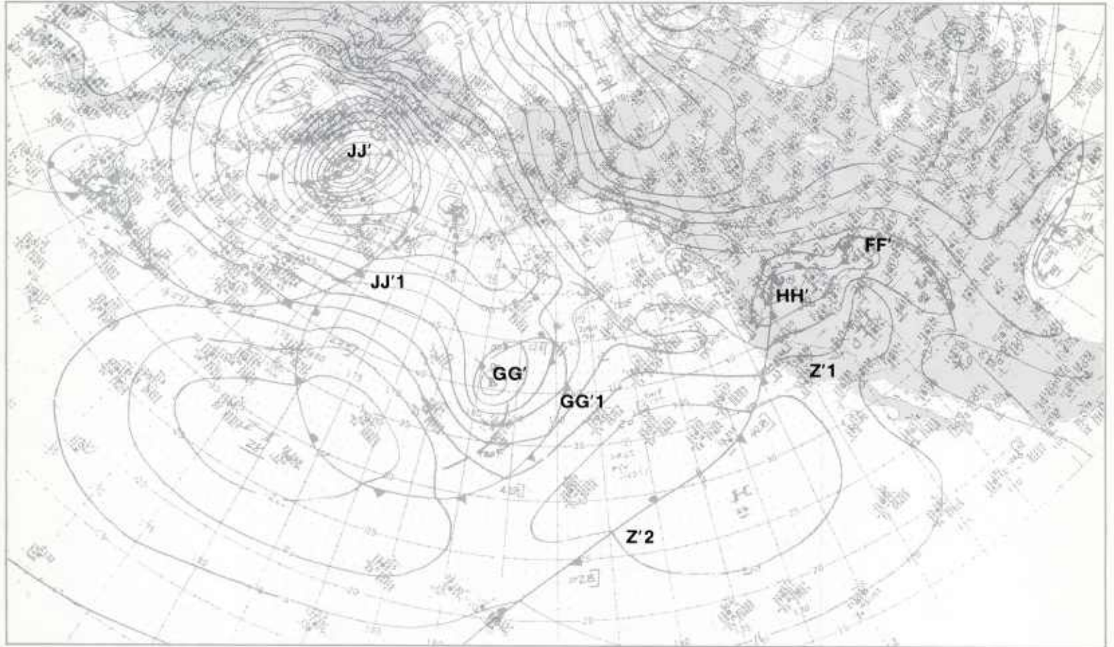
1B-59b. NMC Surface Analysis. 0000 GMT 12 January 1979.
