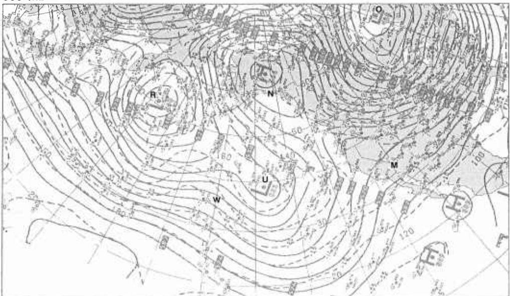
IB-39b. NMC 500-mb Analysis. 0000 GMT 4 January 1979.
