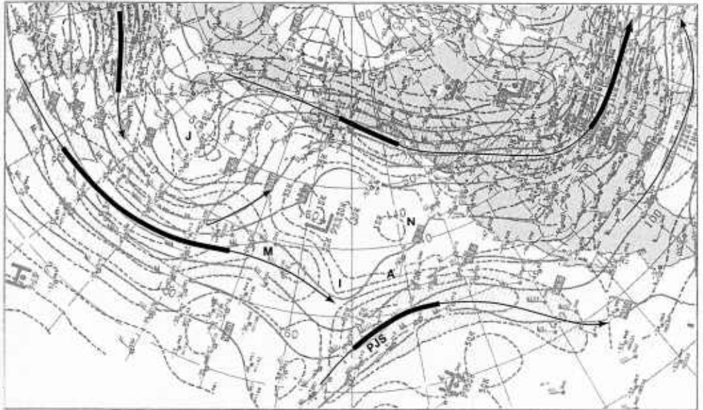
1B-14a. NMC 300-mb Analysis. 1200 GMT 26 December 1978.
