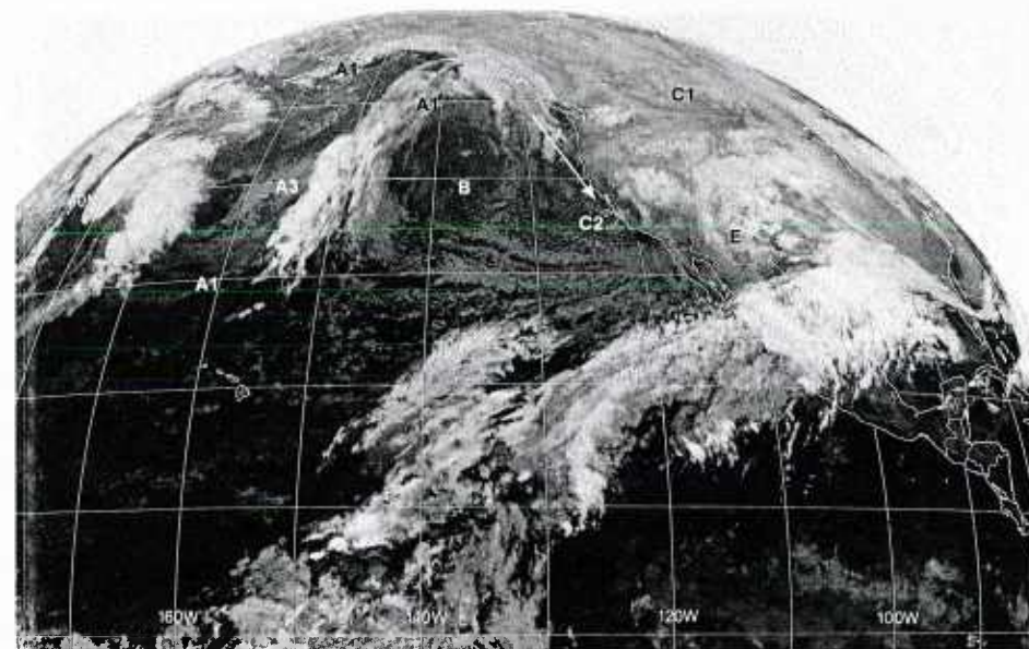
IB-69b. GOES-W. Infrared Picture. 1215 GMT 25 January 1979.
