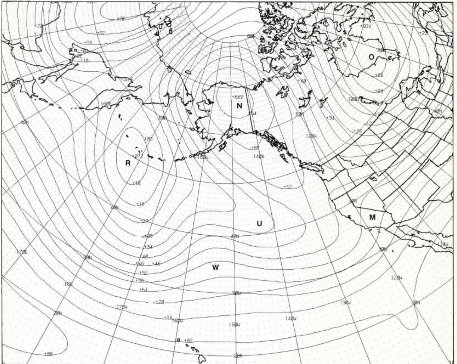
1B-36a. FNOC PE 36-hr 500-mb Prognosis. Valid 1200 GMT 4 January 1979.
