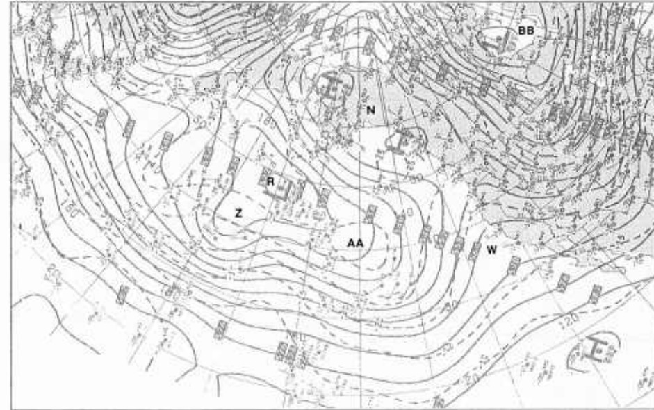
1B-47d. NMC 500-mb Analysis. 1200 GMT 7 January 1979.
