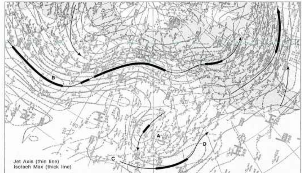
1B-2a. NMC 300-mb Analysis. 0000 GMT 22 December 1978.
