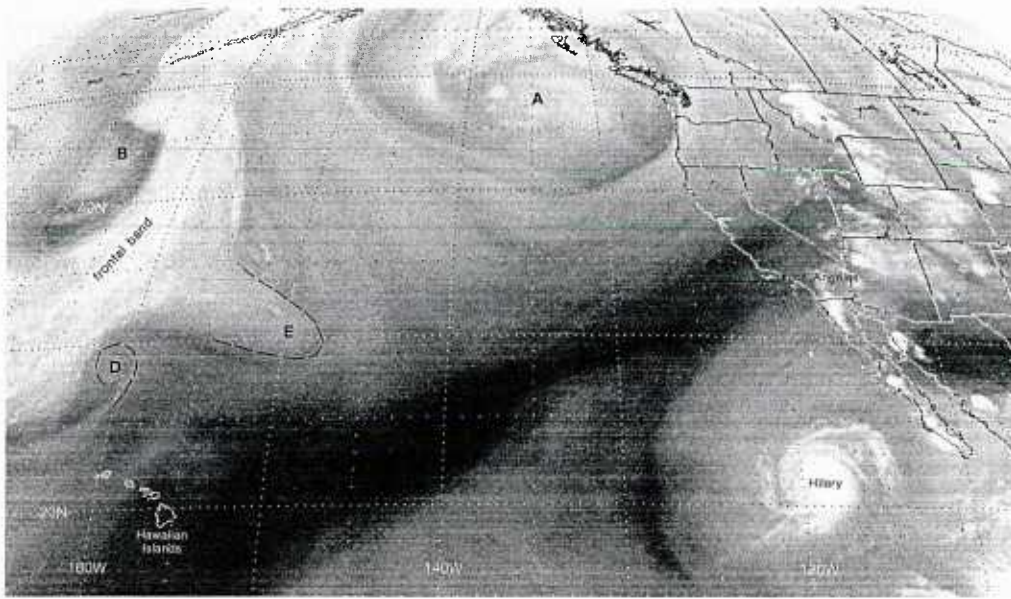
2B-27a. GOES-W. Water Vapor Picture. 0015 GMT 26 August 1981.
