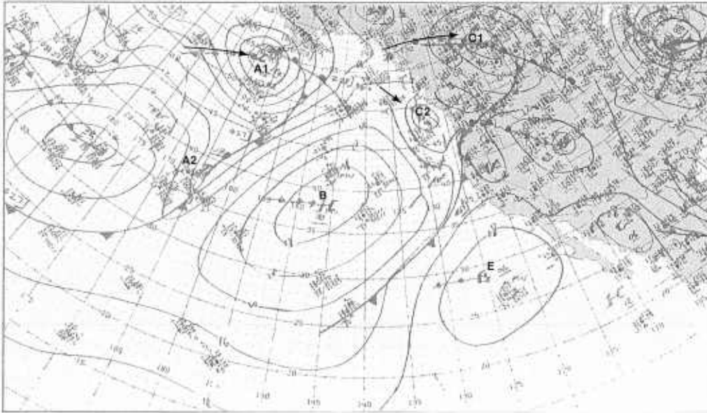
IB-65b. NMC Surface Analysis, 1200 GMT 24 January 1979.
