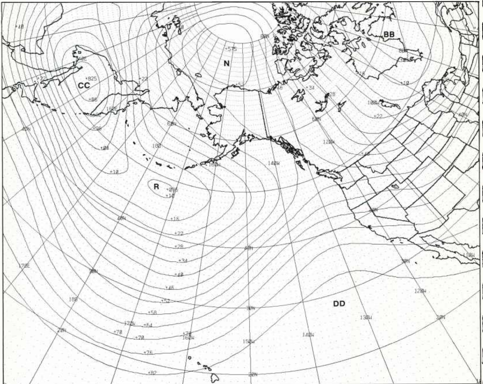
1B-52a. FNOC PE 36-hr 500-mb Prognosis. Valid 1200 GMT 10 January 1979.
