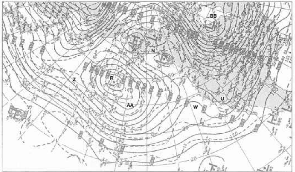
1B-46b. NMC 500-mb Analysis. 1200 GMT 6 January 1979.
