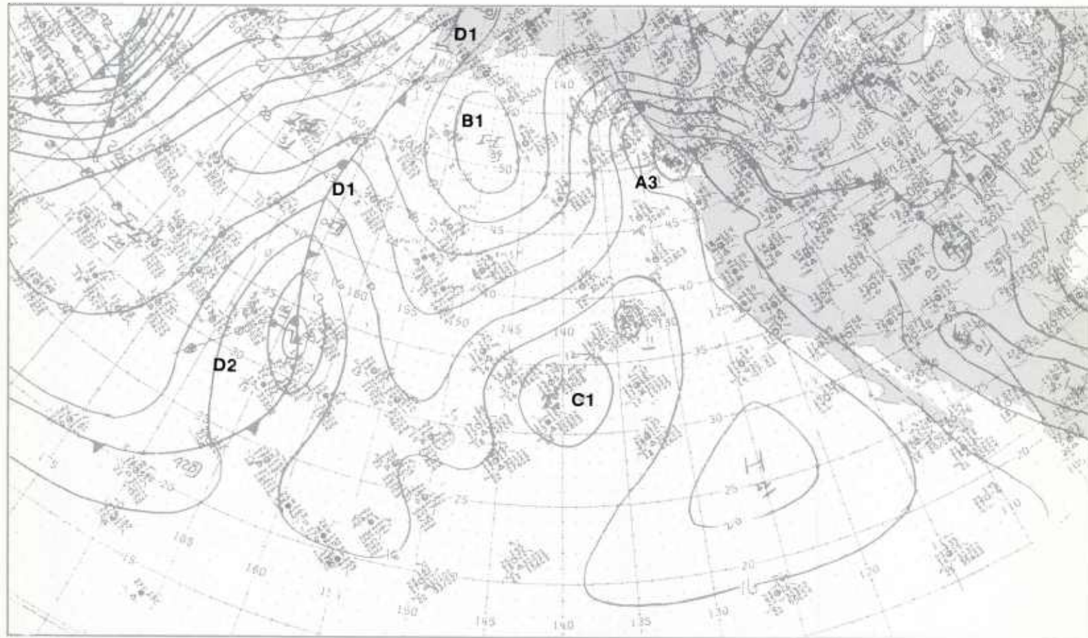
1B-85b. NMC Surface Analysis. 0000 GMT 26 March 1979.
