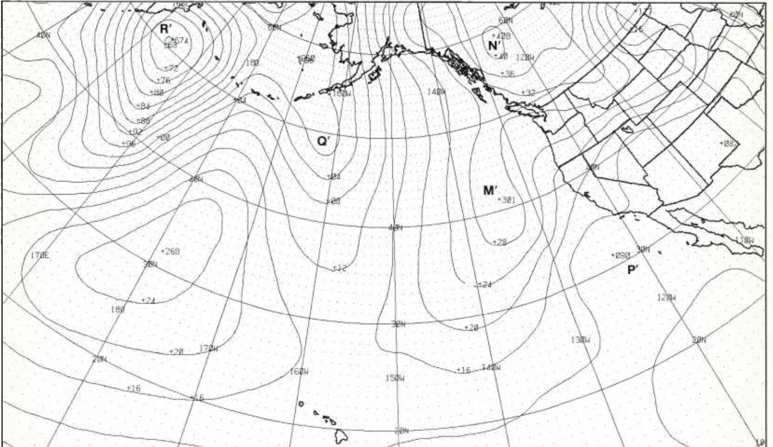
1B-24b. FNOC PE Initial Surface Analysis. 1200 GMT 29 December 1978.
