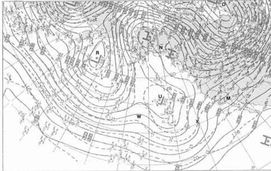
IB-39d. NMC 500-mb Analysis. 1200 GMT 4 January 1979.
