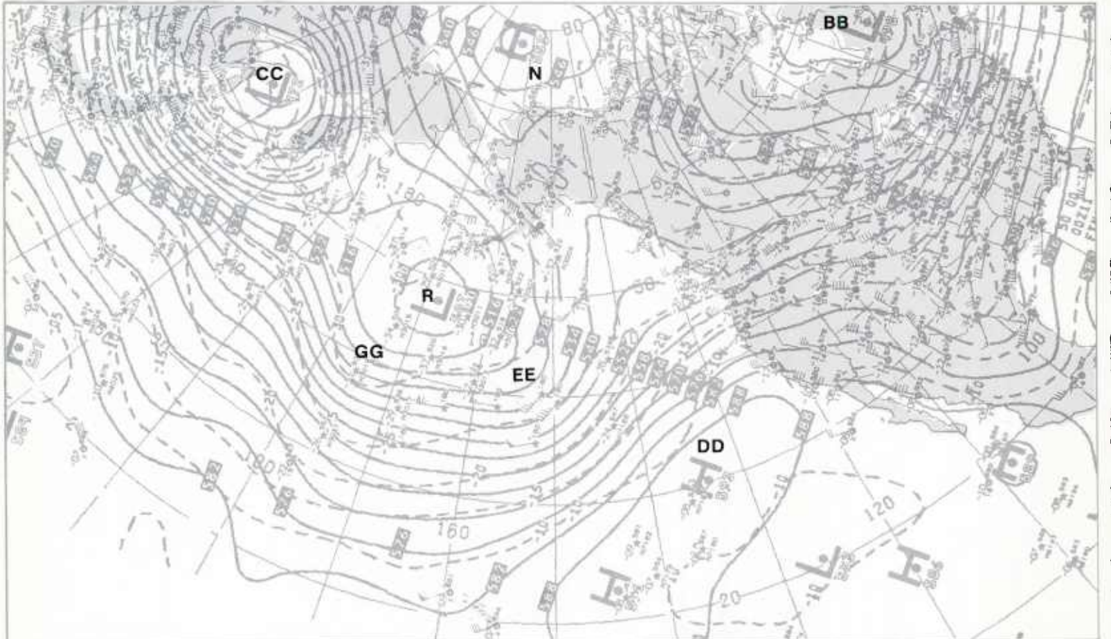
1B-56b. NMC 500-mb Analysis. 0000 GMT 11 January 1979.
