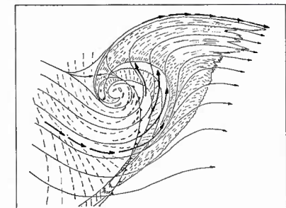
2A-3d. Type B Mature Storm Cloud Pattern with 300-mb Streamlines, Jet Axis and Surface Front.
