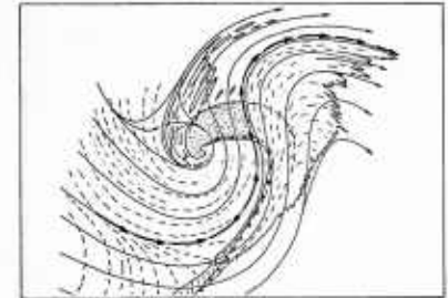
2A-3b. Type A Mature Storm Cloud Pattern with 300-mb Streamlines, Jet Axis and Surface Front.
