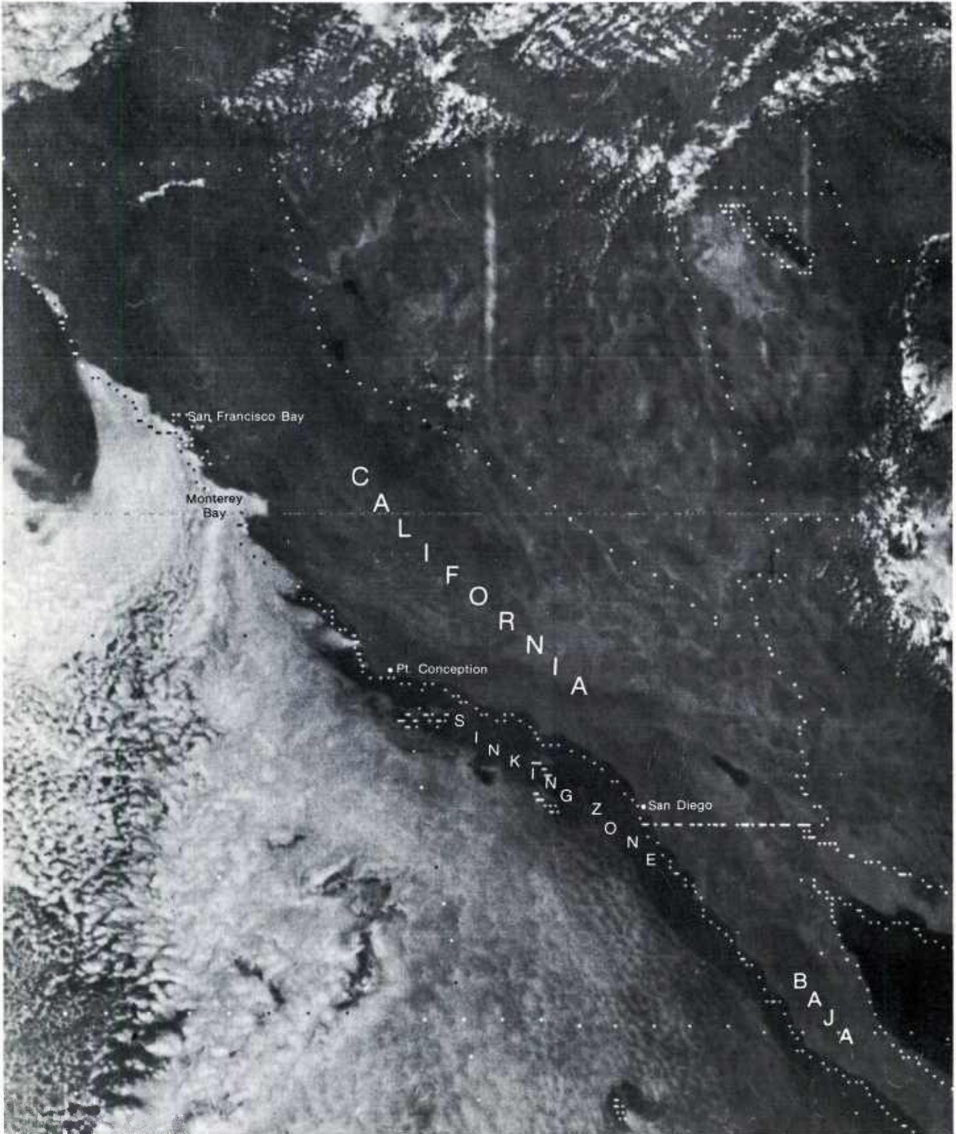
3B-5a. GOES-W. Visible Picture. 2315 GMT 12 July 1977. Offshore Sinking Zone Associated with Sea Breeze Circulation.
