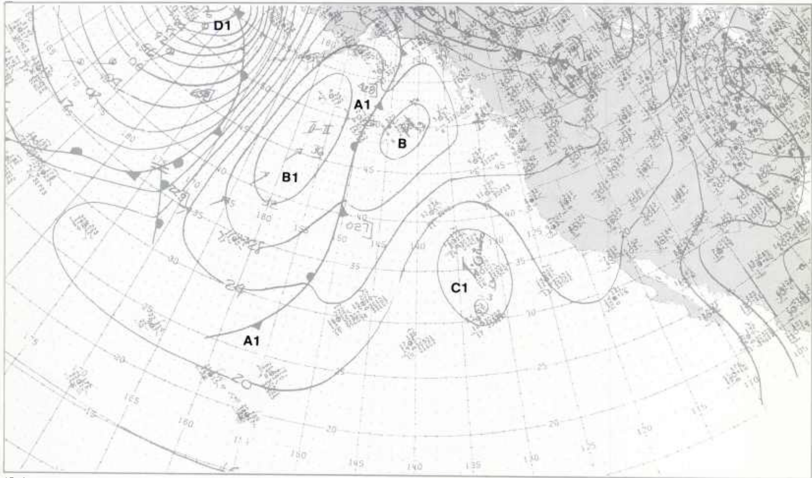
IB-81b. NMC Surface Analysis. 1200 GMT 23 March 1979.
