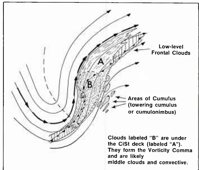
2A-6b. Meridional Trough Cyclogenesis, Phase 2.
