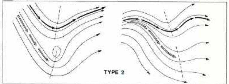
2A-16b. Typical flow patterns for Split Flow Cyclogenesis.
