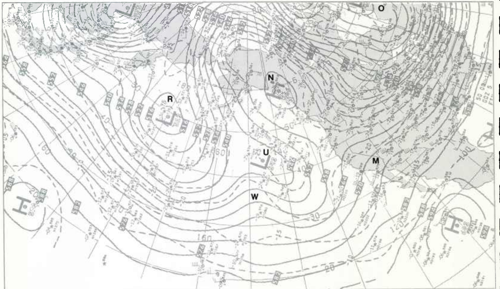
1B-40b. NMC 500-mb Analysis. 0000 GMT 5 January 1979.
