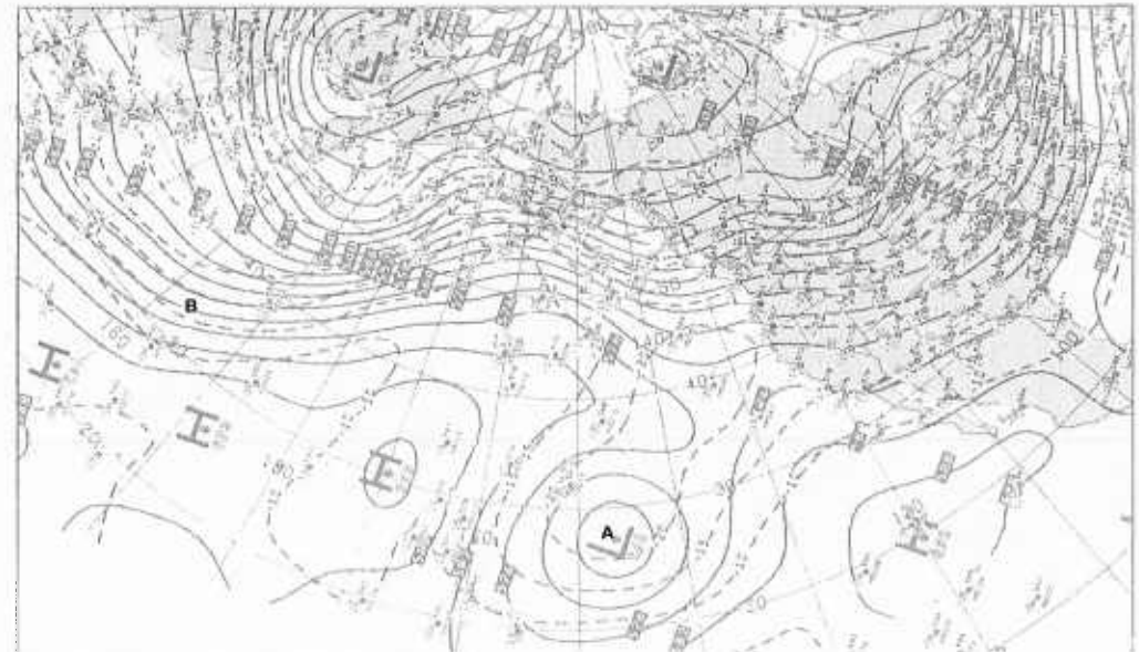
1B-2b. NMC 500-mb Analysis. 0000 GMT 22 December 1978.
