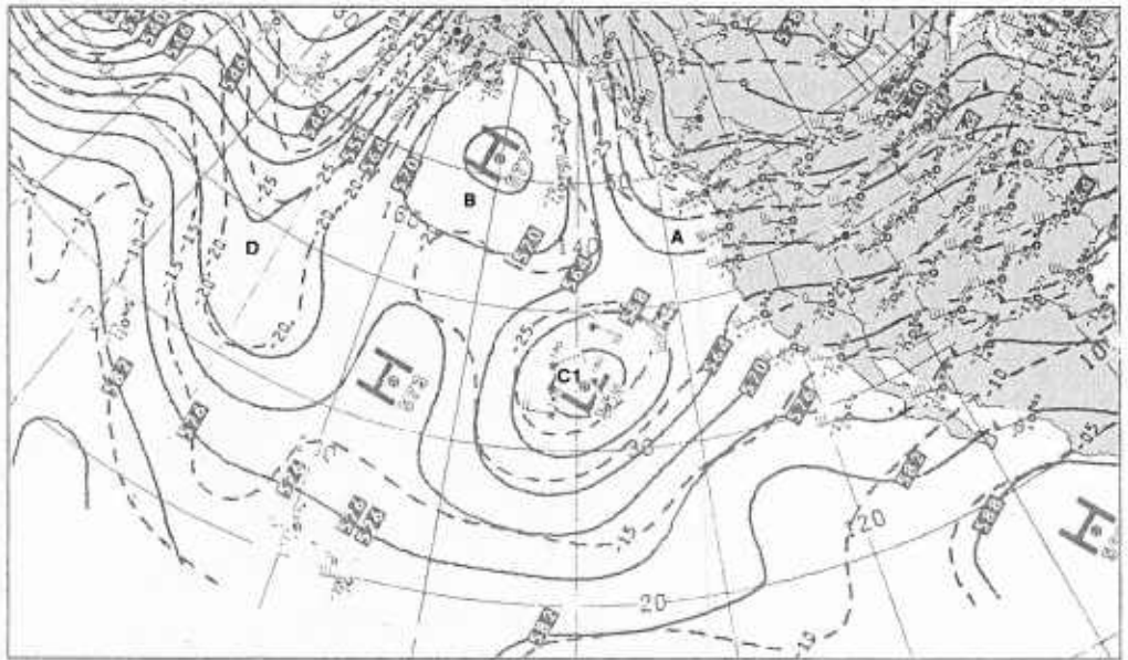
1B-84b. NMC 500-mb Analysis. 0000 GMT 26 March 1979.
