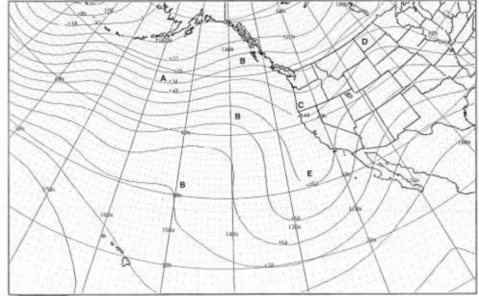
1B-63d. FNOC PE 36-hr 500-mb Prognosis. Valid 1200 GMT 25 January 1979.
