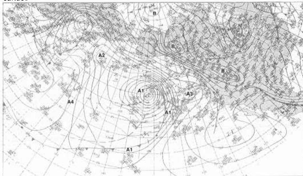
2B-3b. NMC Surface Analysis. 0000 GMT 9 January 1979.
