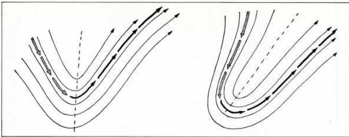
2A-5a. Typical flow patterns for Meridional Trough Cyclogenesis.
