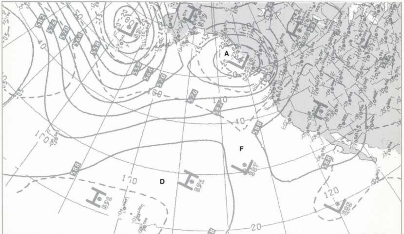
2B-32b. NMC 500-mb Analysis. 1200 GMT 27 August 1981.
