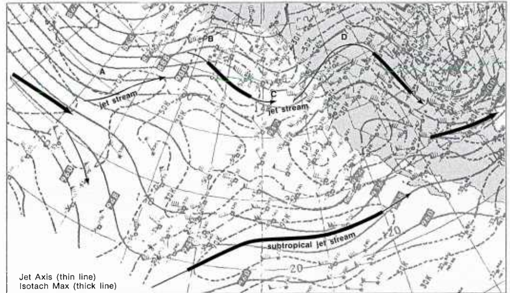
1B-62a. NMC 300-mb Analysis. 0000 GMT 24 January 1979.
