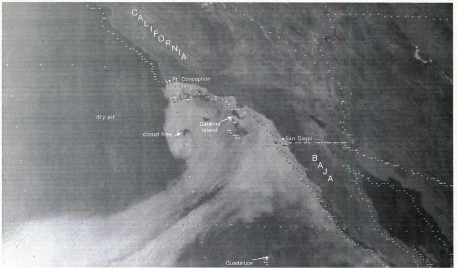
3B-12a. GOES-W. Visible Picture. 2245 GMT 29 August 1977.
