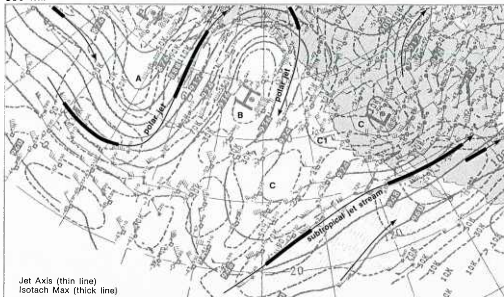
IB-74a. NMC 300-mb Analysis. 0000 GMT 22 March 1979.
