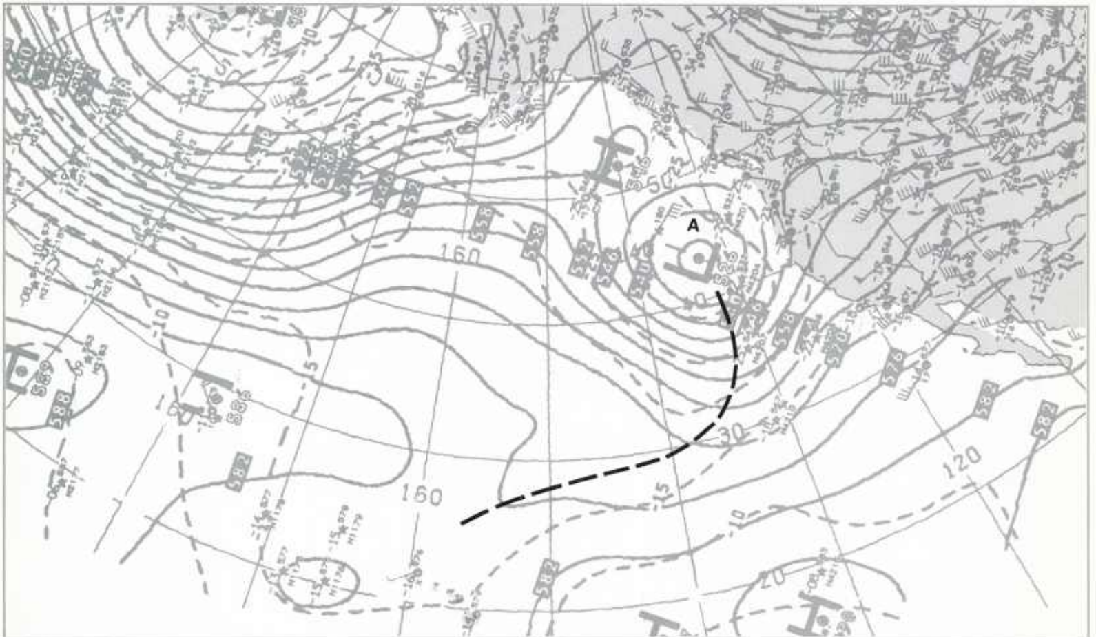
2B-20b. NMC 500-mb Analysis. 1200 GMT 14 January 1979.
