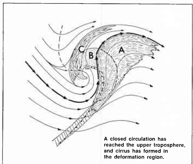
2A-6d. Meridional Trough Cyclogenesis, Phase 4.
