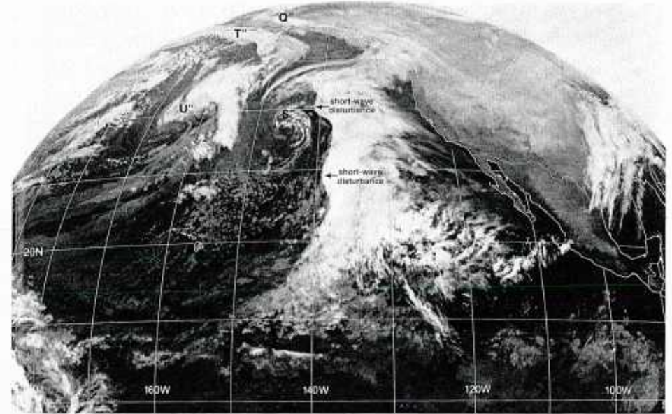
1B-31c. GOES-W. Infrared Picture. 1215 GMT 1 January 1979.
