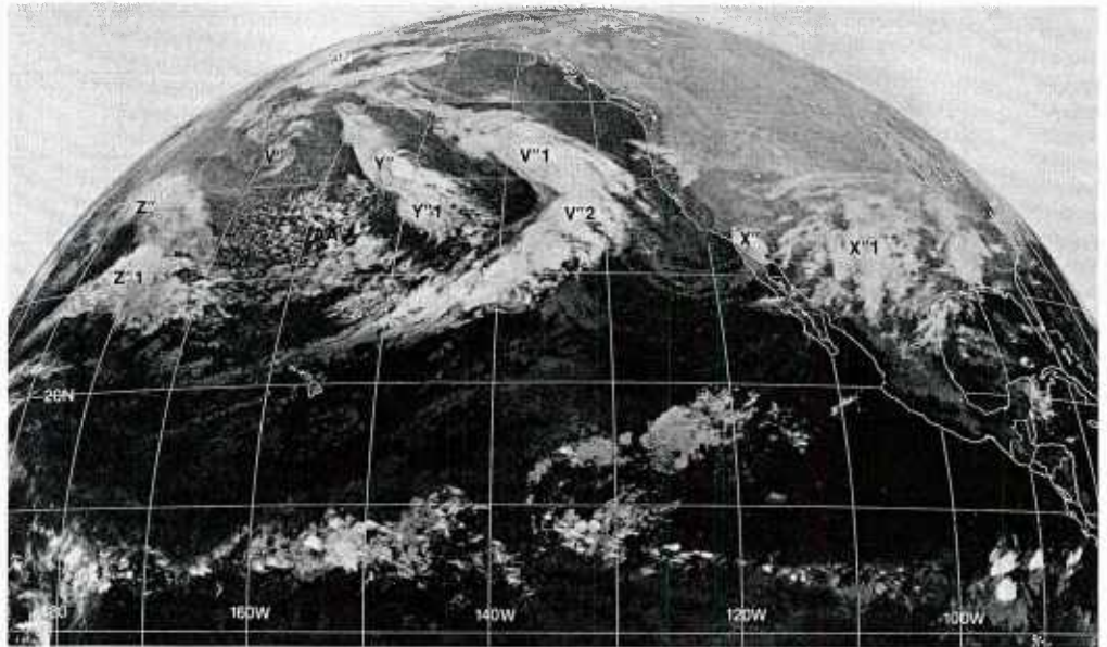
1B-46a. GOES-W. Infrared Picture. 1215 GMT 6 January 1979.
