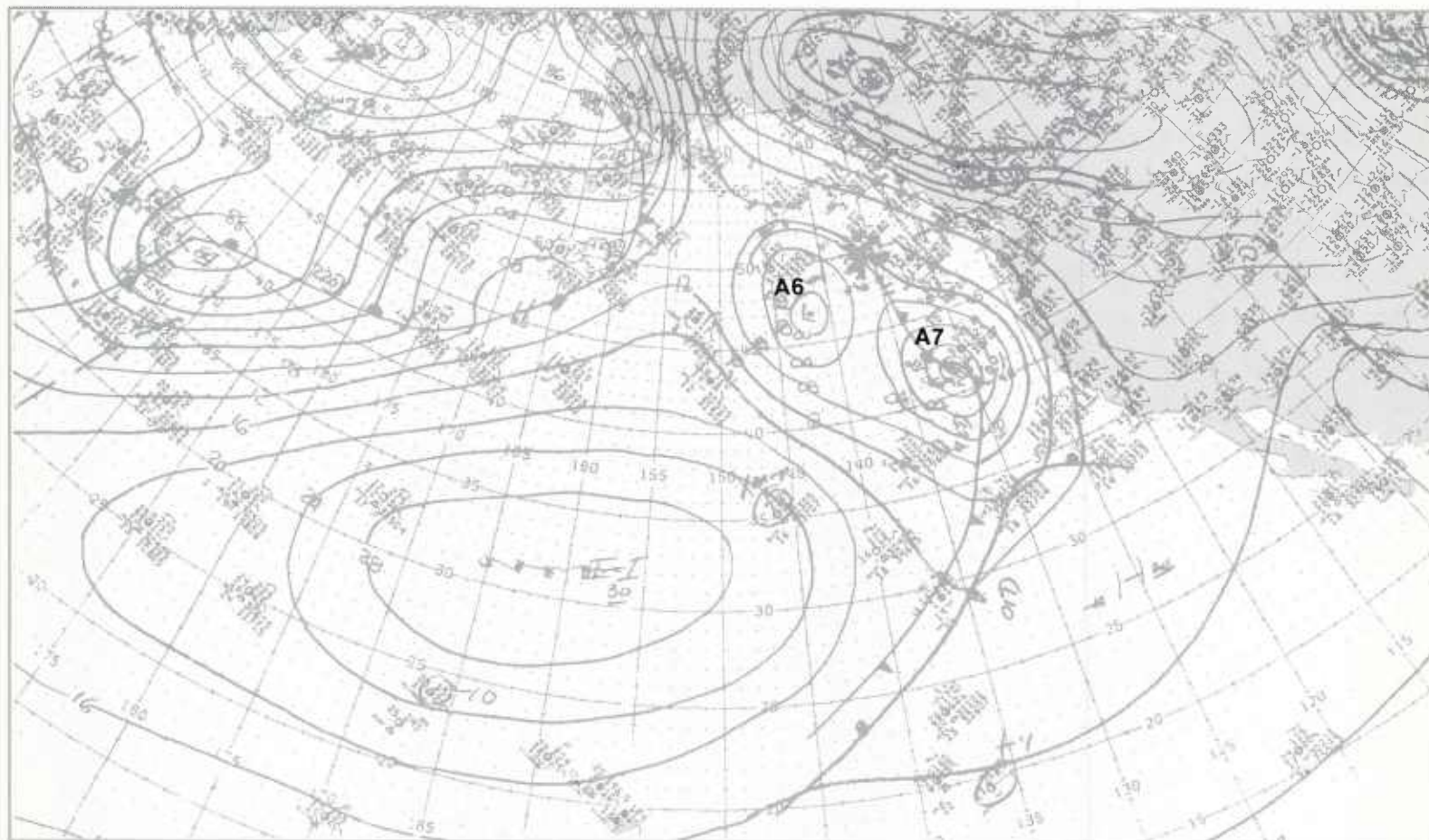
2B-19b. NMC Surface Analysis. 0000 GMT 14 January 1979.
