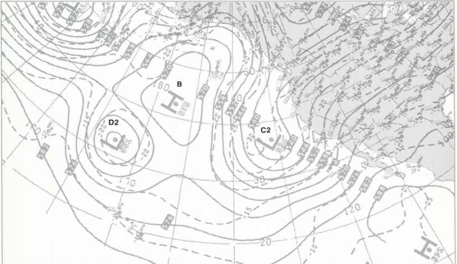
1B-86b. NMC 500-mb Analysis. 0000 GMT 27 March 1979.
