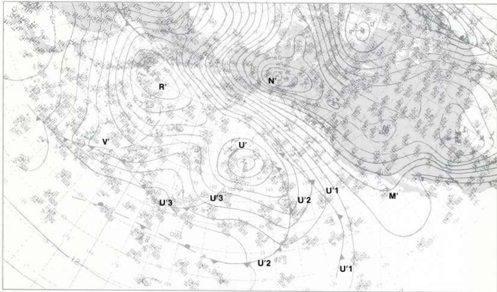
1B-35b. NMC Surface Analysis. 0000 GMT 3 January 1979.
