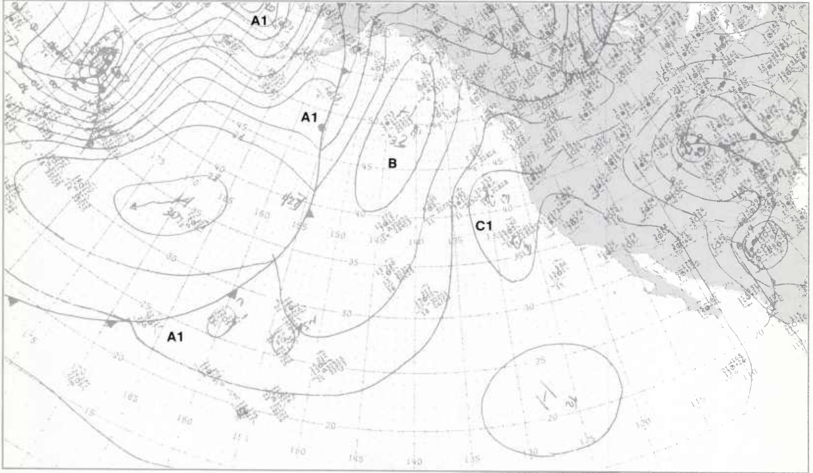
1B-77b. NMC Surface Analysis. 1200 GMT 22 March 1979.
