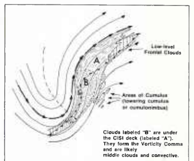
2A-16e. Meridional Trough Cyclogenesis, Phase 2.
