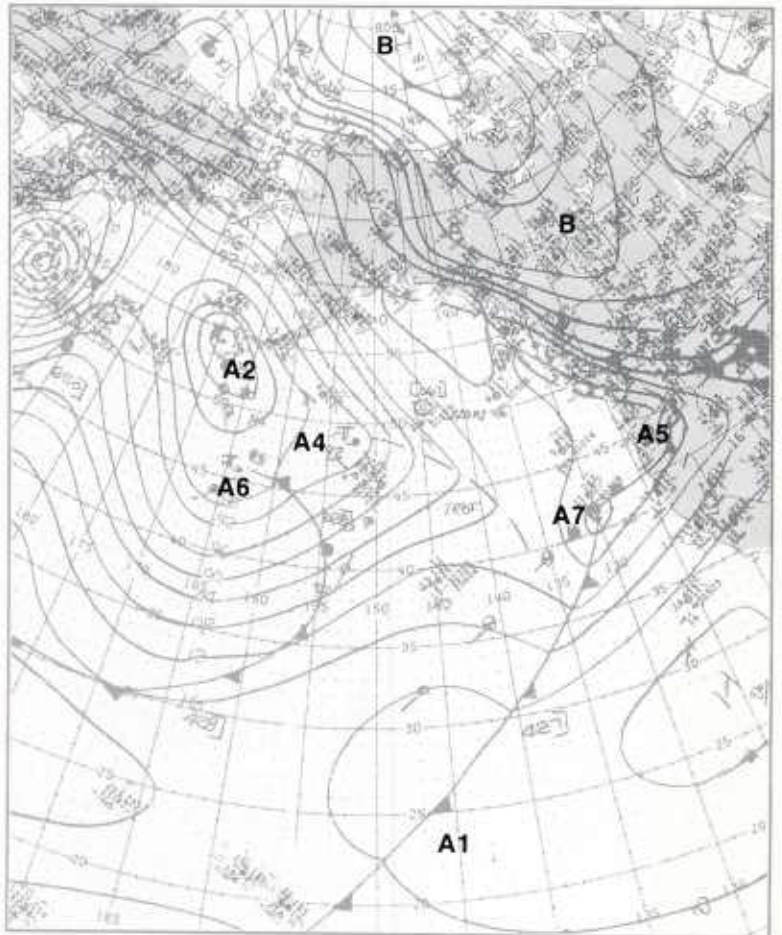
2B-9c. NMC Surface Analysis. 1200 GMT 11 January 1979.
