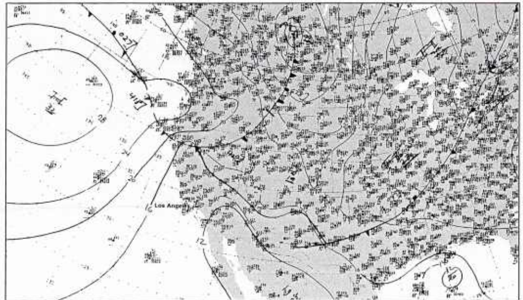
3B-10b. NMC Surface Analysis. 1800 GMT 29 August 1977.
