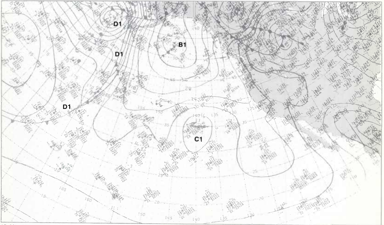
IB-83b. NMC Surface Analysis. 0000 GMT 25 March 1979.
