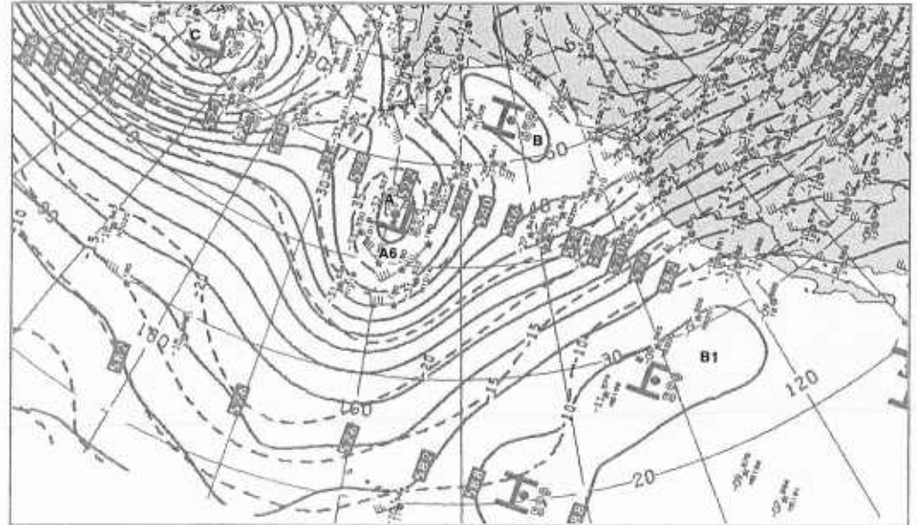
2B-10b. NMC 500-mb Analysis. 0000 GMT 12 January 1979.
