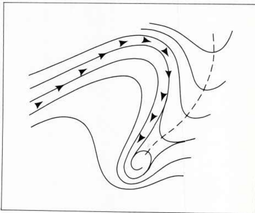
1B-73a. Formation of a cutoff low (Weldon, 1983).
