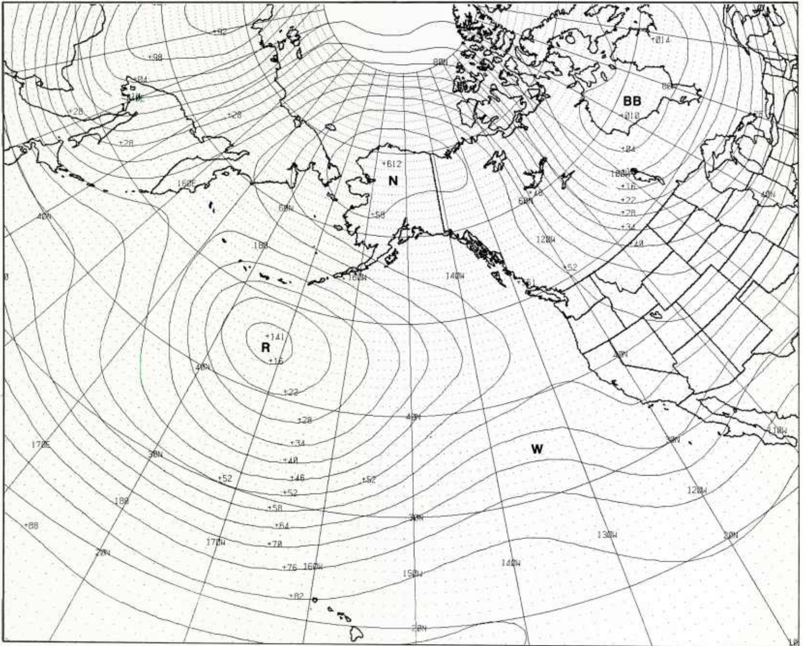
1B-45a. FNOc PE 72-hr 500-mb Prognosis. Valid 0000 GMT 9 January 1979.
