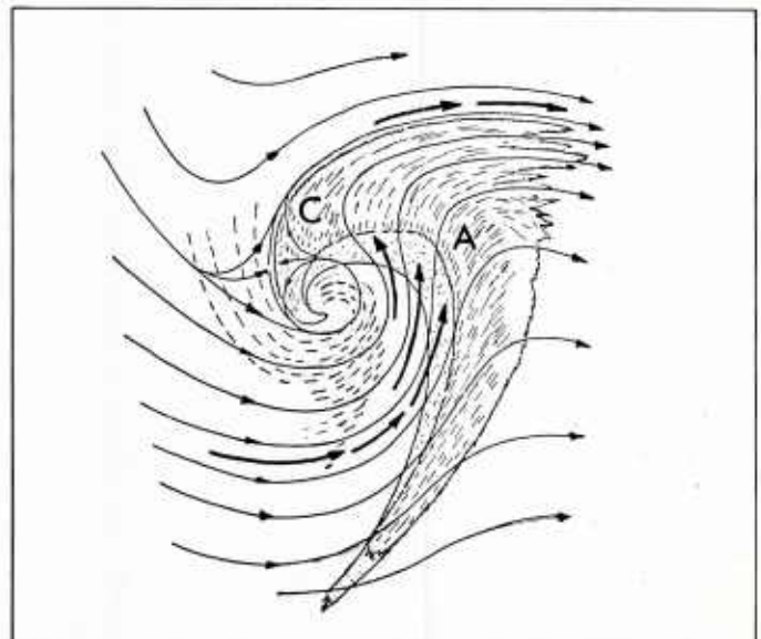
2A-9d. Split Flow Cyclogenesis, Phase 4.
