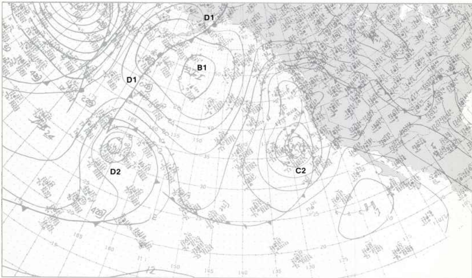
1B-87b. NMC Surface Analysis. 0000 GMT 27 March 1979.
