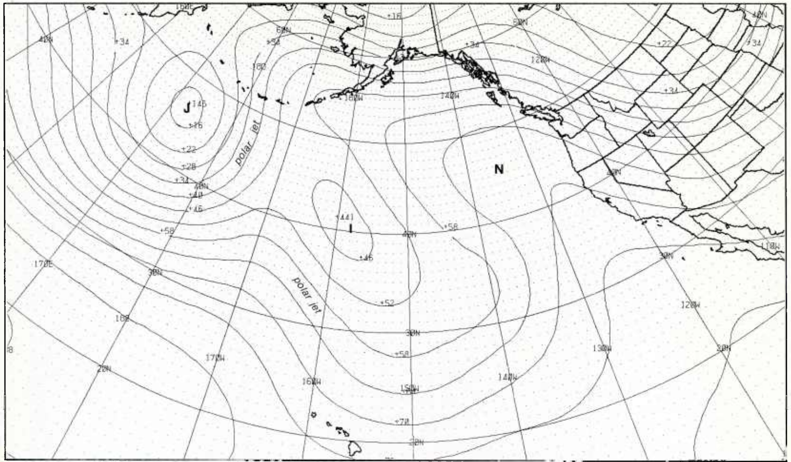
1B-13a. FNOC PE 36-hr 500-mb Prognosis. Valid 1200 GMT 26 December 1978.
