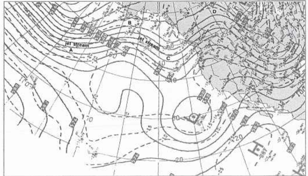
1B-62b. NMC 500-mb Analysis. 0000 GMT 24 January 1979.
