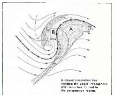
2A-16g. Meridional Trough Cyclogenesis, Phase 4.
