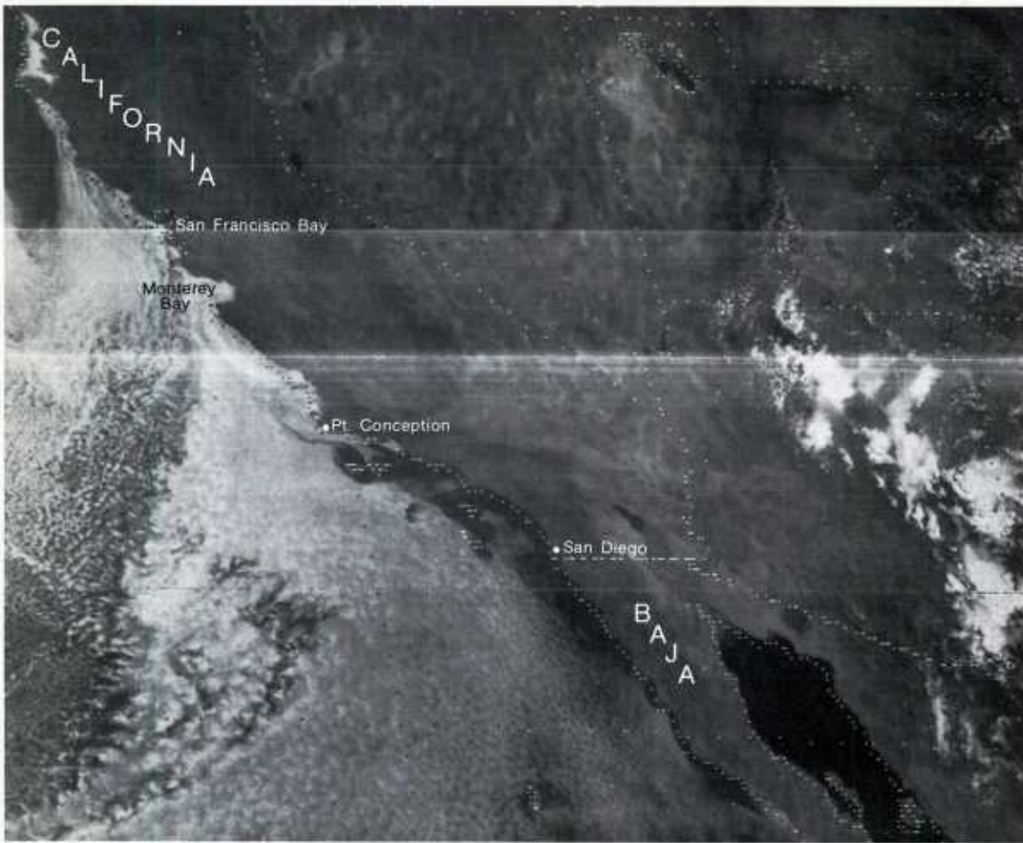
3B-3a. GOES-W. Visible Picture. 1945 GMT 12 July 1977.
