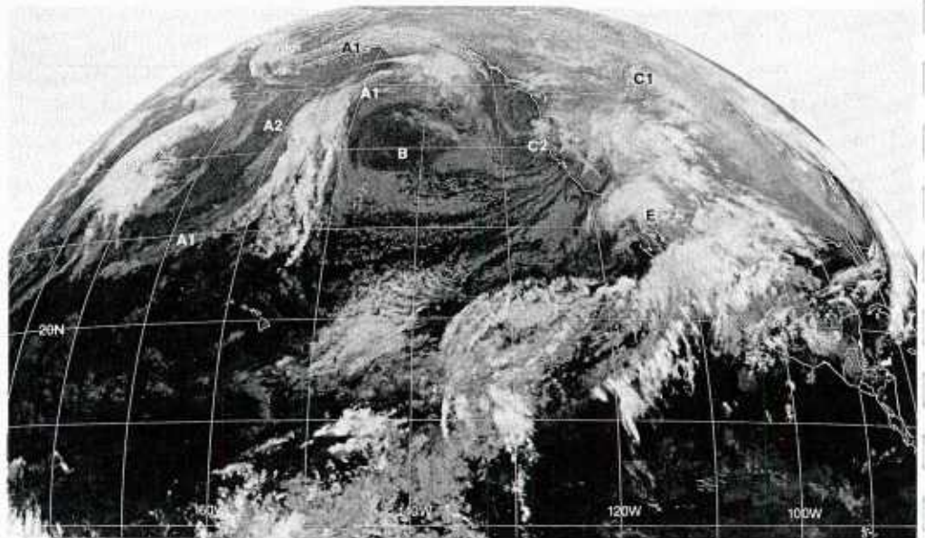
1B-68a. GOES-W. Infrared Picture. 0015 GMT 25 January 1979.
