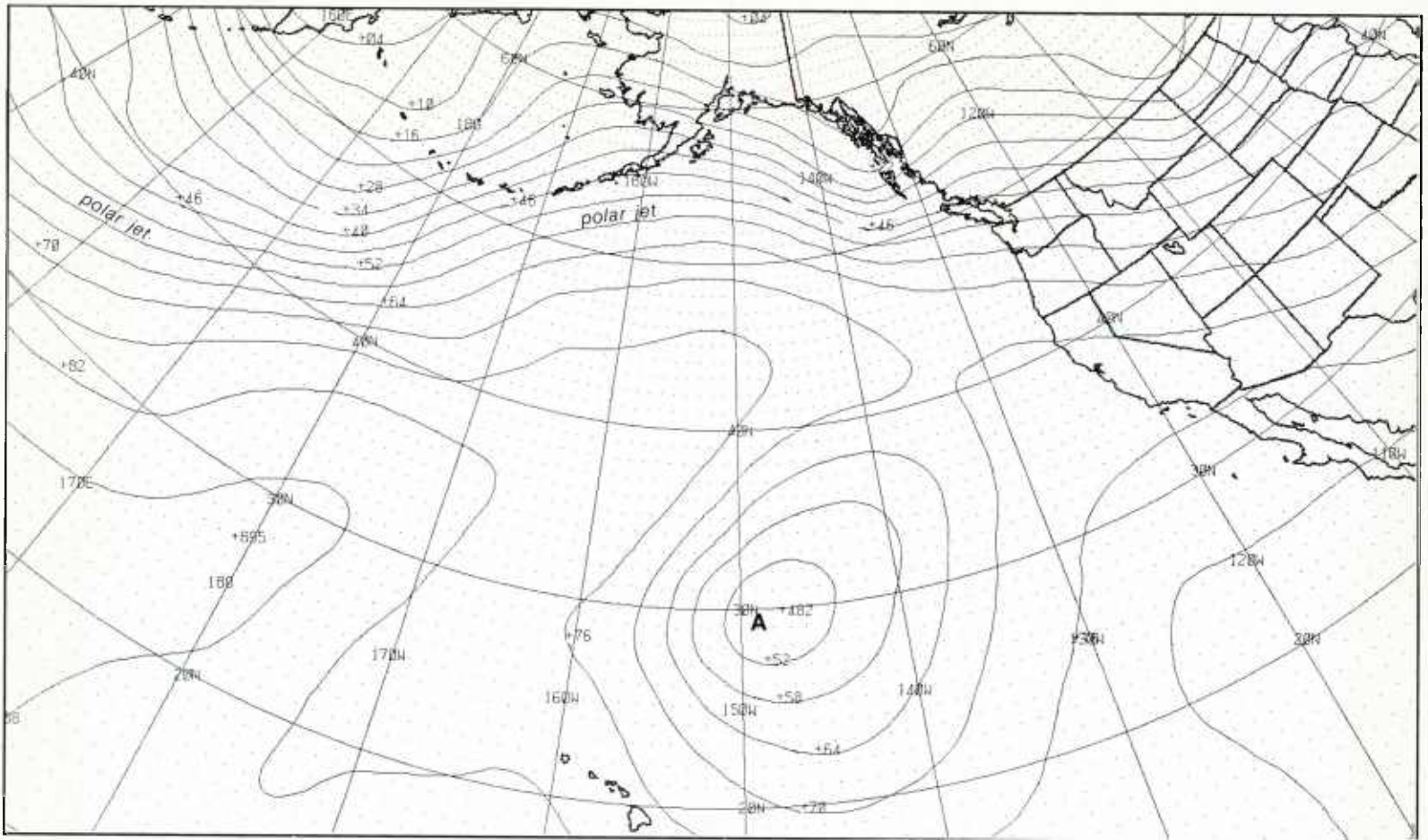
1B-4a. FNOC PE Initial 500-mb Analysis. 0000 GMT 22 December 1978.
