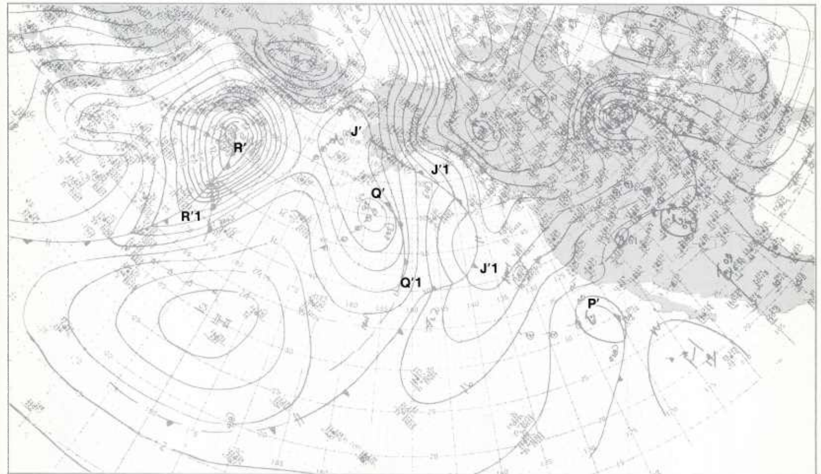
1B-23b. NMC Surface Analysis. 1200 GMT 29 December 1978.
