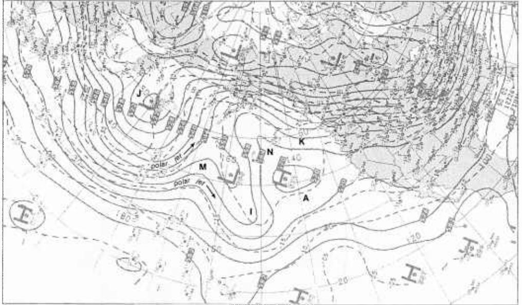
1B-14b. NMC 500-mb Analysis. 1200 GMT 26 December 1978.
