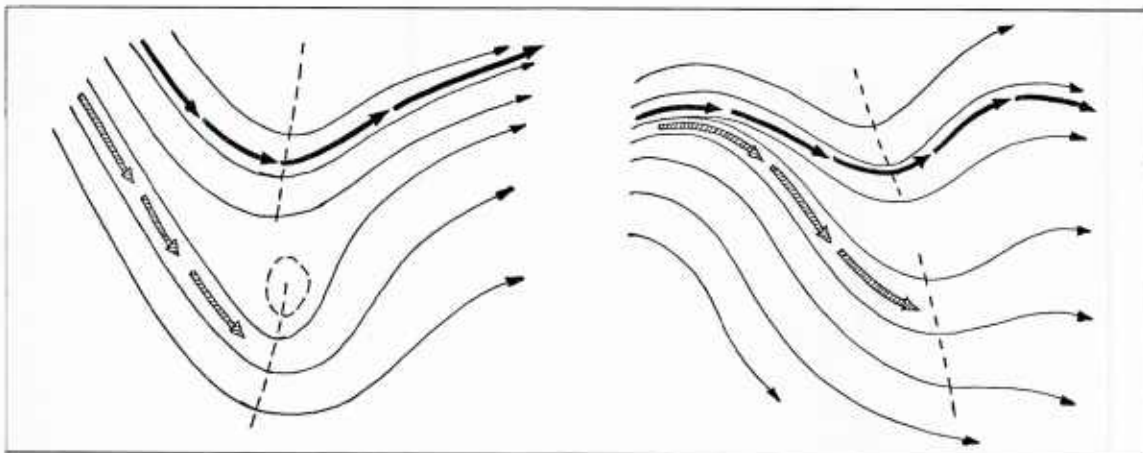
2A-5b. Typical flow patterns for Split Flow Cyclogenesis.
