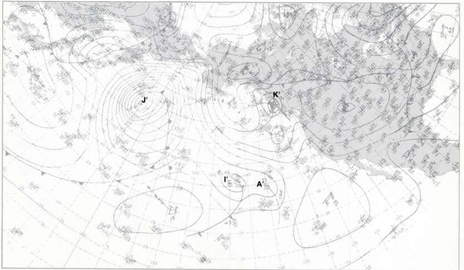
1B-15b. NMC Surface Analysis. 1200 GMT 26 December 1978.
