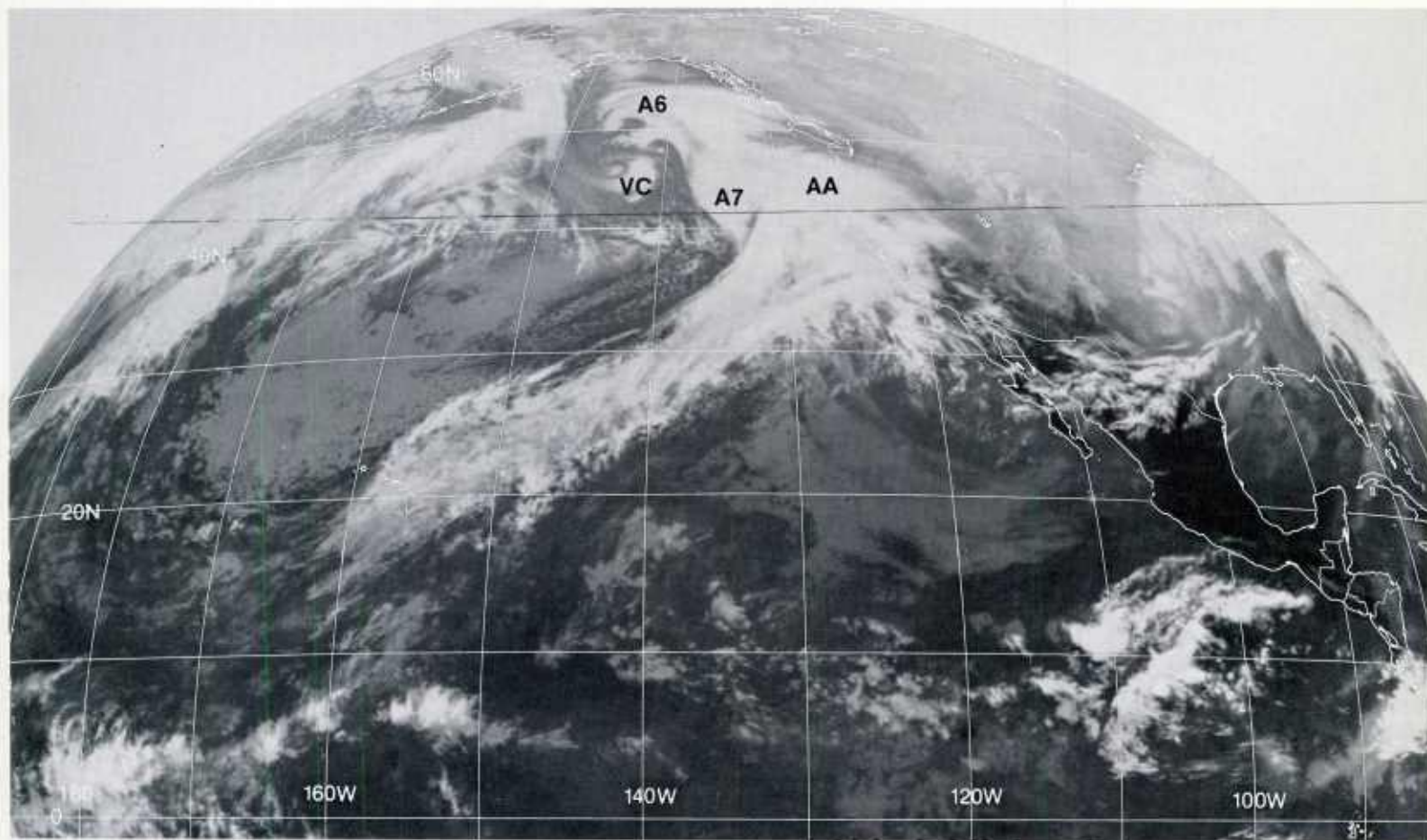
2B-17a. GOES-W. Infrared Picture. 2015 GMT 13 January 1979.
