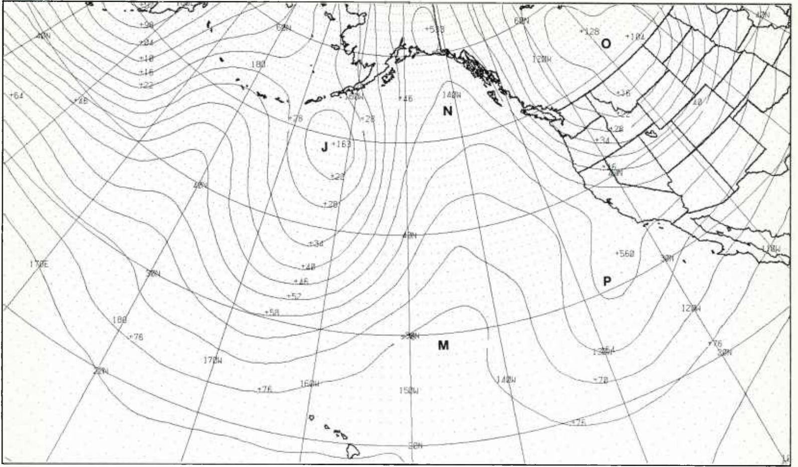
1B-24a. FNOC PE Initial 500-mb Analysis. 1200 GMT 29 December 1978.
