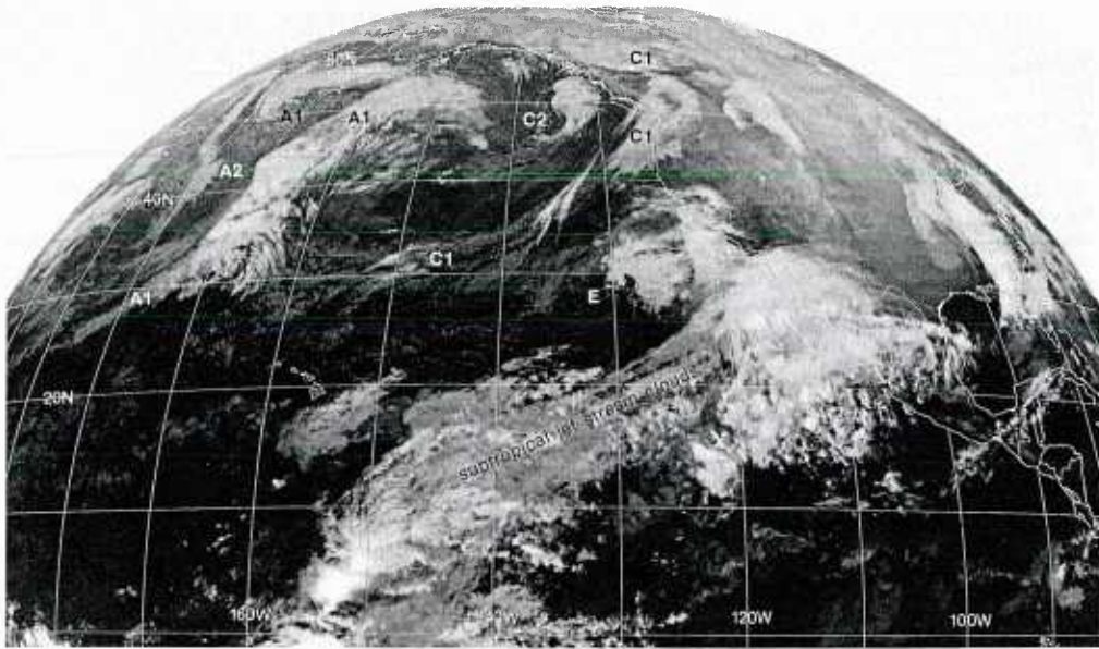
1B-63a. GOES-W. Infrared Picture. 0015 GMT 24 January 1979.
