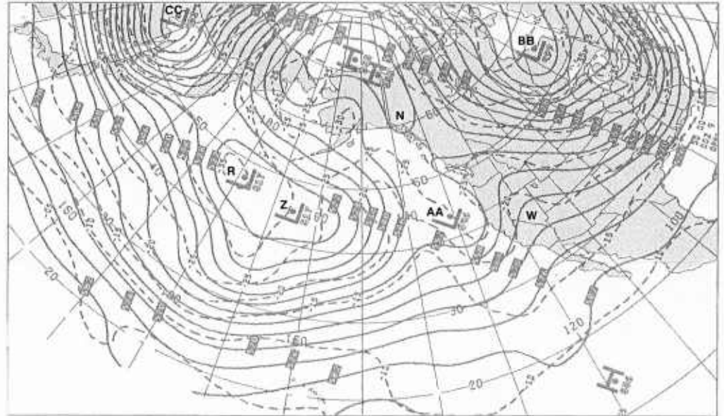
1B-50b. NMC 500-mb Analysis. 0000 GMT 9 January 1979.
