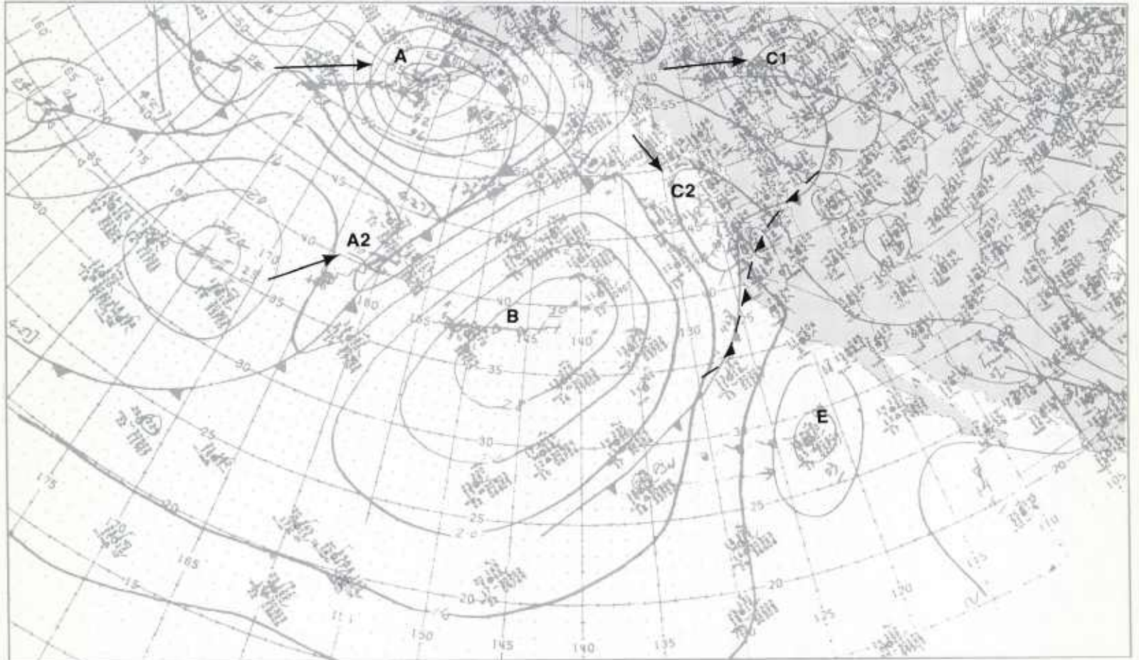
1B-66b. NMC Surface Analysis. 1800 GMT 24 January 1979.
