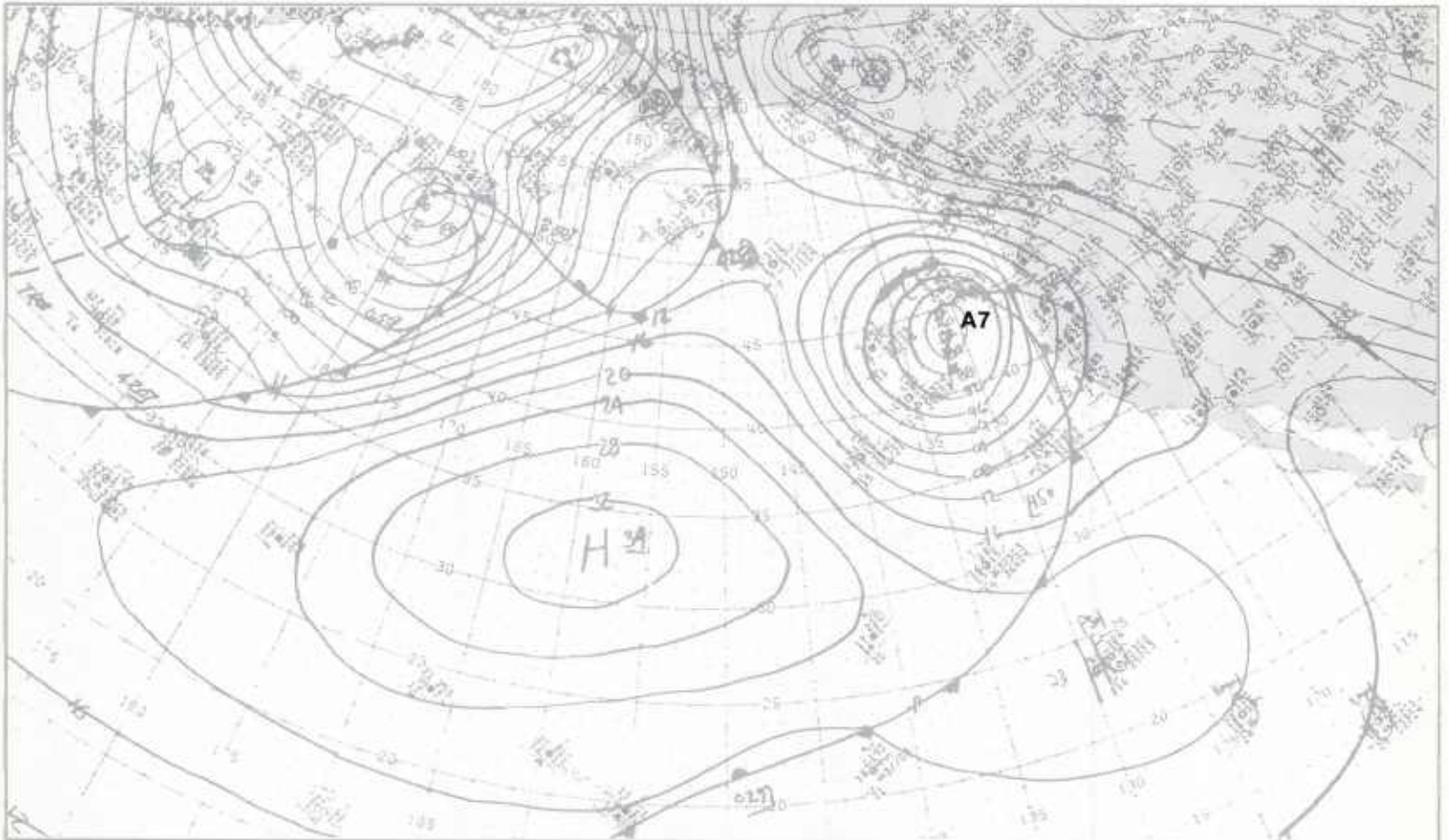
2B-21b. NMC Surface Analysis. 1200 GMT 14 January 1979.
