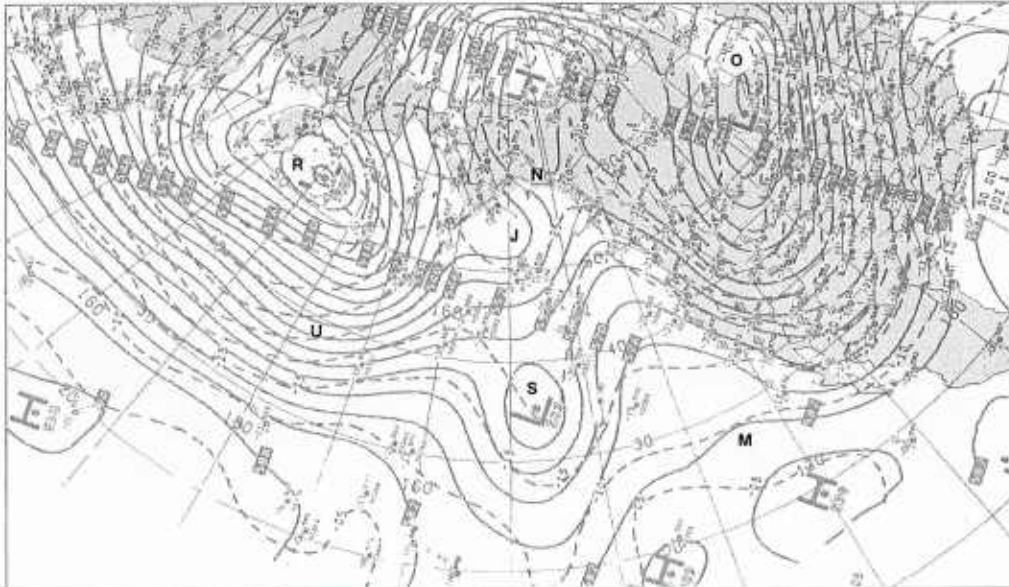
1B-31b. NMC 500-mb Analysis. 0000 GMT 1 January 1979.
