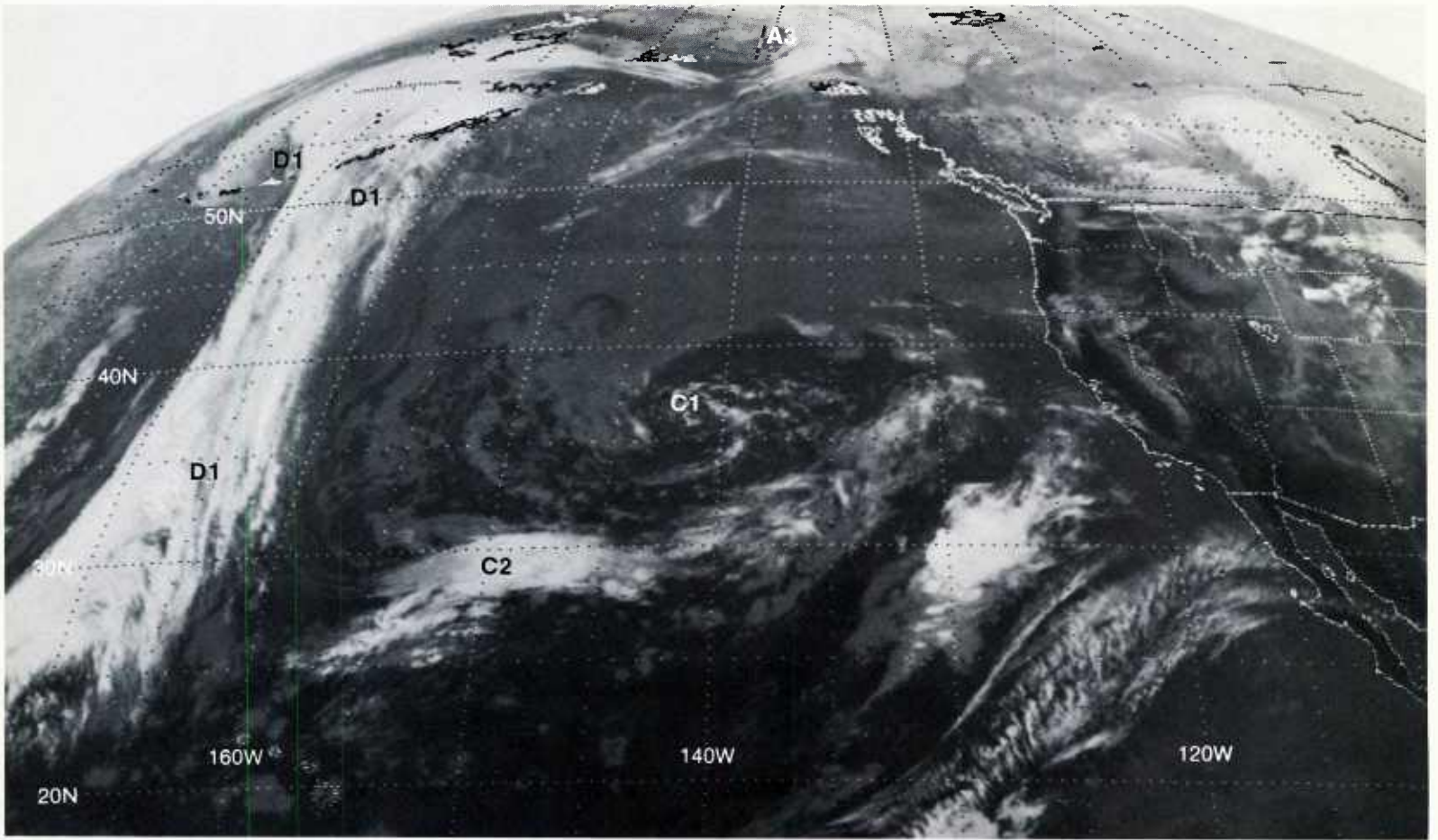
IB-83a. GOES-W. Infrared Picture. 0045 GMT 25 March 1979.
