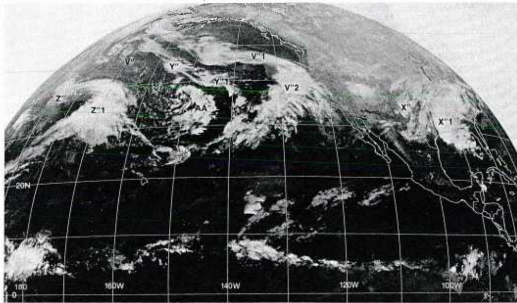
1B-47a. GOES-W. Infrared Picture. 0015 GMT 7 January 1979.
