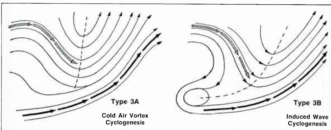
2A-5c. Typical flow patterns for Cold Air Vortex/ Induced Wave Cyclogenesis.
