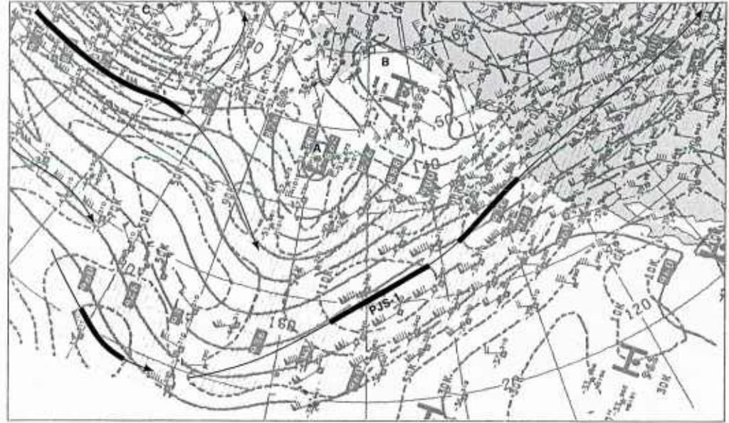
2B-10a. NMC 300-mb Analysis. 0000 GMT 12 January 1979.
