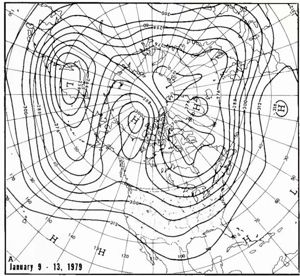
1B-53b. Mean 700-mb Contours for 9-13 January 1979. (After Wagner, 1979.)
