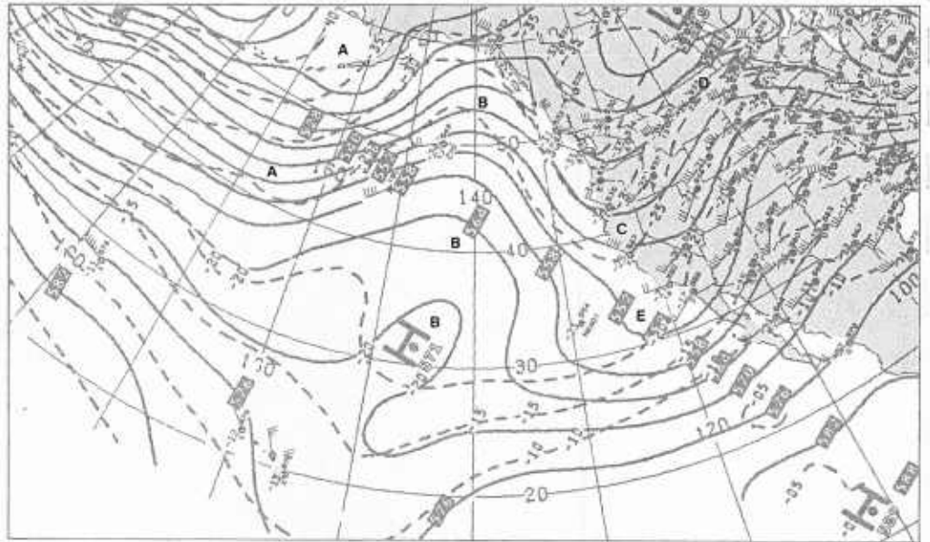
1B-68b. NMC 500-mb Analysis. 0000 GMT 25 January 1979.
