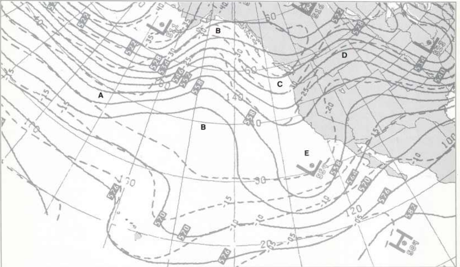
1B-64b. NMC 500-mb Analysis. 1200 GMT 24 January 1979.
