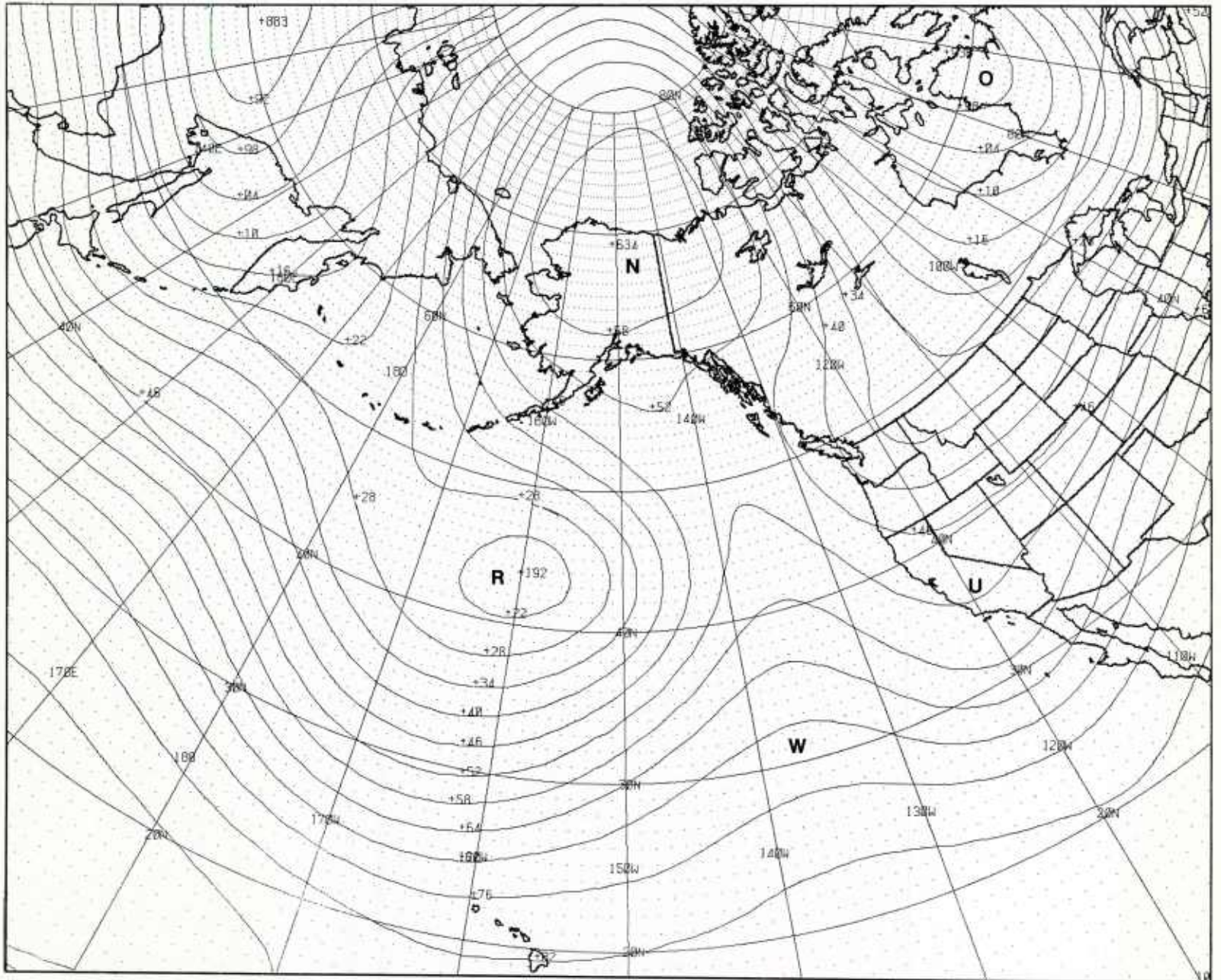
1B-37a. FNOC PE 72-hr 500-mb Prognosis. Valid 0000 GMT 6 January 1979.
