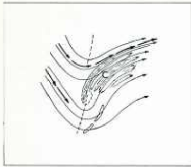
2A-17a. Split Flow Cyclogenesis, Phase 1.
