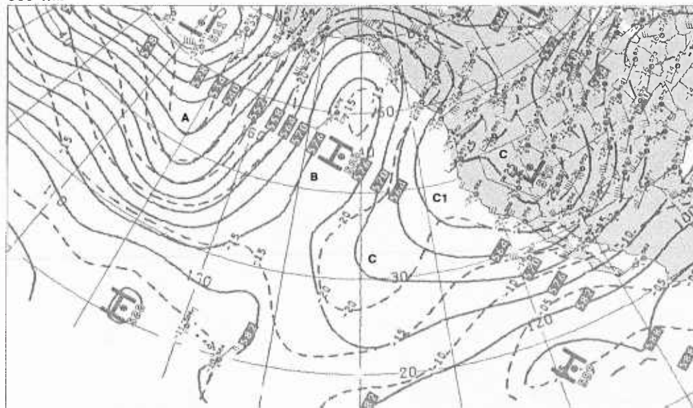
IB-74b. NMC 500-mb Analysis. 0000 GMT 22 March 1979.
