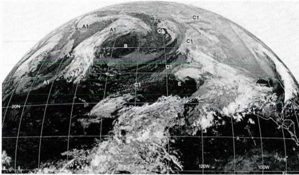
IB-65a. GOES-W. Infrared Picture, 1215 GMT 24 January 1979.
