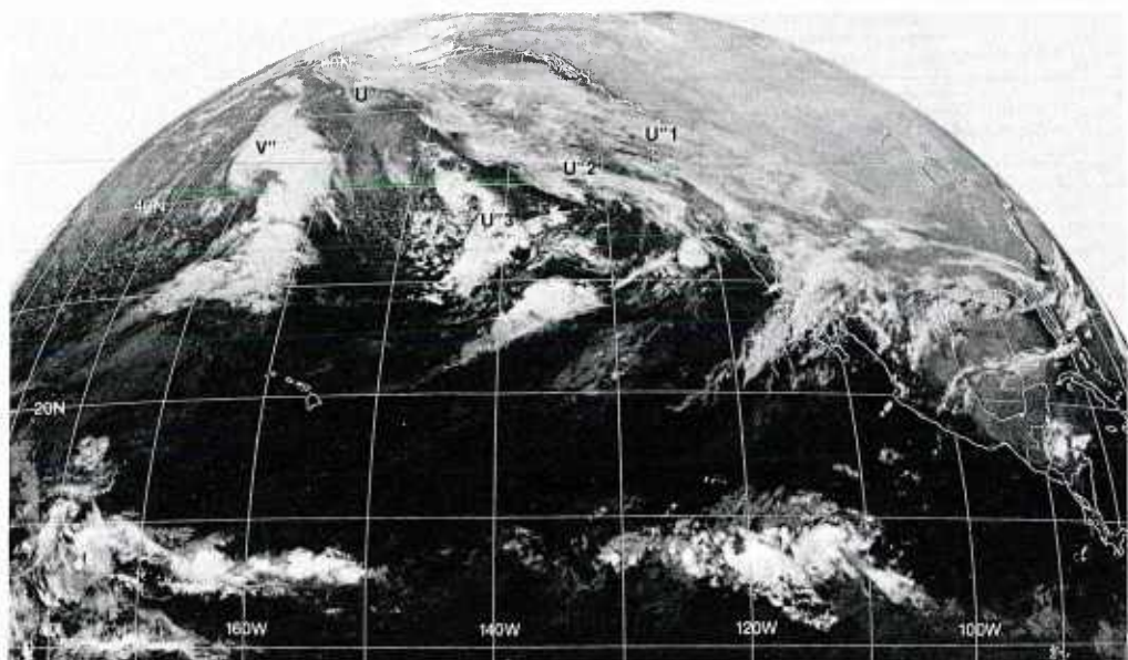
IB-39a. GOES-W. Infrared Picture. 0015 GMT 4 January 1979.
