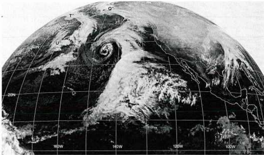
1B-31a. GOES-W. Infrared Picture. 0015 GMT 1 January 1979.
