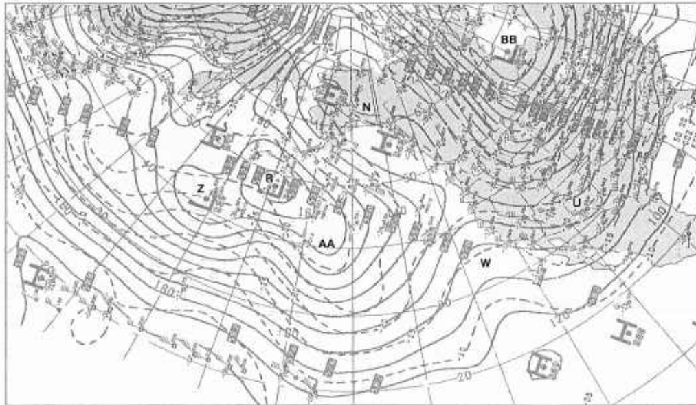
1B-47b. NMC 500-mb Analysis. 0000 GMT 7 January 1979.
