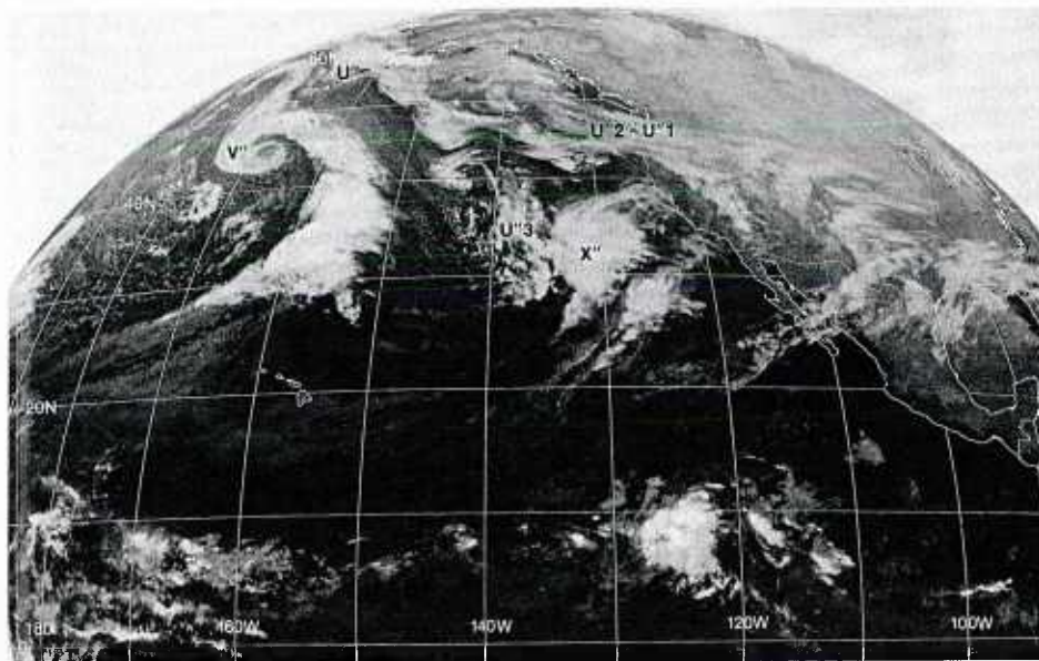
IB-39c. GOES-W. Infrared Picture. 1215 GMT 4 January 1979.
