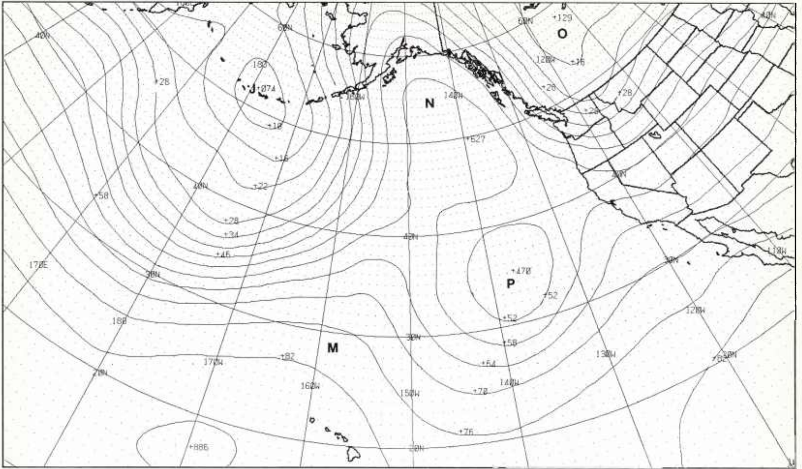
1B-20a. FNOC PE Initial 500-mb Analysis. 0000 GMT 28 December 1978.
