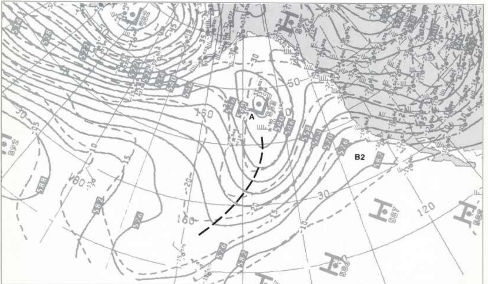
2B-14b. NMC 500-mb Analysis. 1200 GMT 13 January 1979.
