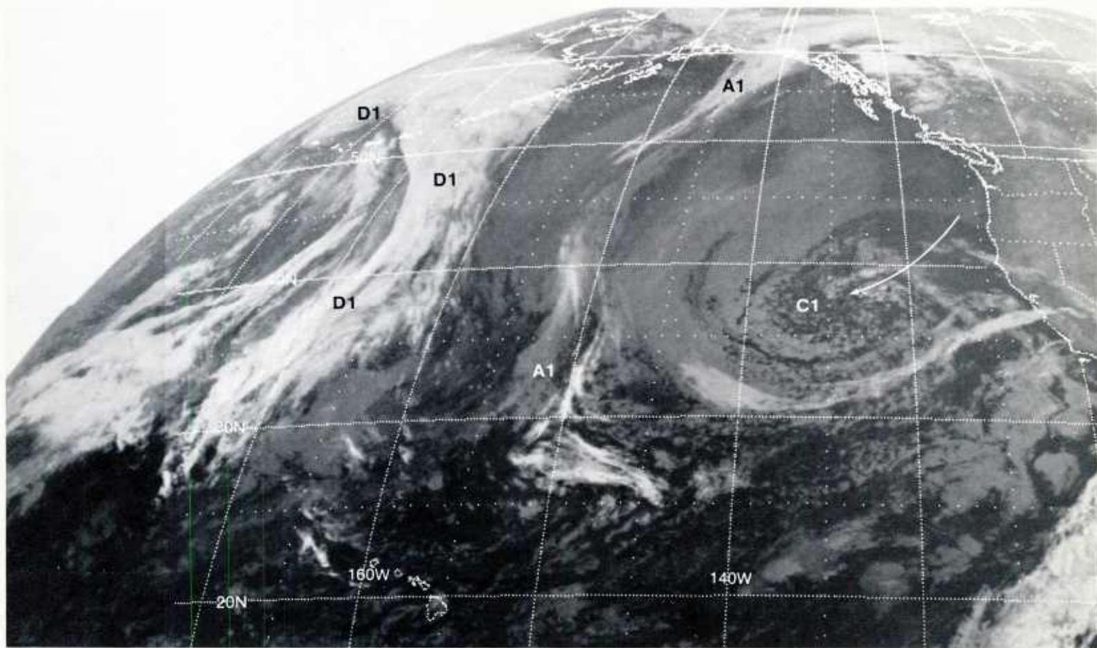
IB-81a. GOES-W. Infrared Picture. 1215 GMT 23 March 1979.
