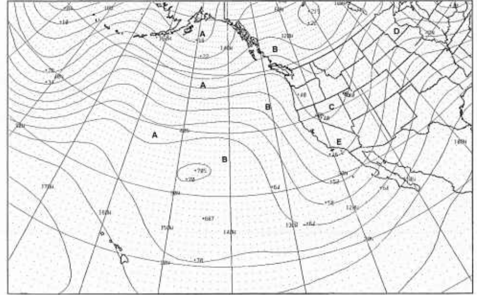
IB-65d. FNOC PE 36-hr 500-mb Prognosis, Valid 0000 GMT 26 January 1979.
