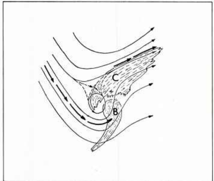
2A-9b. Split Flow Cyclogenesis, Phase 2.
