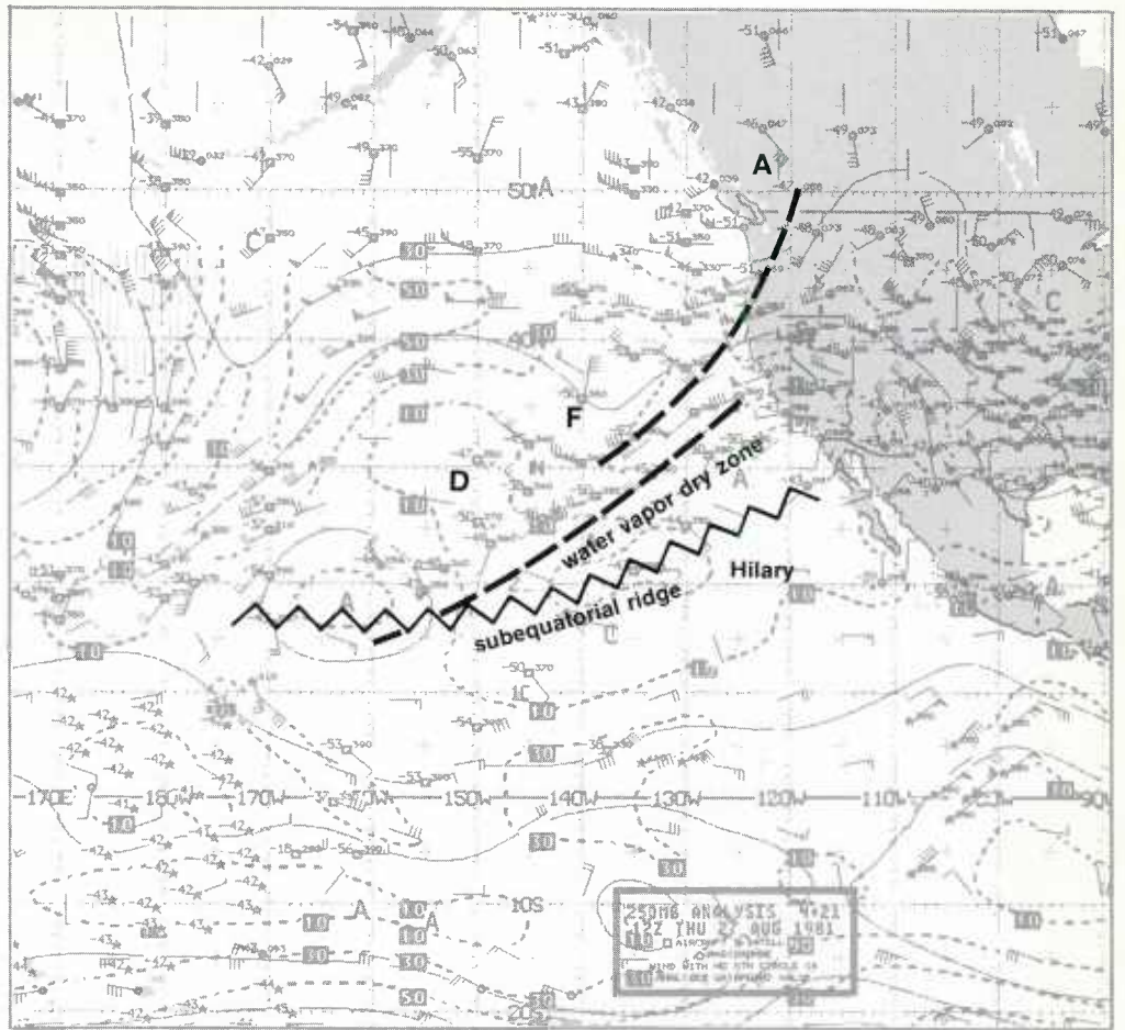
2B-32a. NMC Tropical Mercator 250-mb Analysis. 1200 GMT 27 August 1981.
