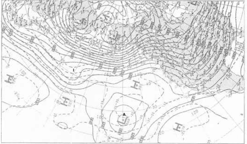
1B-6b. NMC 500-mb Analysis. 1200 GMT 23 December 1978.
