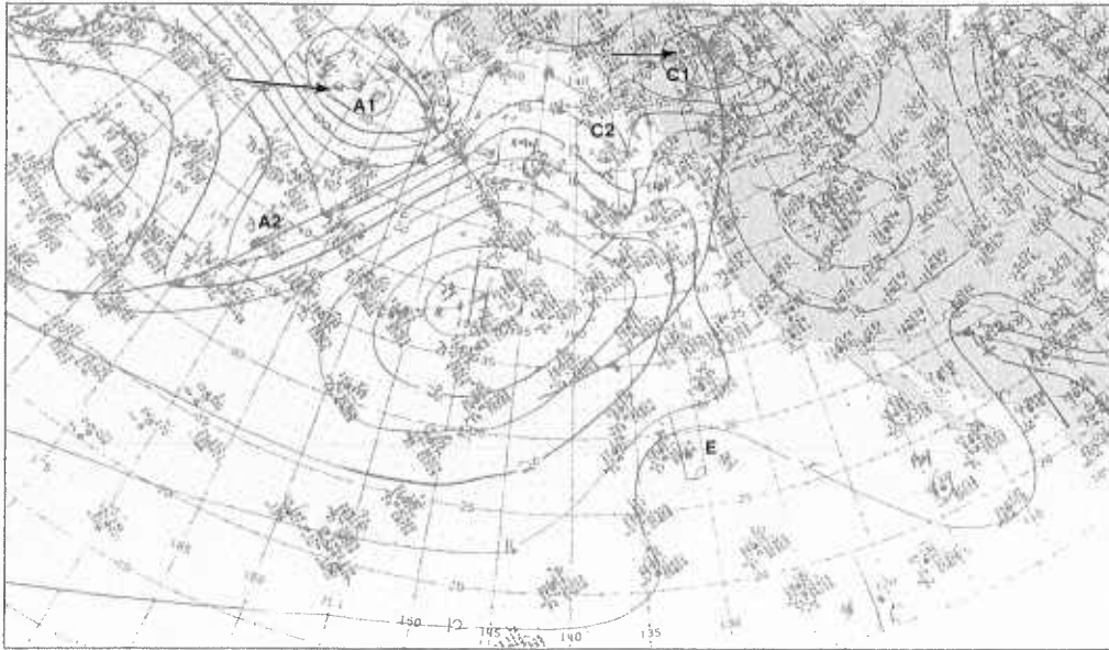
1B-63b. NMC Surface Analysis. 0000 GMT 24 January 1979.
