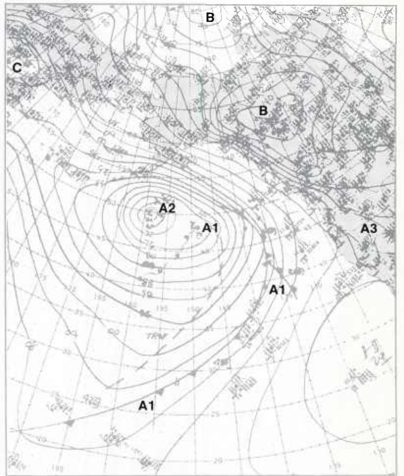
2B-4c. NMC Surface Analysis. 1200 GMT 9 January 1979.
