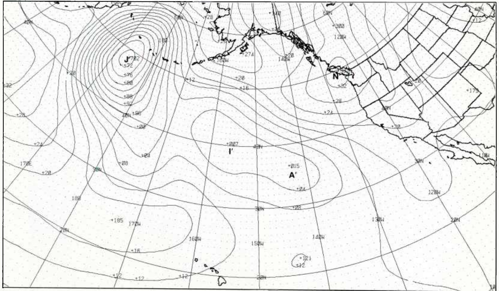
1B-13b. FNOC PE 36-hr Surface Prognosis. Valid 1200 GMT 26 December 1978.
