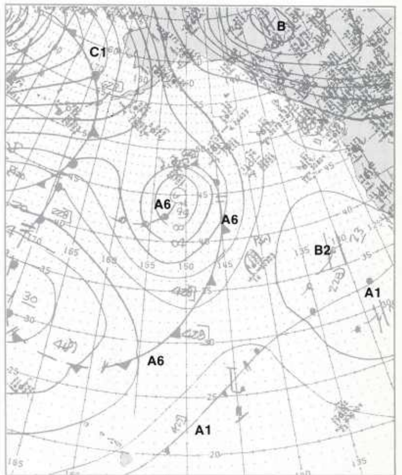
2B-12c. NMC Surface Analysis. 1200 GMT 12 January 1979.
