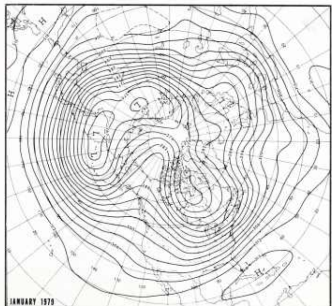
1B-1b. Mean 700-mb Contours for January 1979. (After Wagner, 1979.)
