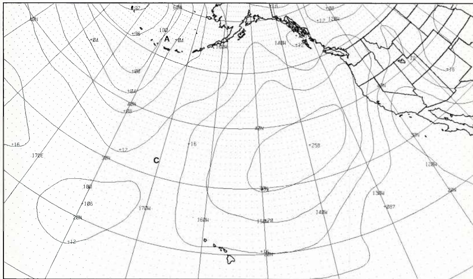
2B-33b. FNOC PE 24-hr Surface Prognosis. Valid 1200 GMT 28 August 1981.
