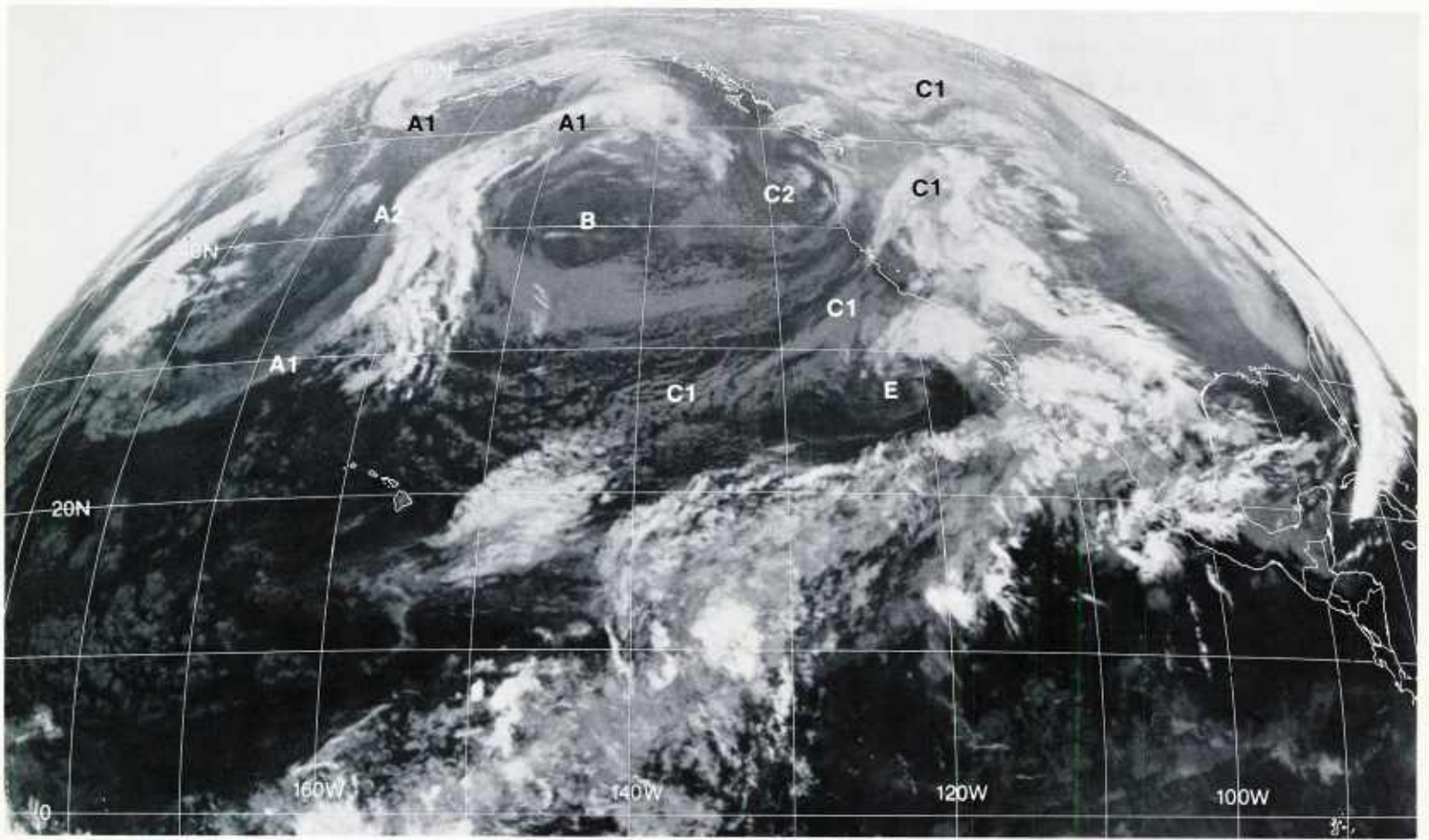
1B-66a. GOES-W. Infrared Picture. 1815 GMT 24 January 1979.
