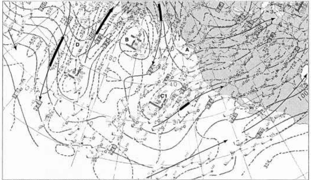
1B-84a. NMC 300-mb Analysis. 0000 GMT 26 March 1979.
