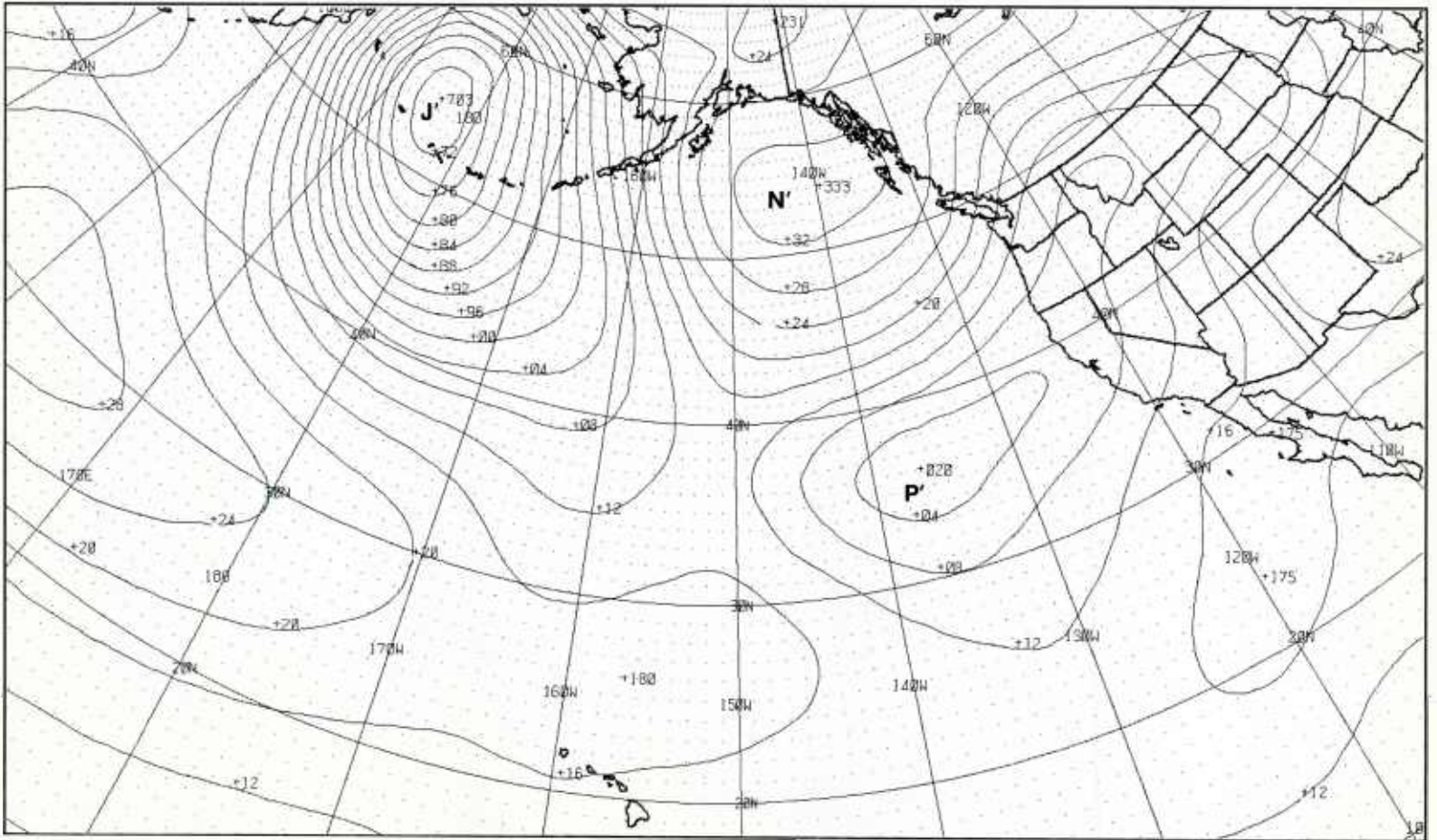
IB-17b. FNOC PE 36-hr Surface Prognosis. Valid 0000 GMT 28 December 1978.
