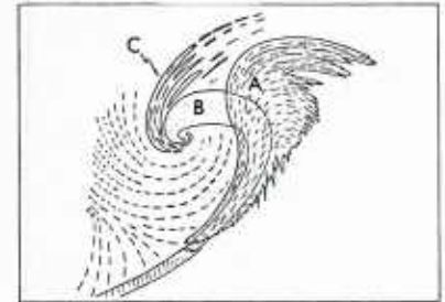
2A-3a. Type A Mature Storm Cloud Pattern.
