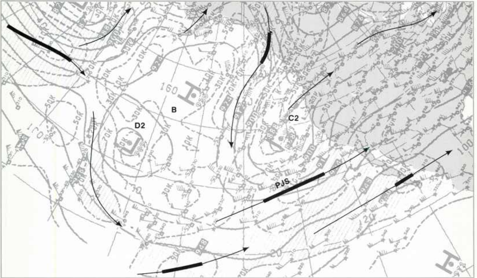
1B-86a. NMC 300-mb Analysis. 0000 GMT 27 March 1979.
