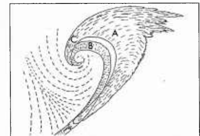
2A-3c. Type B Mature Storm Cloud Pattern.
