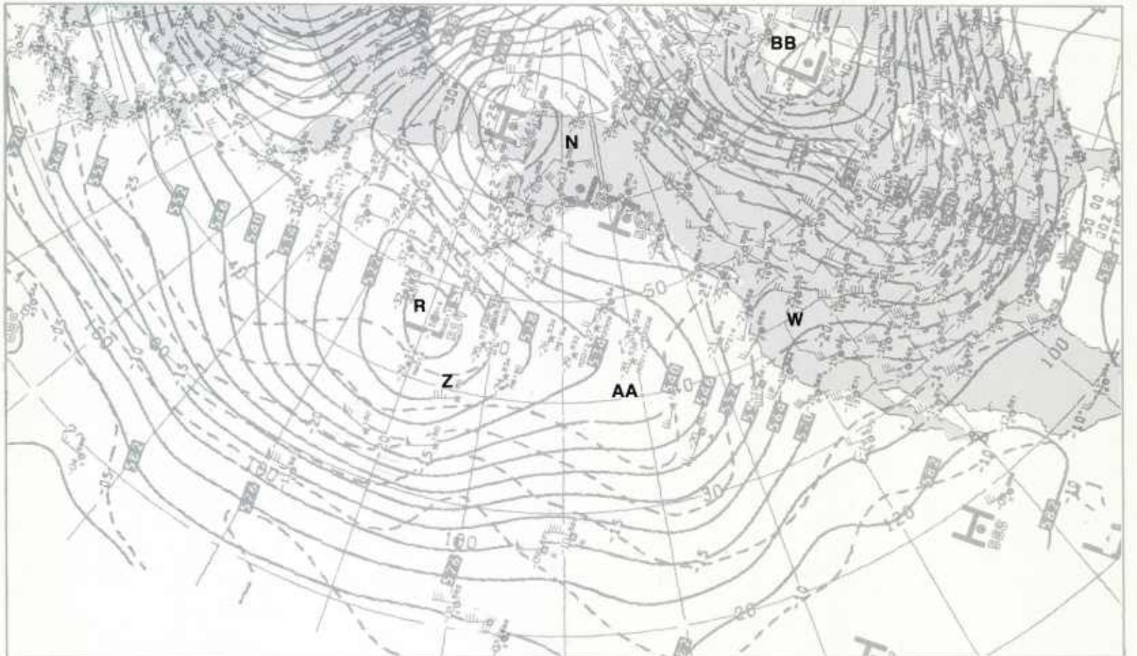
1B-48b. NMC 500-mb Analysis. 0000 GMT 8 January 1979.
