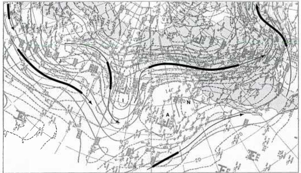
1B-10a. NMC 300-mb Analysis. 0000 GMT 25 December 1978.
