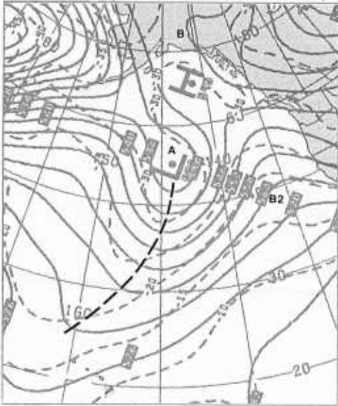
2B-13b. NMC 500-mb Analysis. 0000 GMT 13 January 1979.
