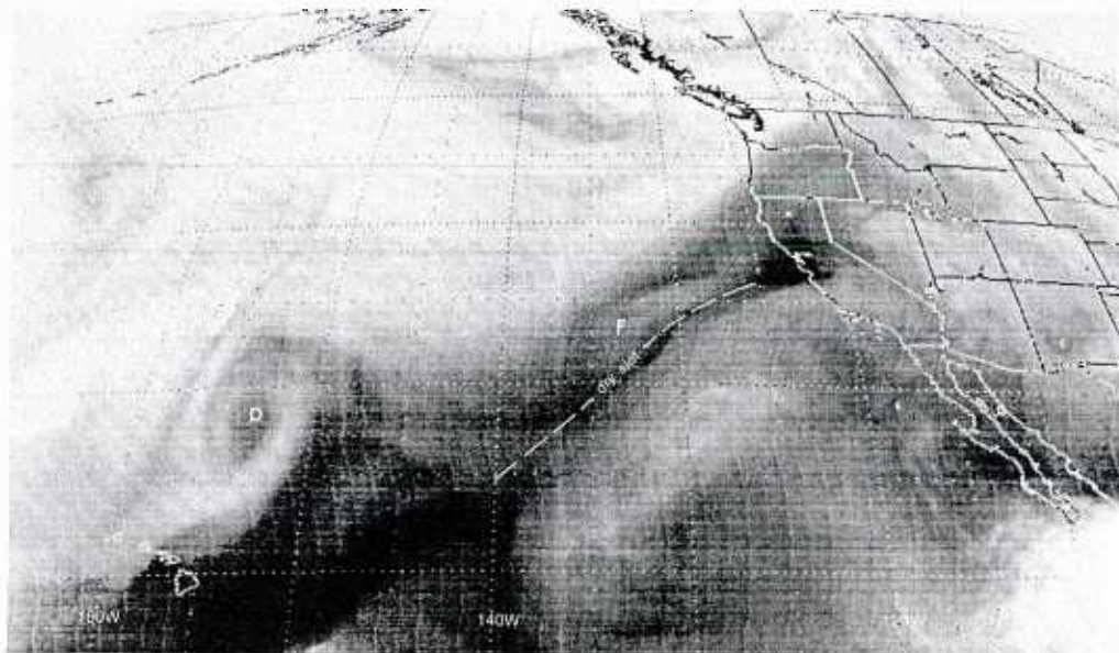
2B-35a. GOES-W. Water Vapor Picture. 1215 GMT 28 August 1981.
