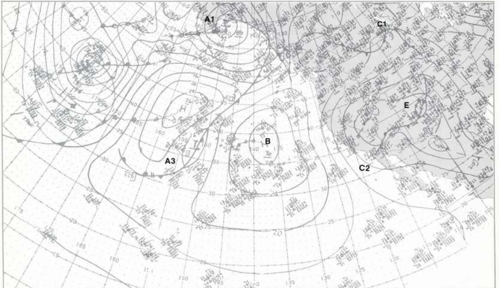
1B-70b. NMC Surface Analysis. 1800 GMT 25 January 1979.
