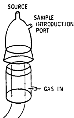
Figure 9. Design of Glass Atomization Chamber with Sample Introduction Port.
