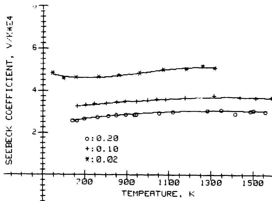
FIGURE 6.9. Seebeck Coefficient for Y_{1-x}Ca_xCrO_3
