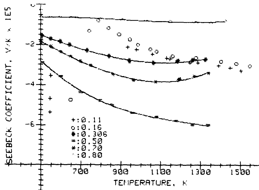
FIGURE 6.2. Seebeck Coefficient for (\text{In}_2\text{O}_3)_x \cdot (\text{SnO}_2)_{1-x}
