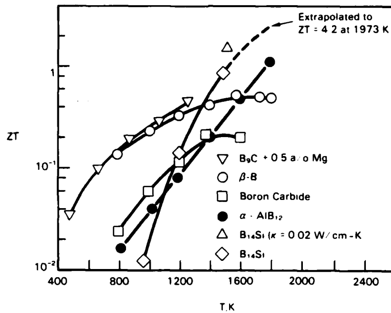
FIGURE 3.3. Values for Boron and Boron-Rich Borides (3.1)
