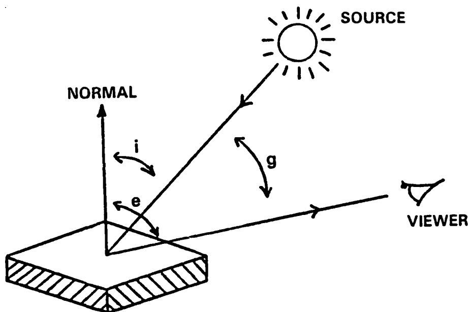
Figure 2.1-3 Image Formation Process
