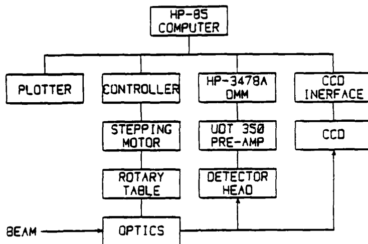
Figures 4. Computer control schematic.
