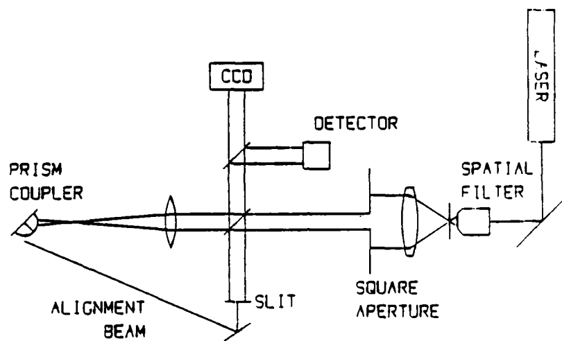
Figure 3. Optical system.
