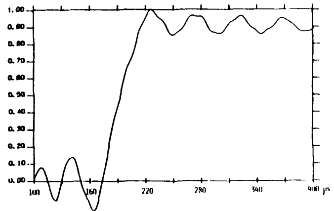
Fig. 4. Normalized u_y displacement at x=37.5 in.
