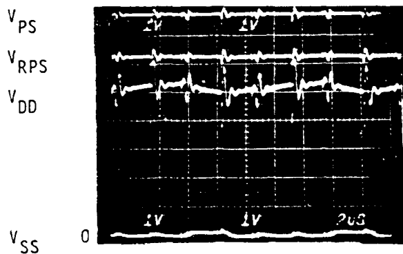
c) .01μF CAPACITOR ACROSS R_{SS1}
