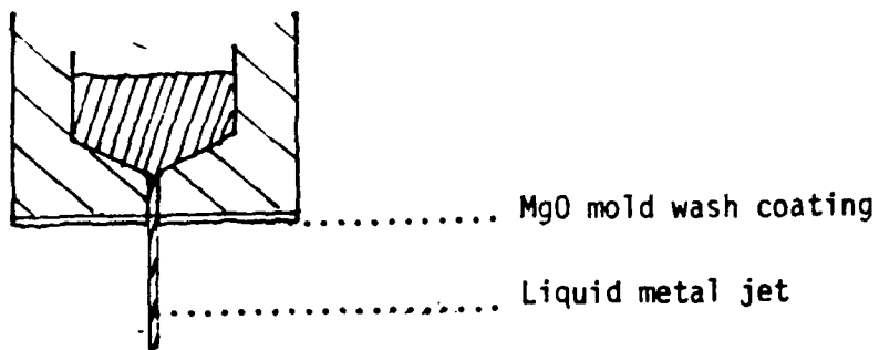
Figure 8-b , Coated crucible .
