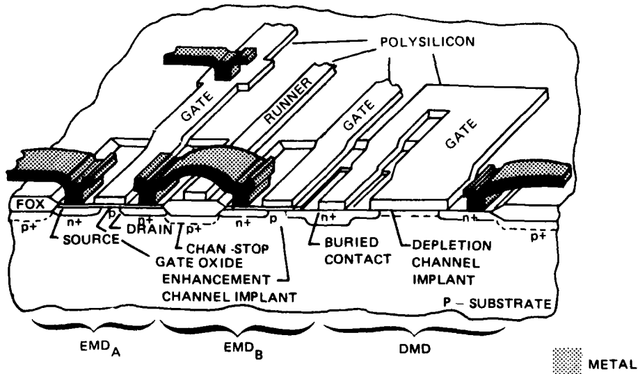
Figure 2. NMOS Structure
