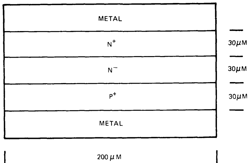
Figure 40. SOS Diode Topology
