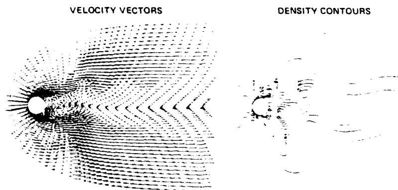
Fig. 13. Compressible flow around a circular cylinder at M = 0.8 and Re = 5 \cdot 10^6 (Ref. 31); 121 x 60 grid.
