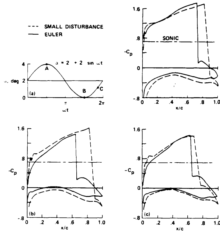
Fig. 3. Euler calculations of a transonic oscillating airfoil (Ref. 21); NACA 64A-410 airfoil, M = 0.72 , u_c/U_\infty = 0.20 .
