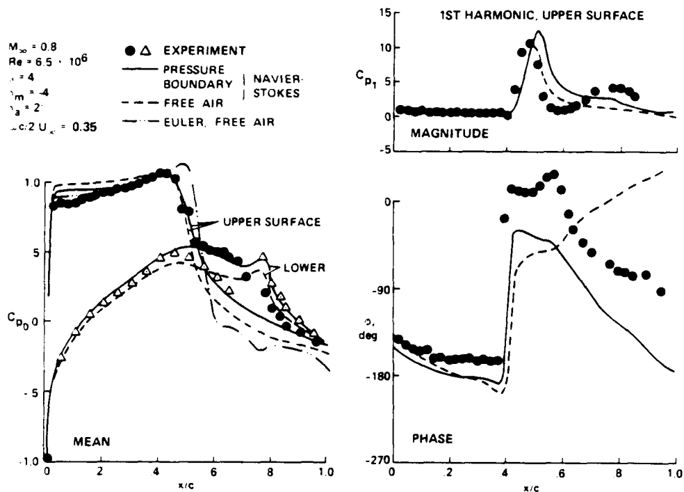
Fig. 12. Transonic viscous flow over an airfoil with an oscillating flap (Ref. 30); 139 x 49 grid.
